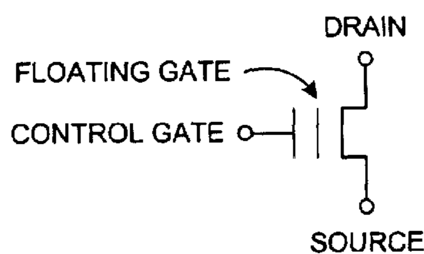
Figure 1B (PRIOR ART)
