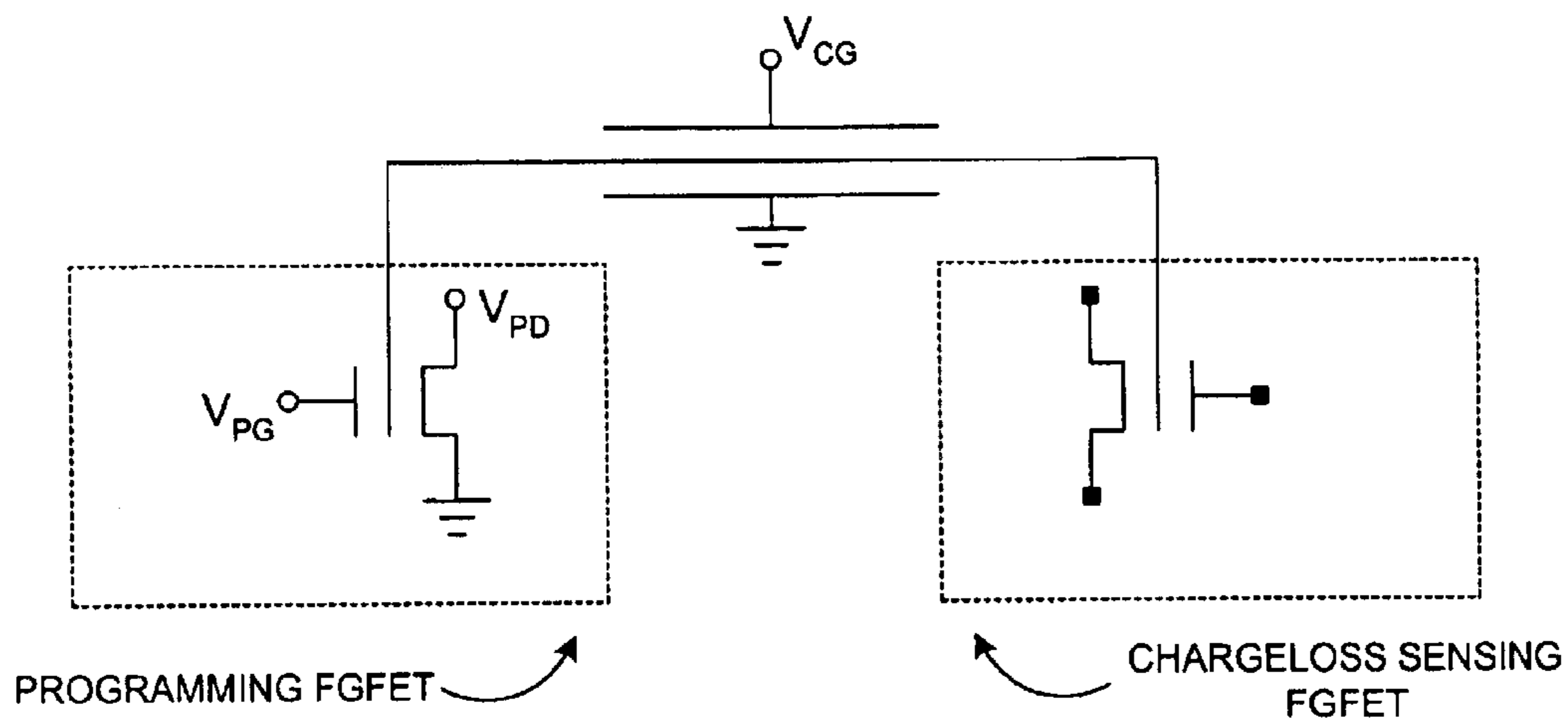
VOLTAGES DURING PROGRAMMING OPERATION
