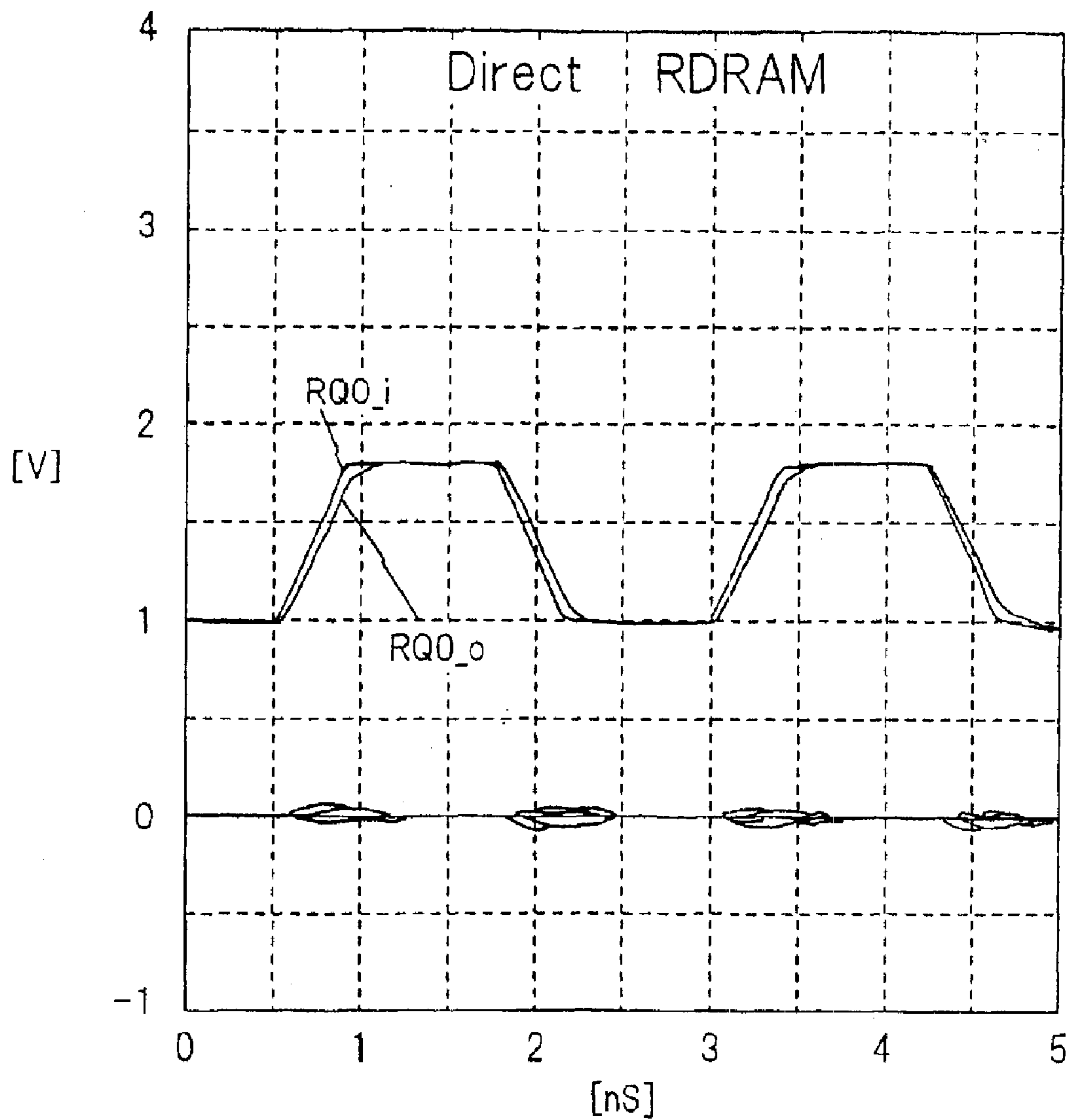
(c) CALCULATION OF CASE WITH ELECTROMAGNETIC SHIELDING FILM
