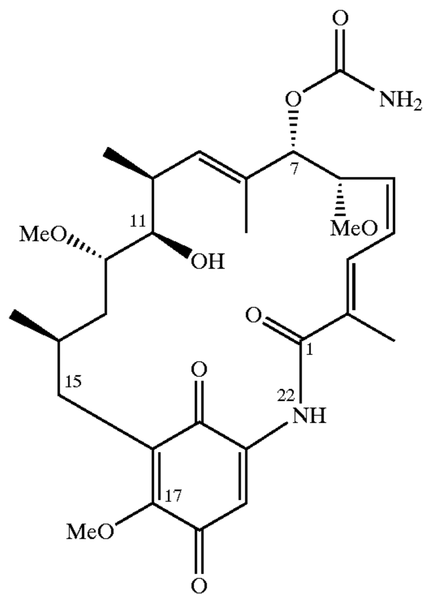
Geldanamycin
