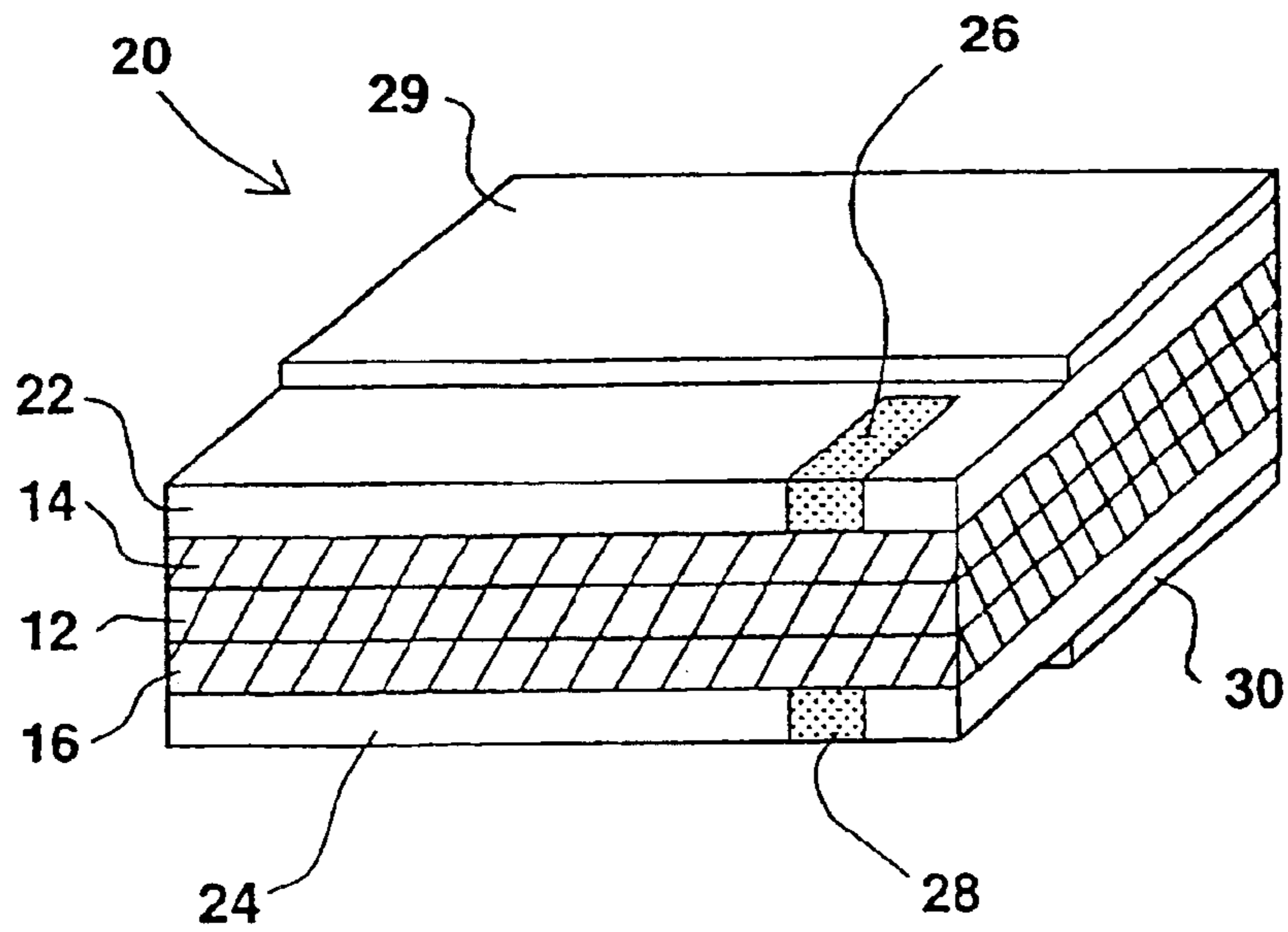
FIG. 2 (PRIOR ART)
