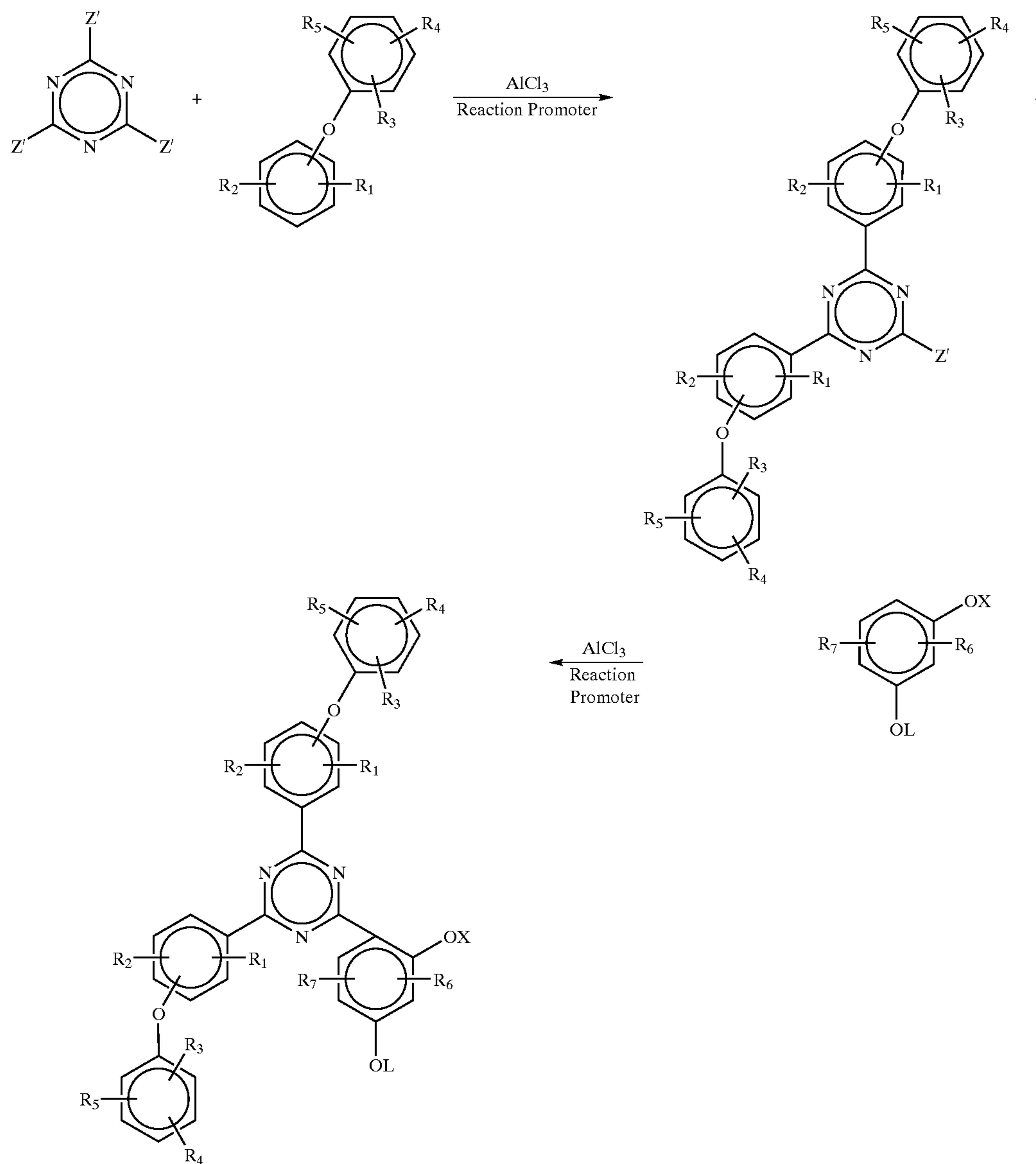
Scheme 1
