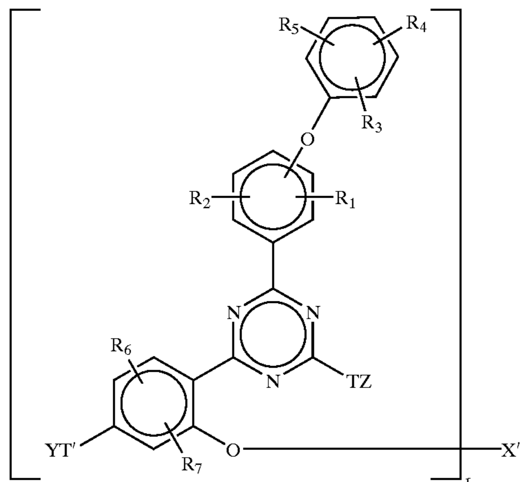
Formula VII
