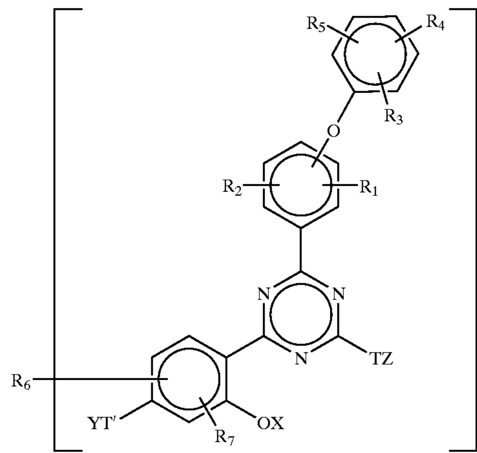
Formula VIII
