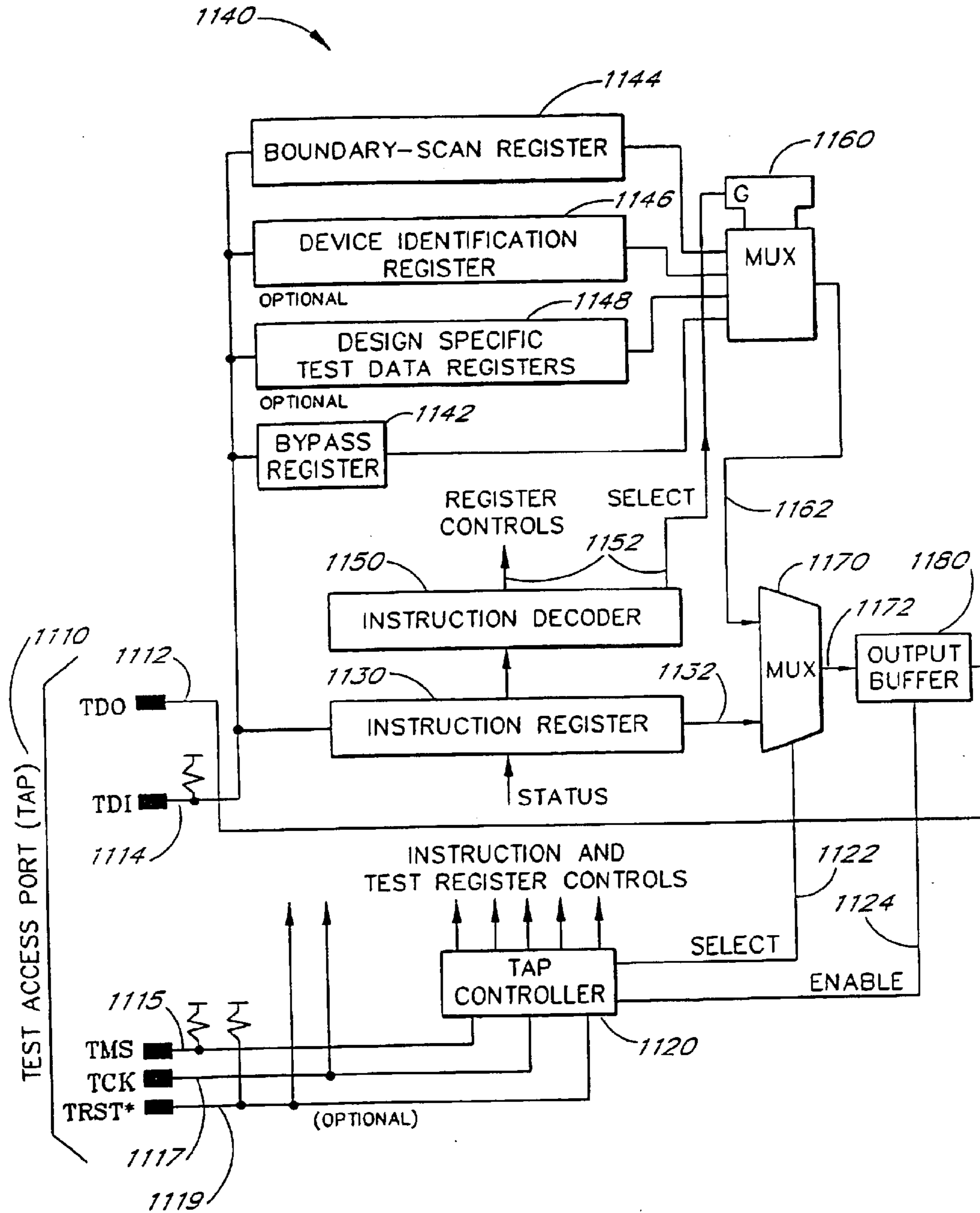
FIG. 11 (PRIOR ART)
