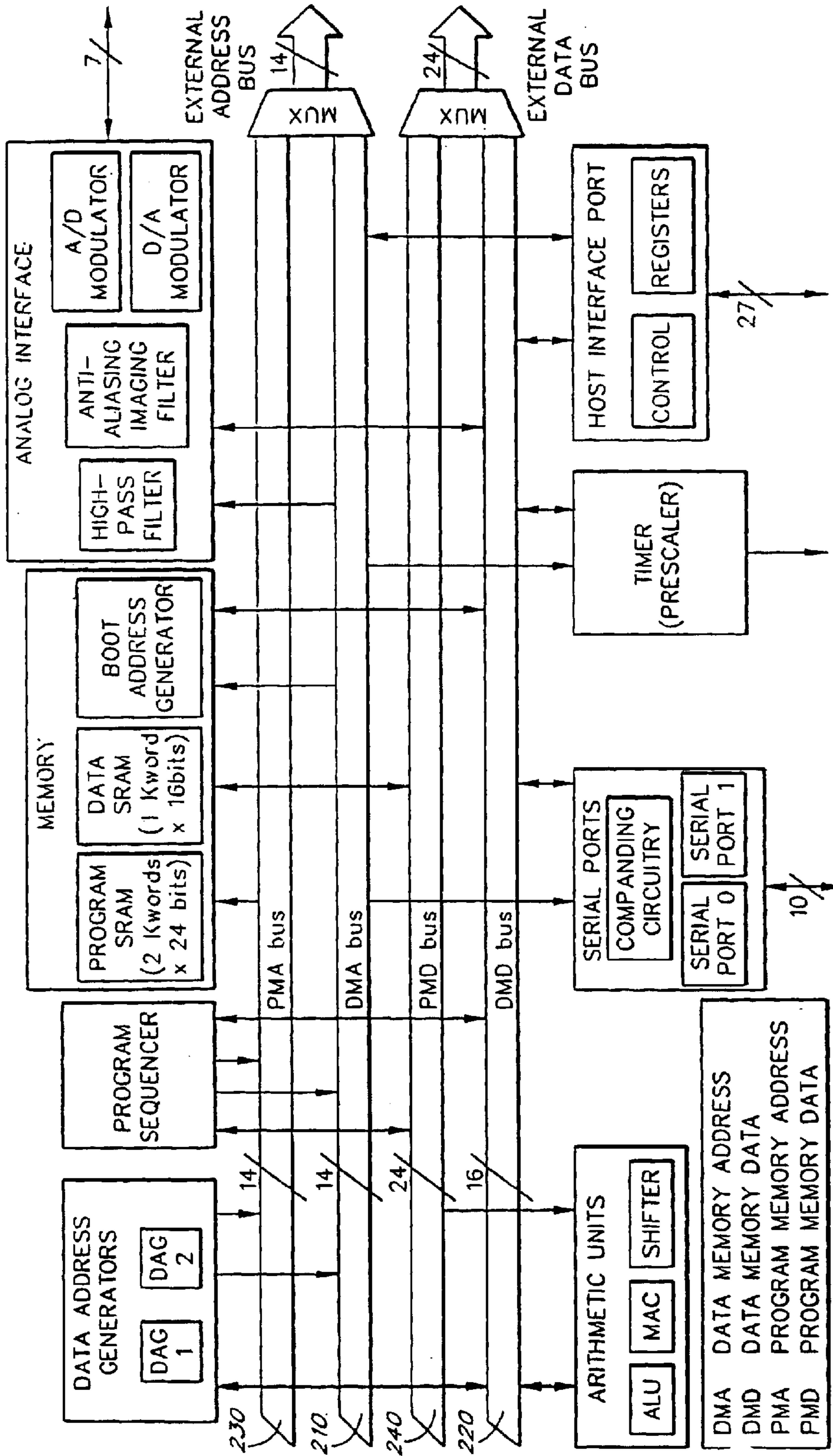
FIG. 2 (PRIOR ART)
