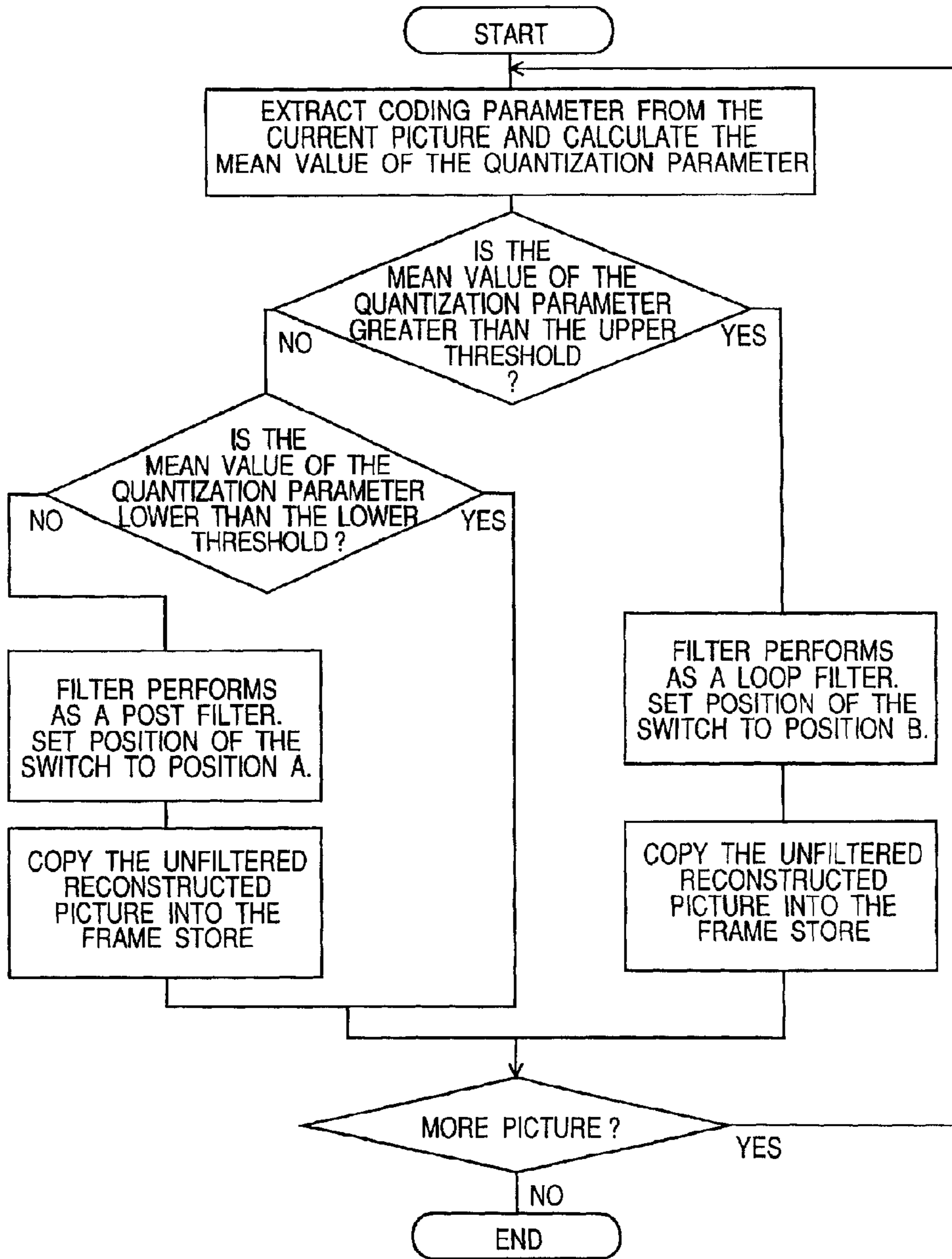
FLOWCHART FOR 3-STATE DYNAMIC SWITCHING DECISION
