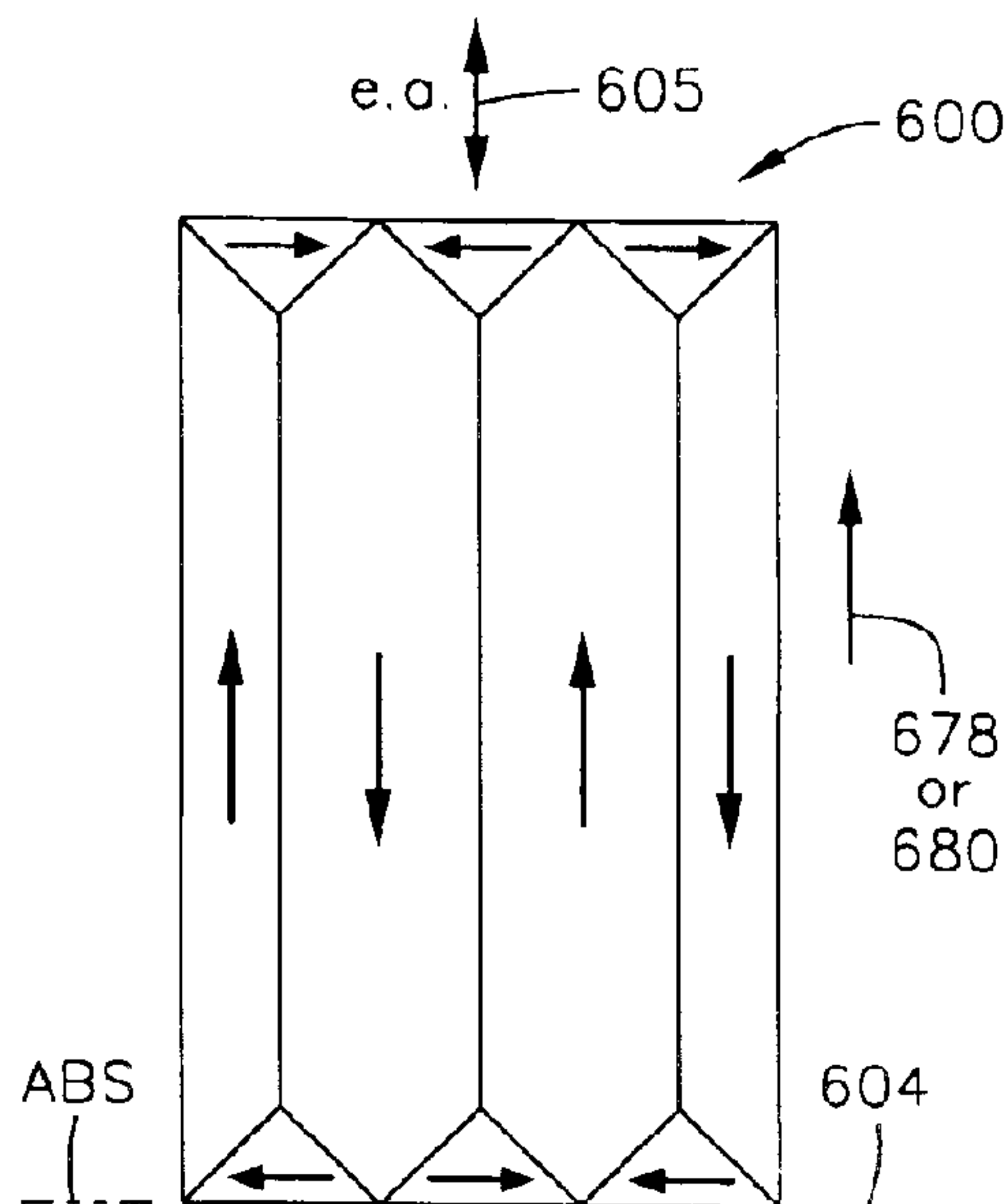
FIG. 28B (PRIOR ART)
