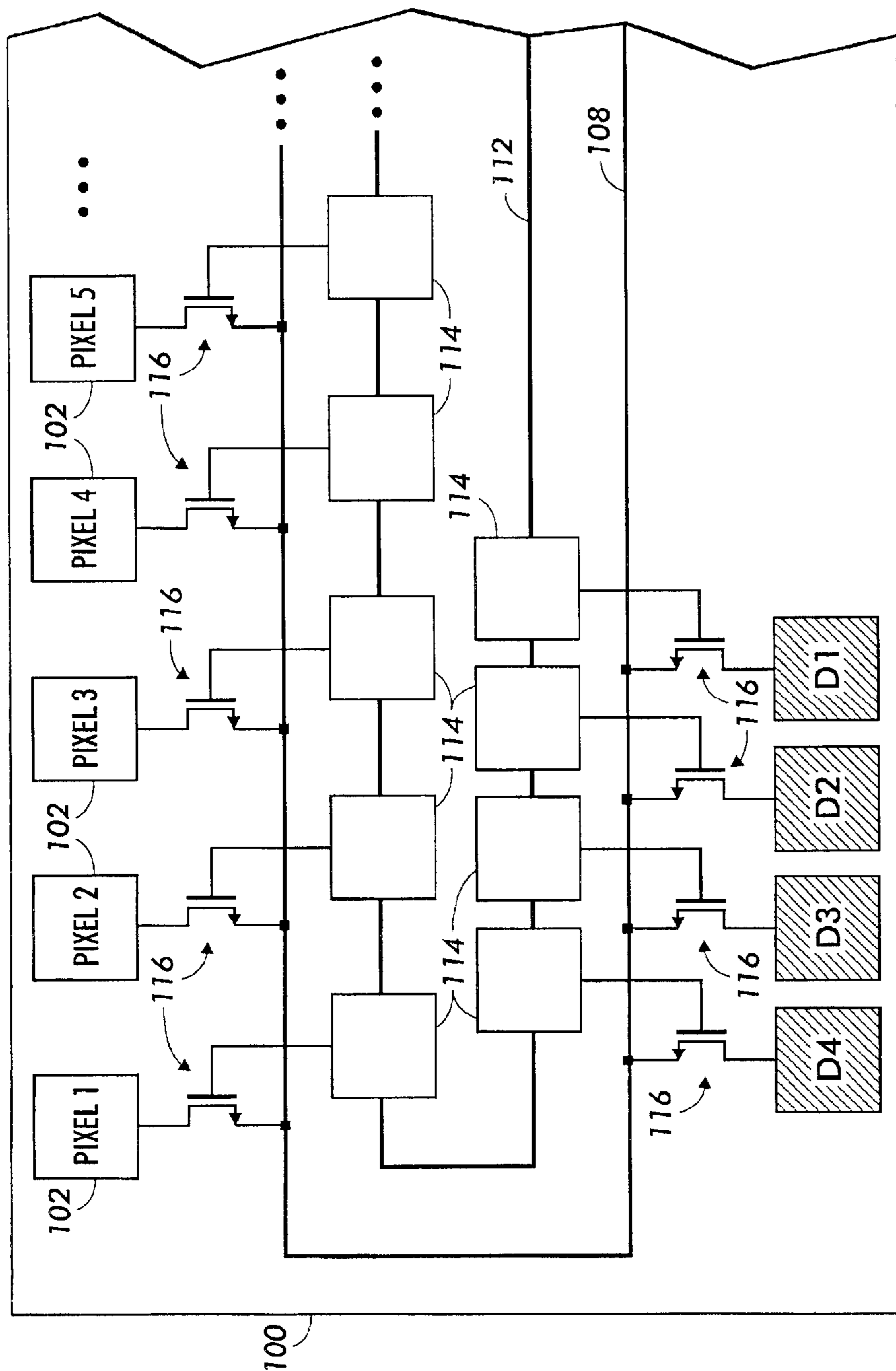
FIG. 1 PRIOR ART
