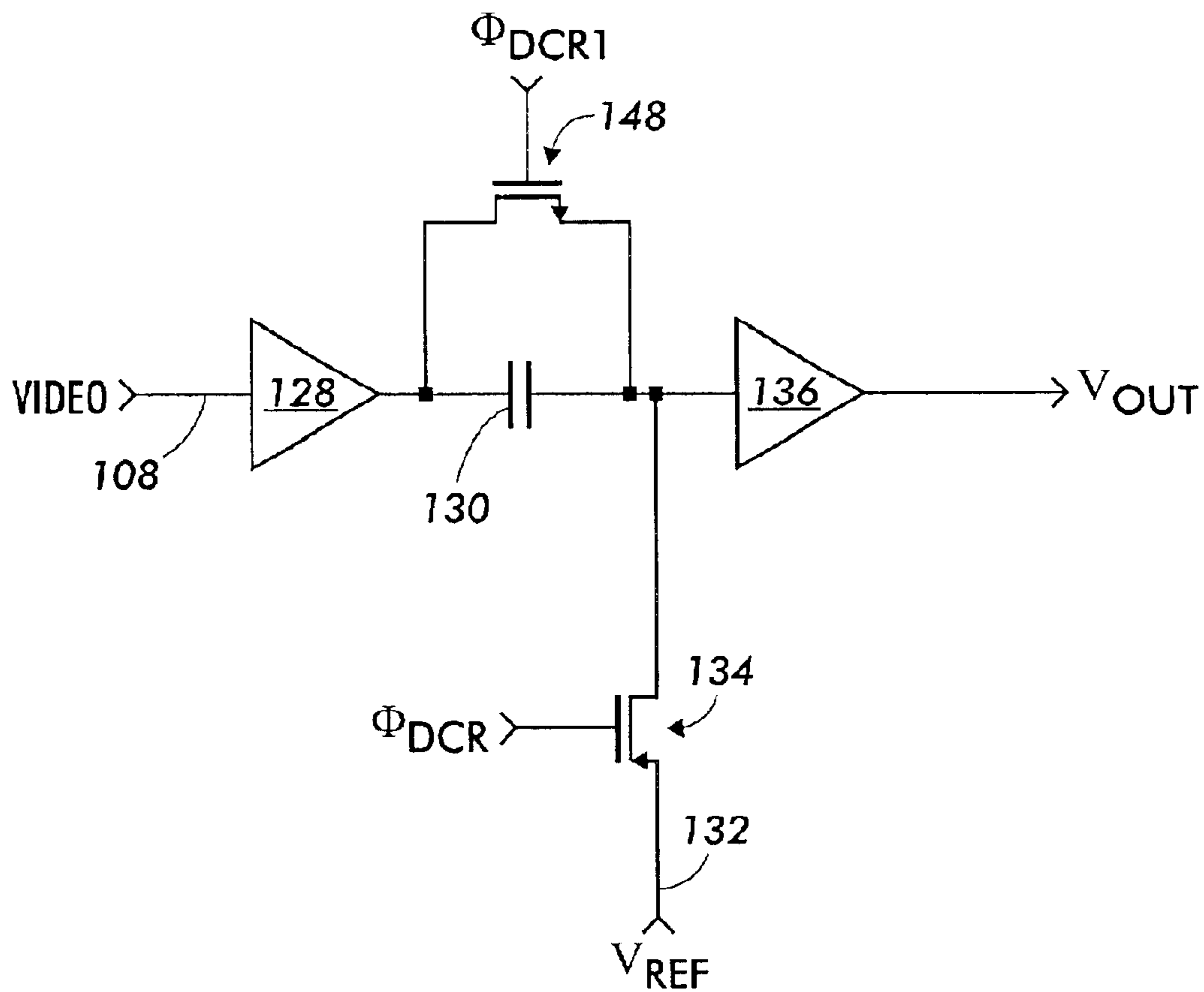
FIG. 2 PRIOR ART
