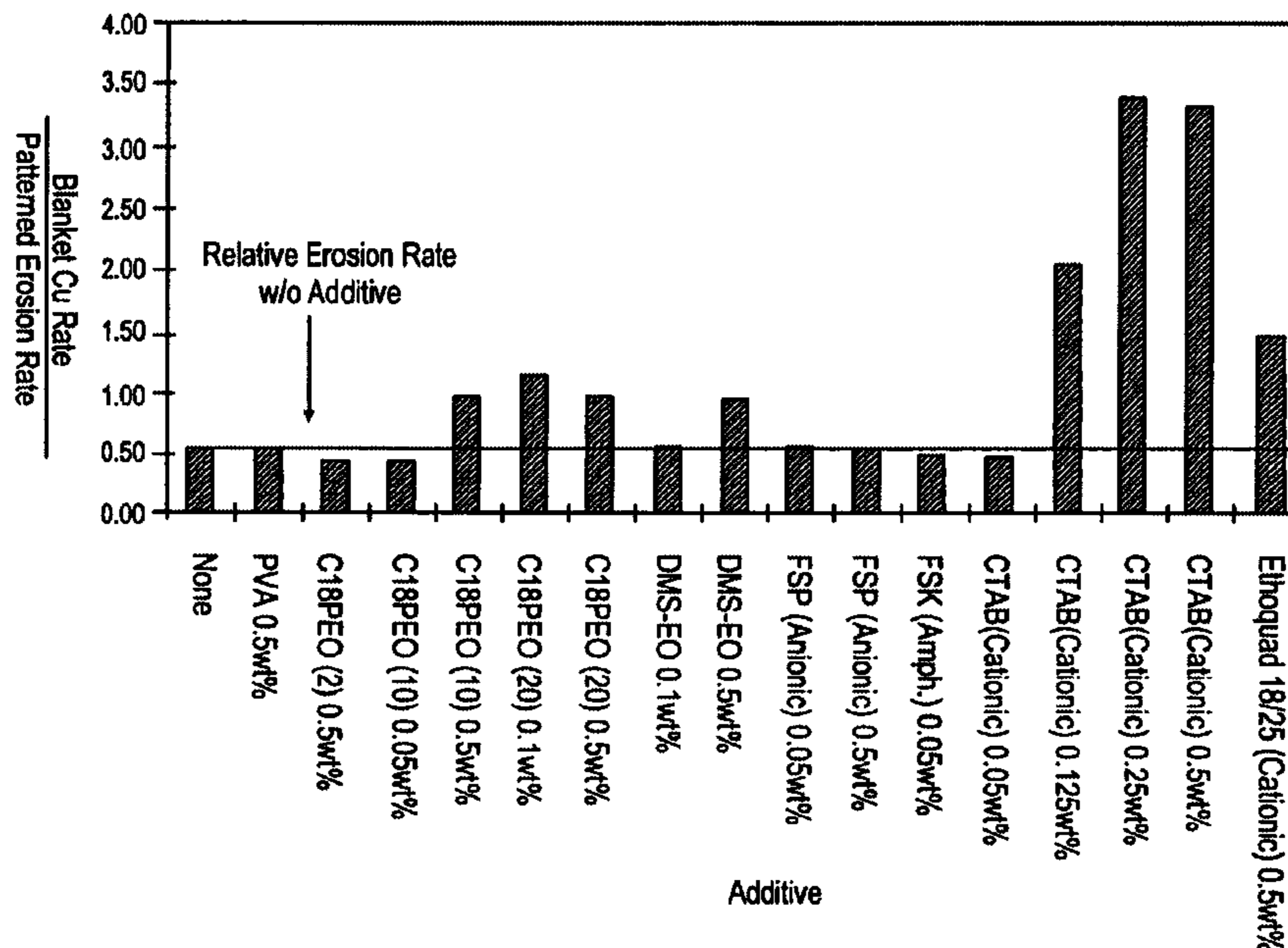
Surfactant Effects on Relative Erosion Rates
