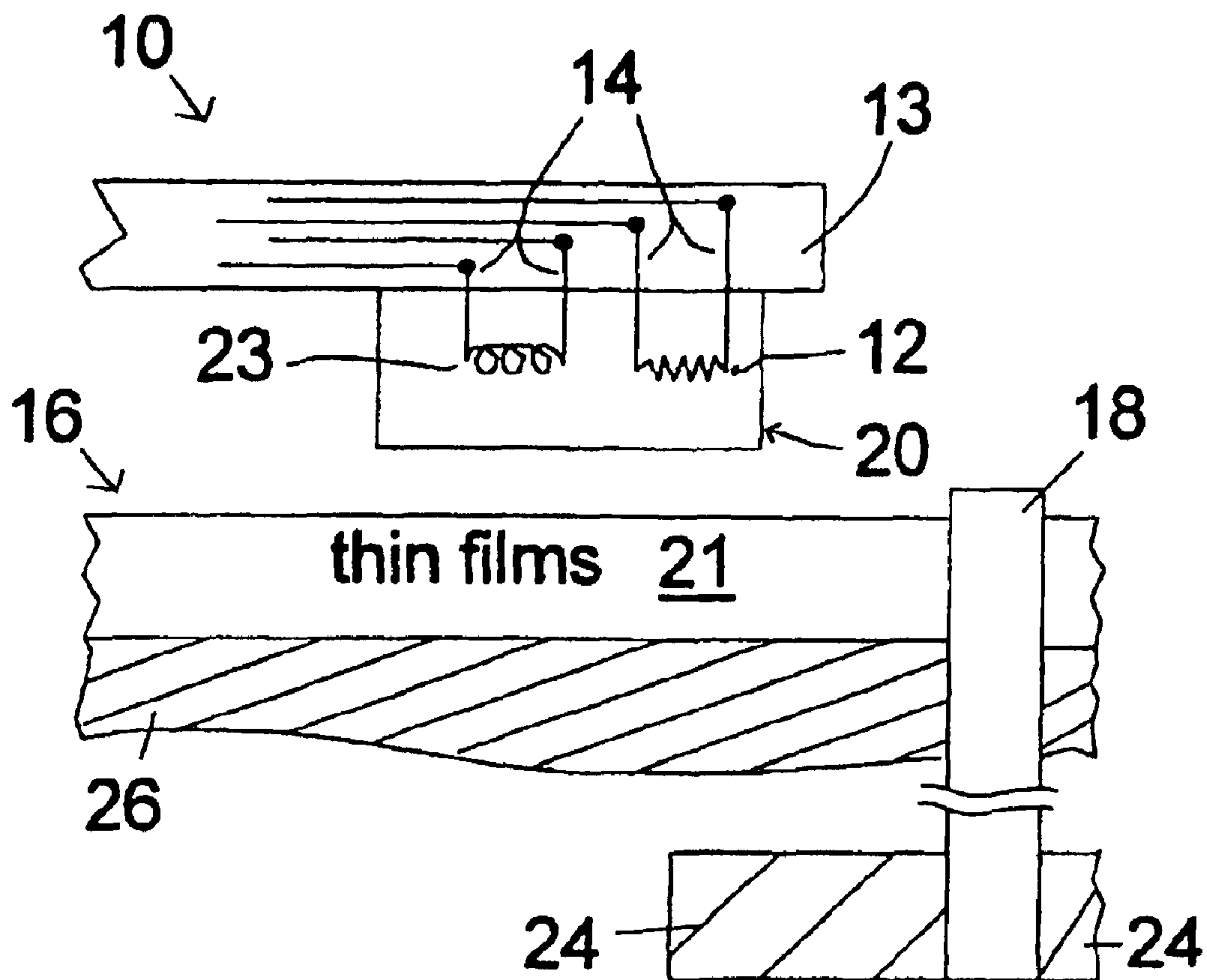
Figure 1 (prior art)
