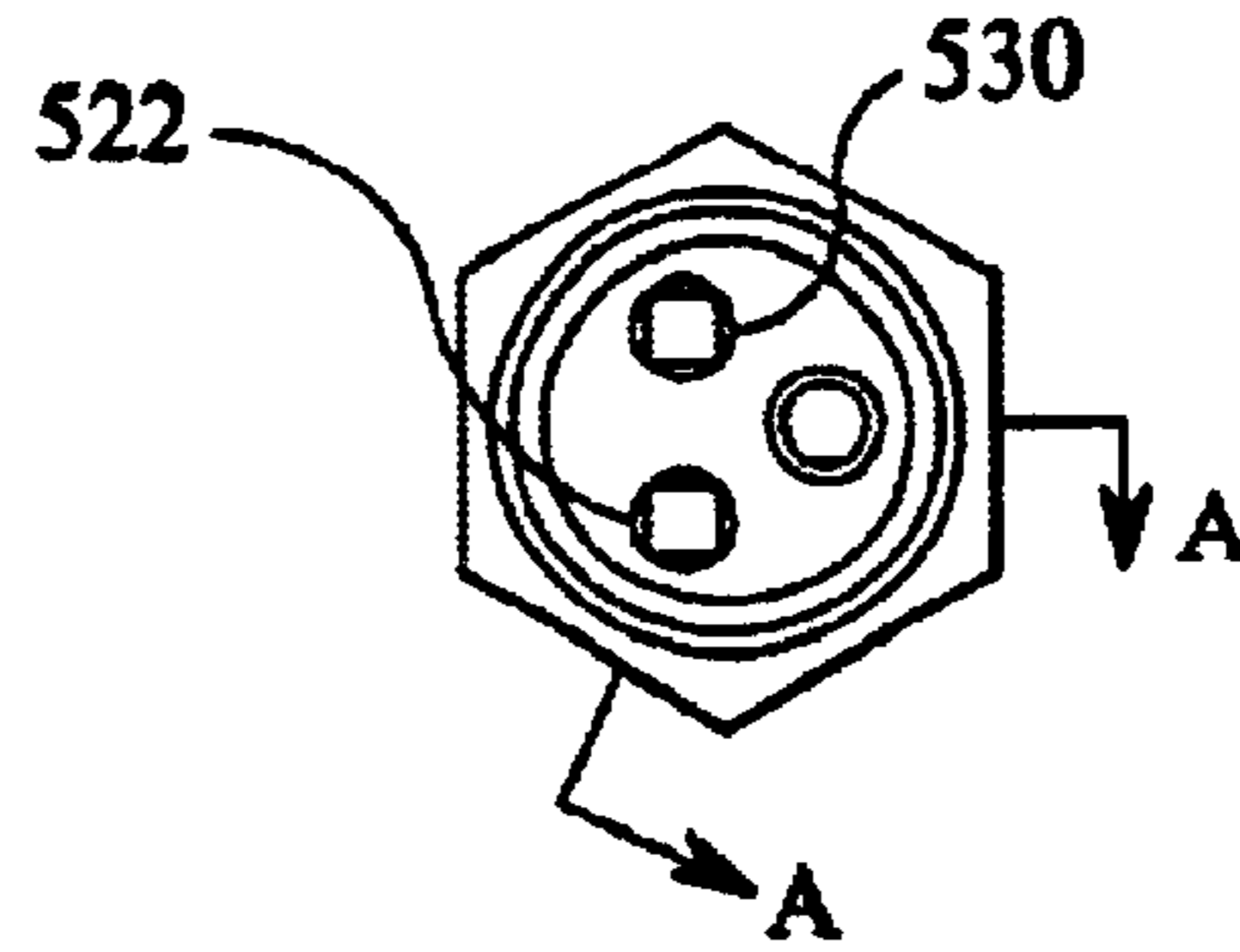
FIG 3 bottom view
