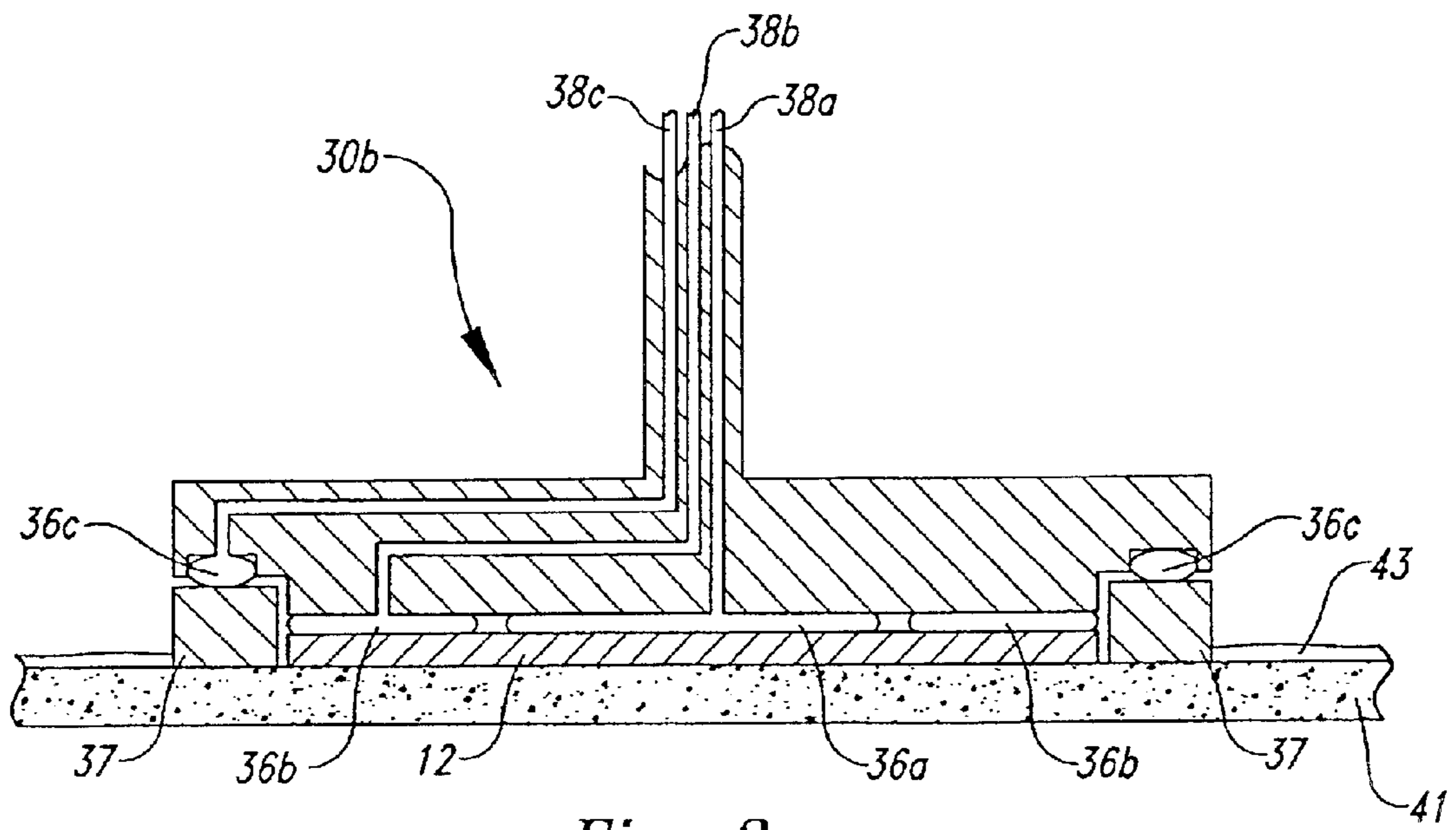
Fig. 3 (Prior Art)
