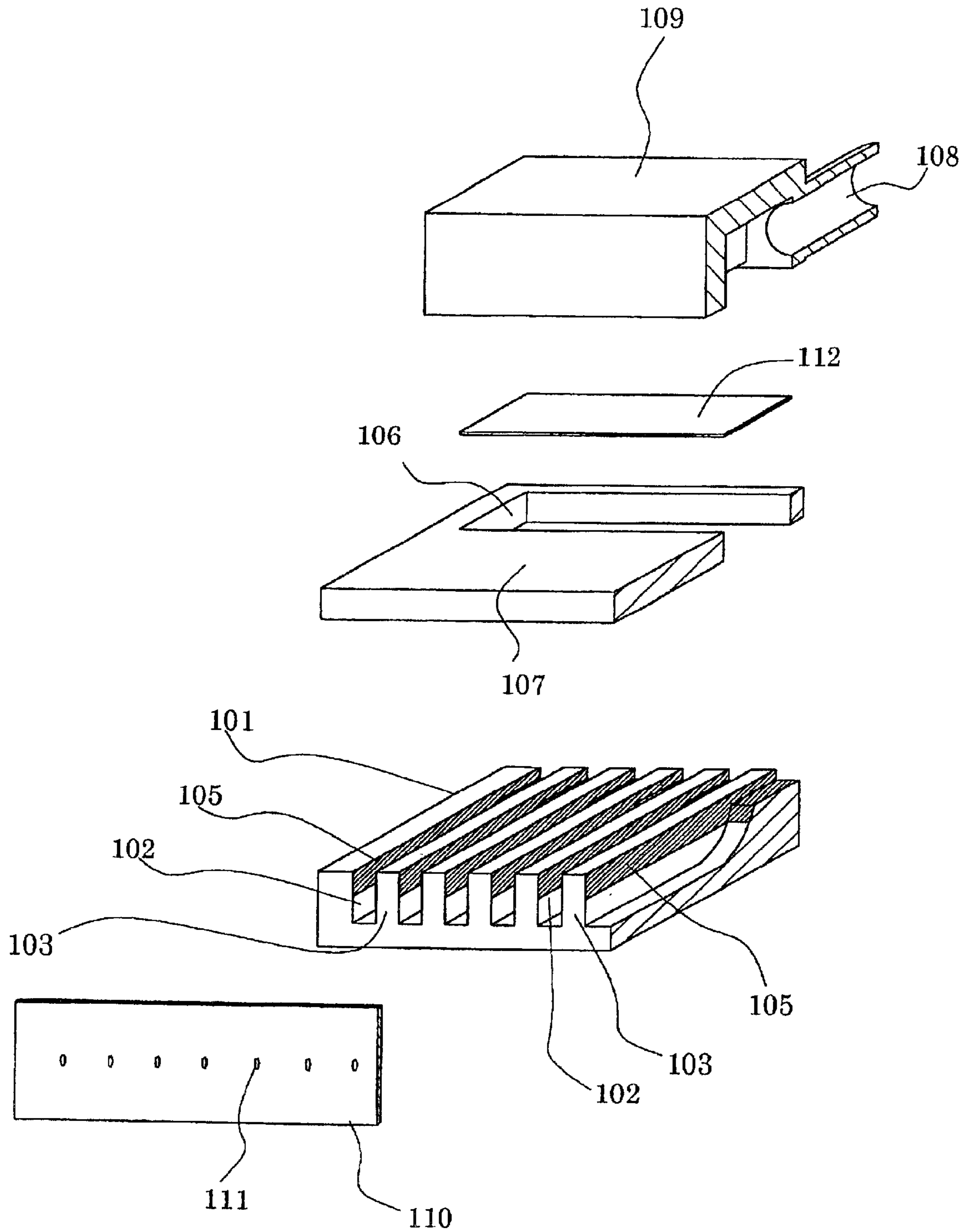
FIG. 7 PRIOR ART
