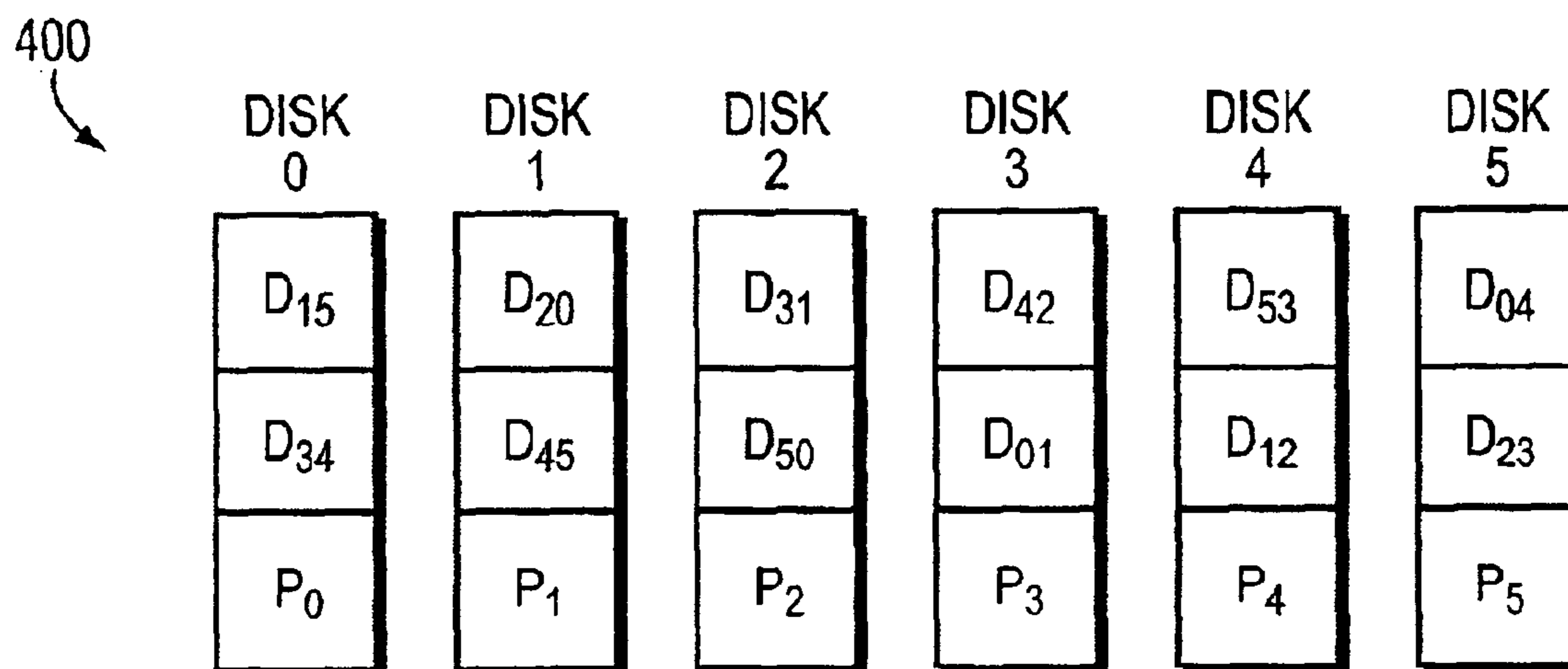
FIG. 4 (PRIOR ART)
