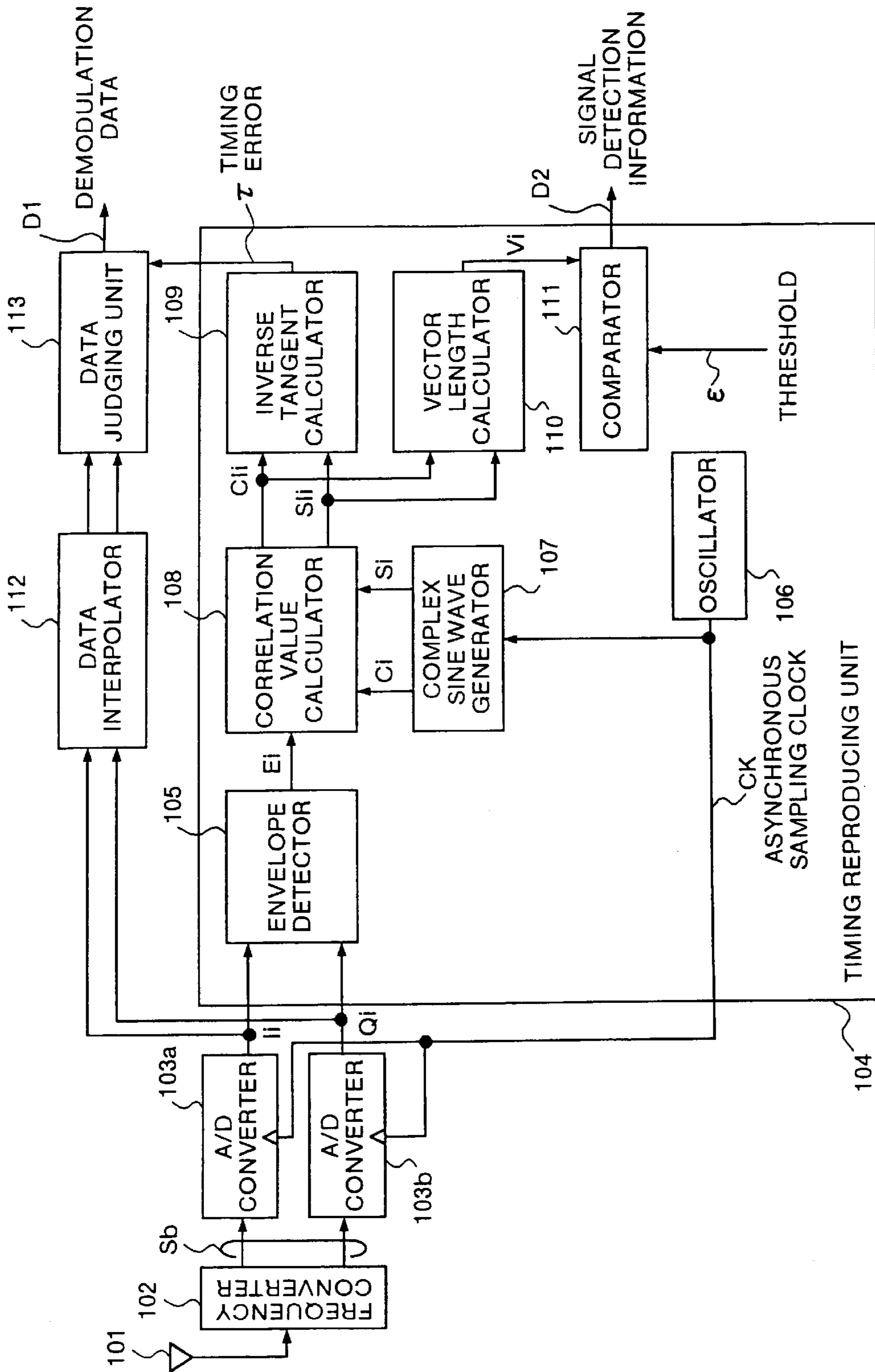
FIG.10 BACKGROUND ART
