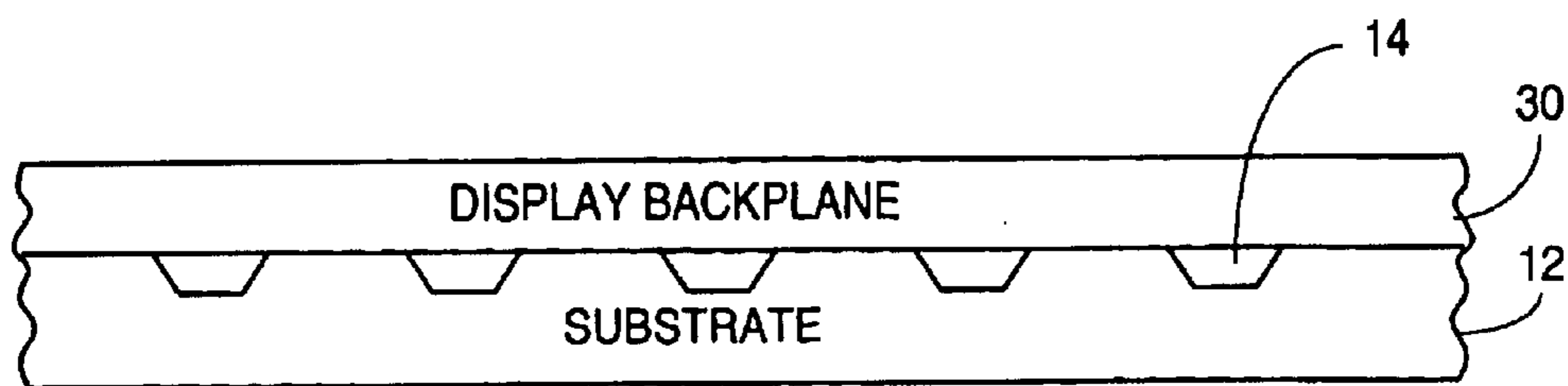
Fig. 4 (Prior Art)
