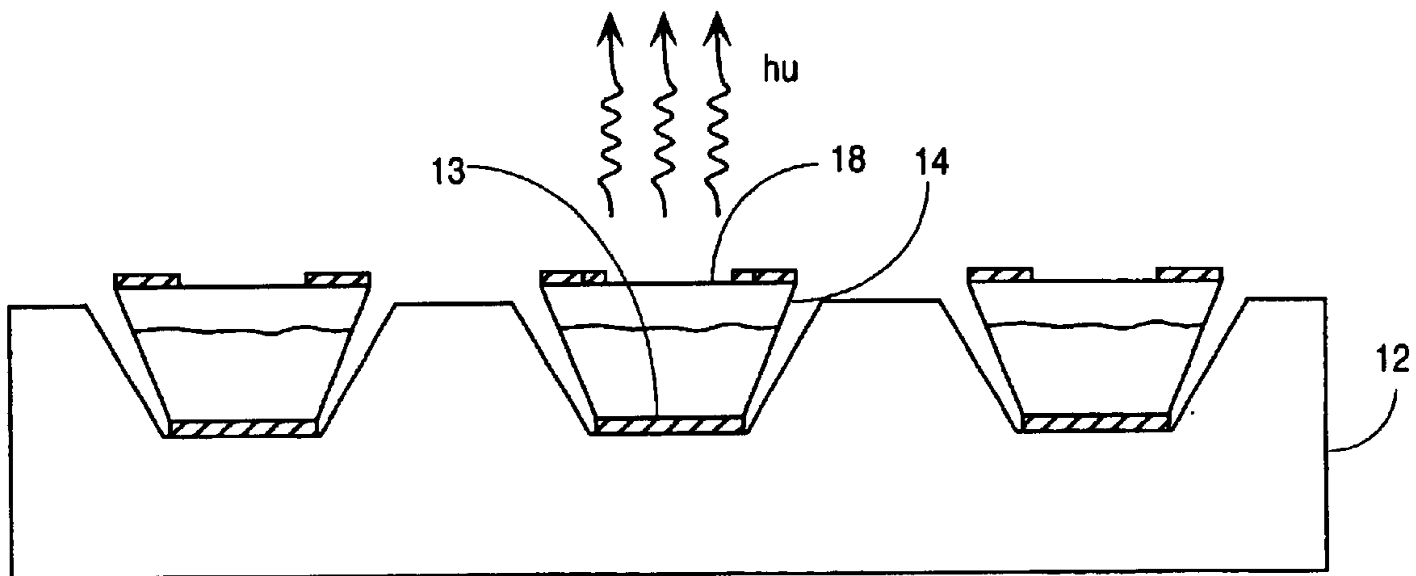
Fig. 3 (Prior Art)
