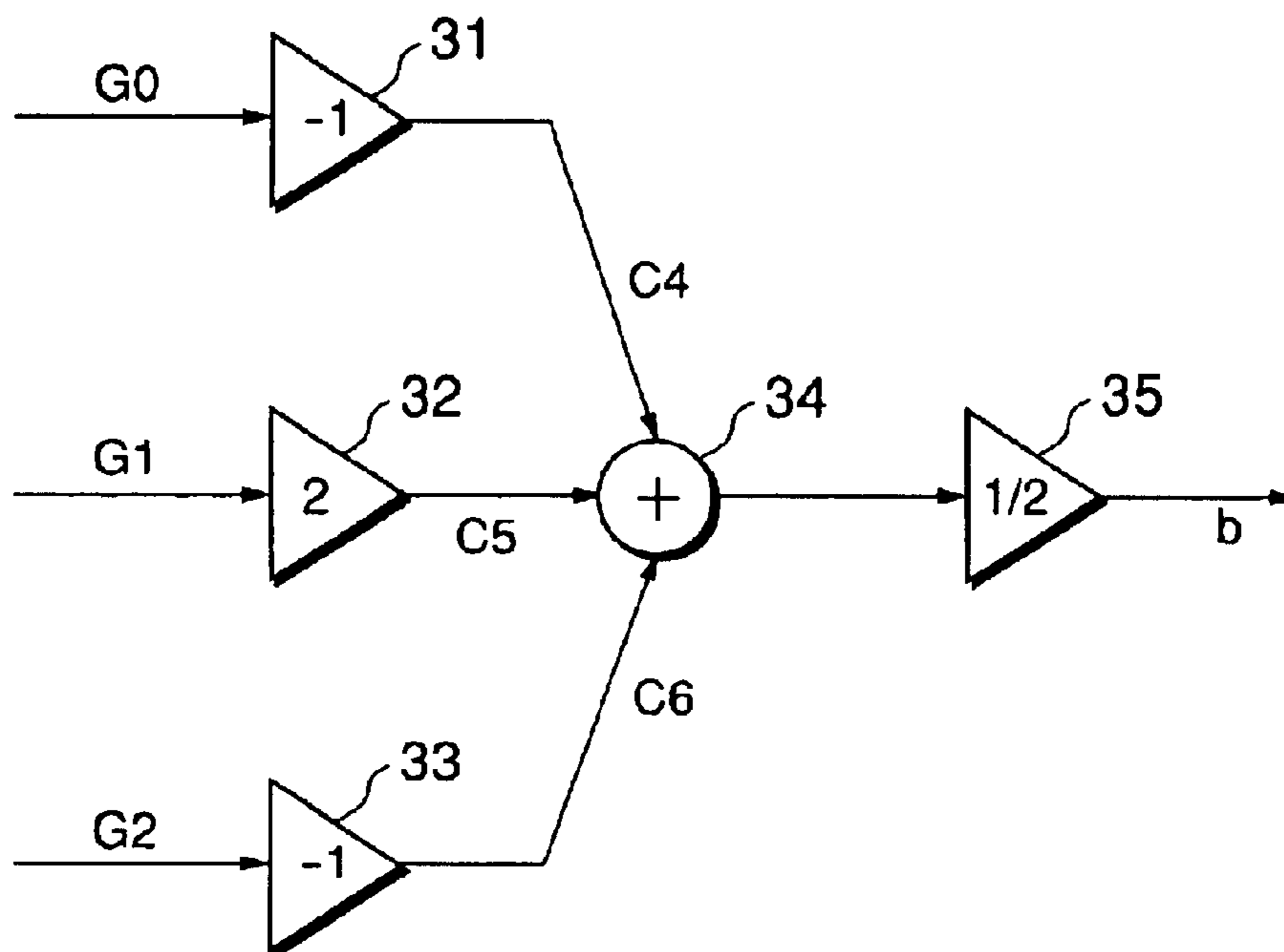
FIG.4 PRIOR ART
