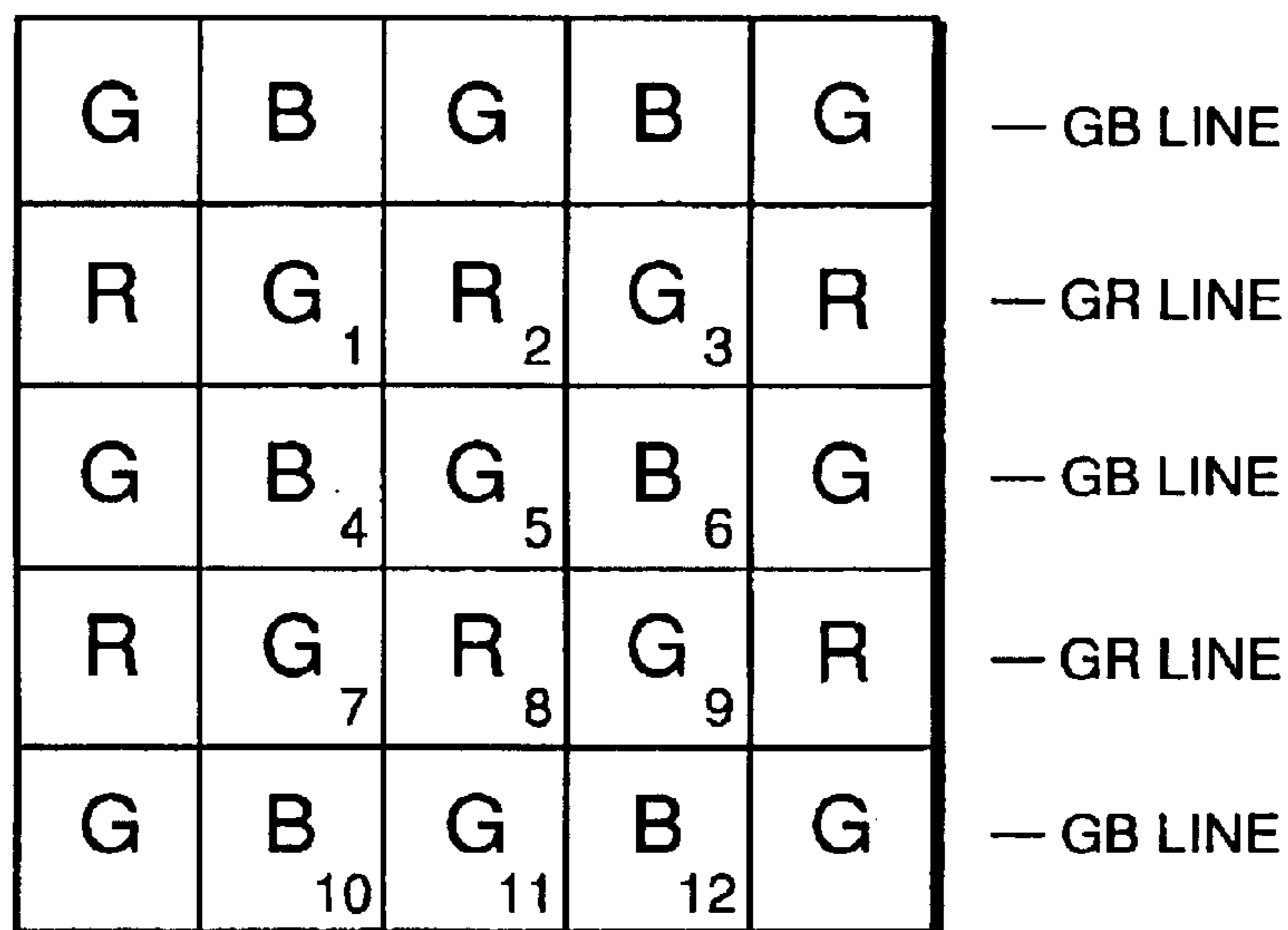
FIG.2 PRIOR ART
