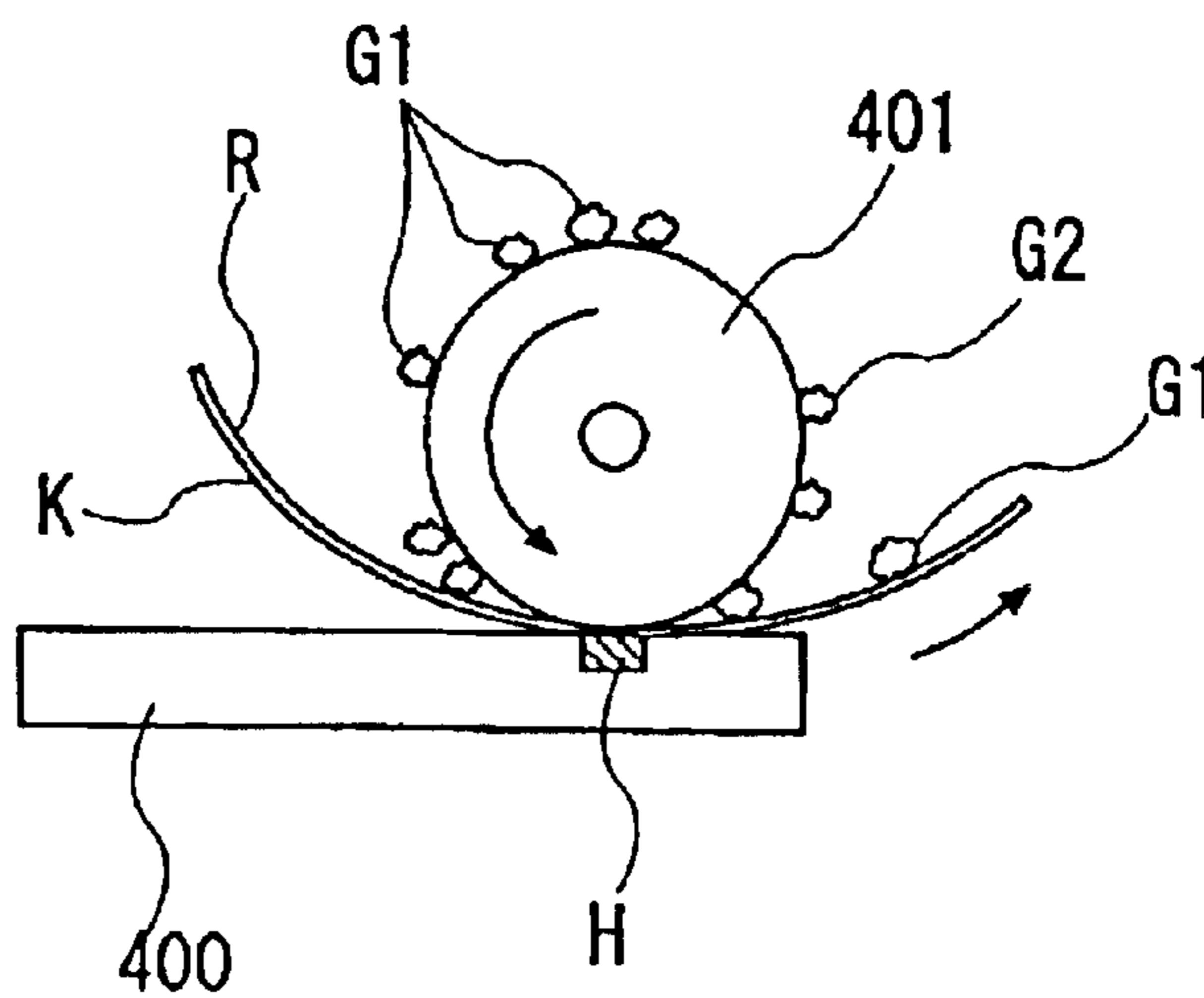
FIG. 8C PRIOR ART
