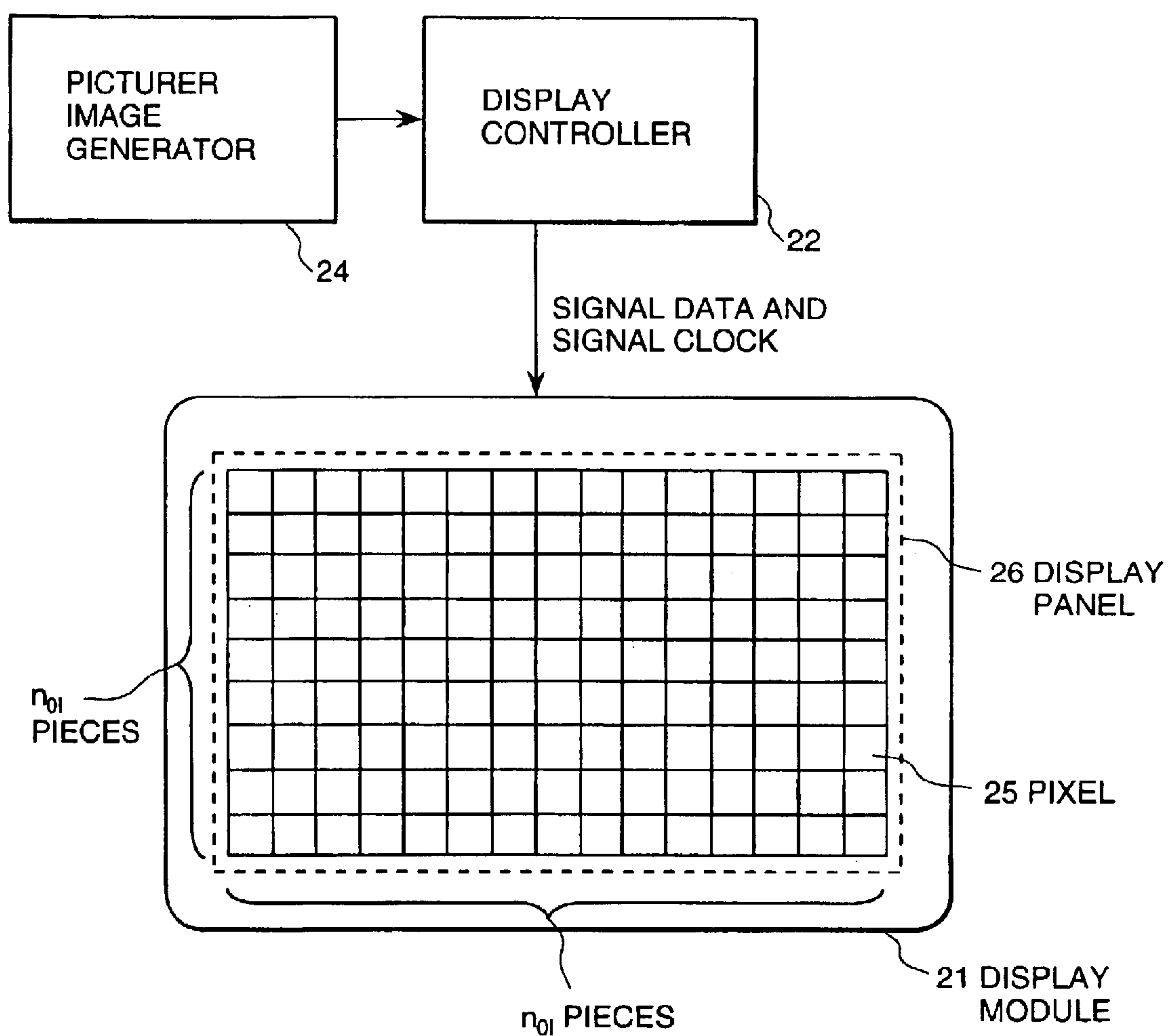
FIG. 2 - PRIOR ART
