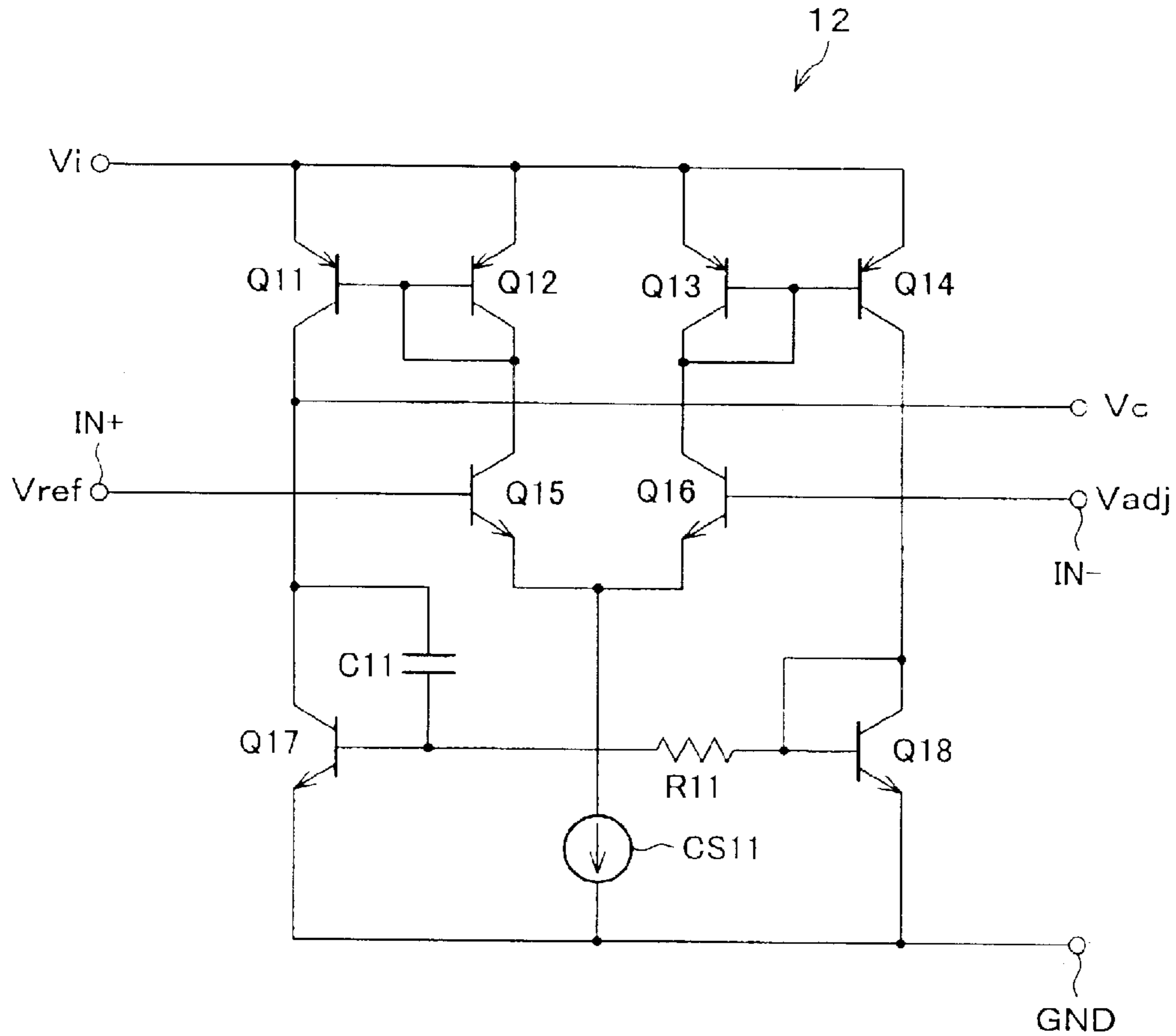
FIG. 7 (PRIOR ART)
