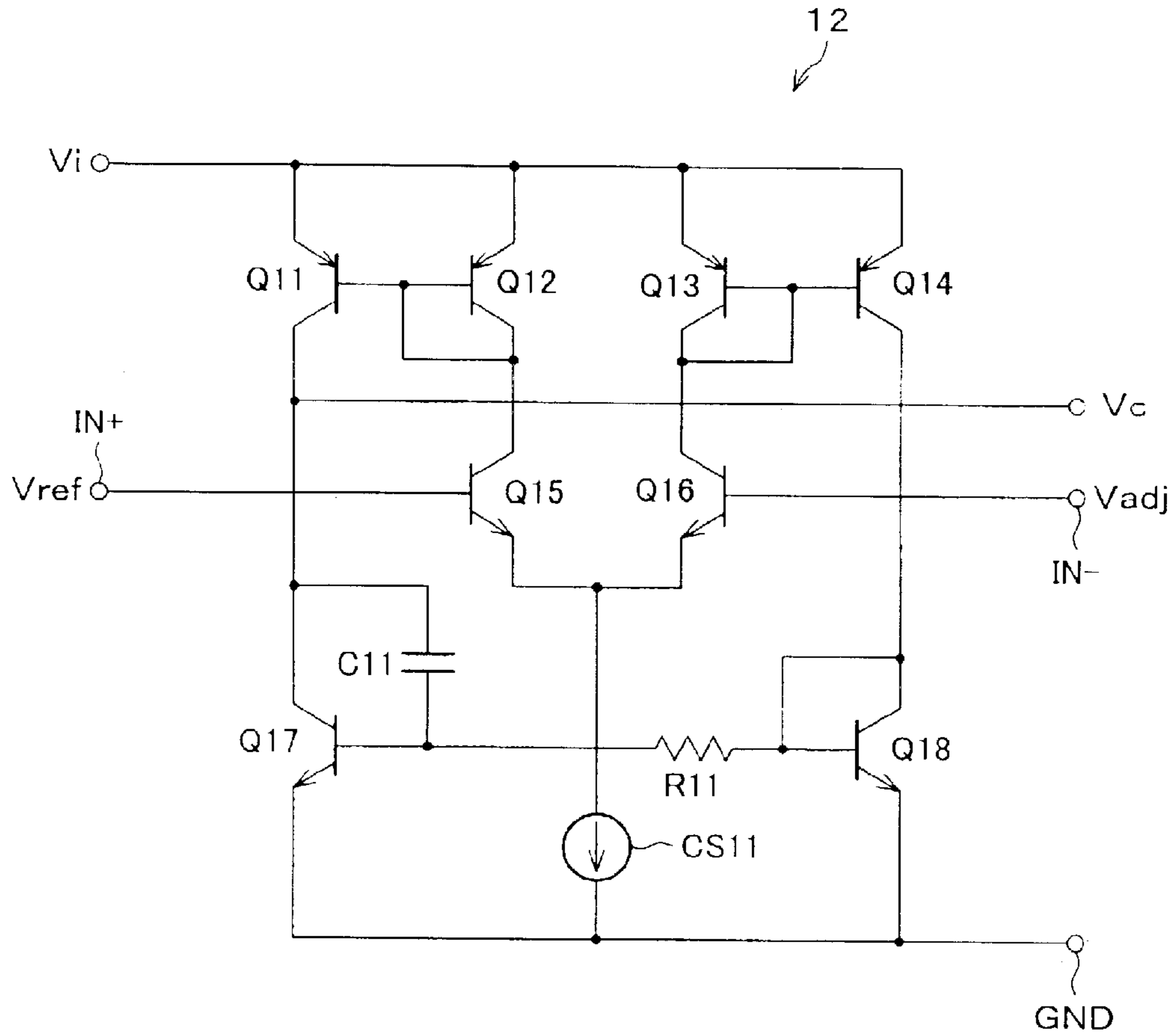
FIG. 7 (PRIOR ART)
