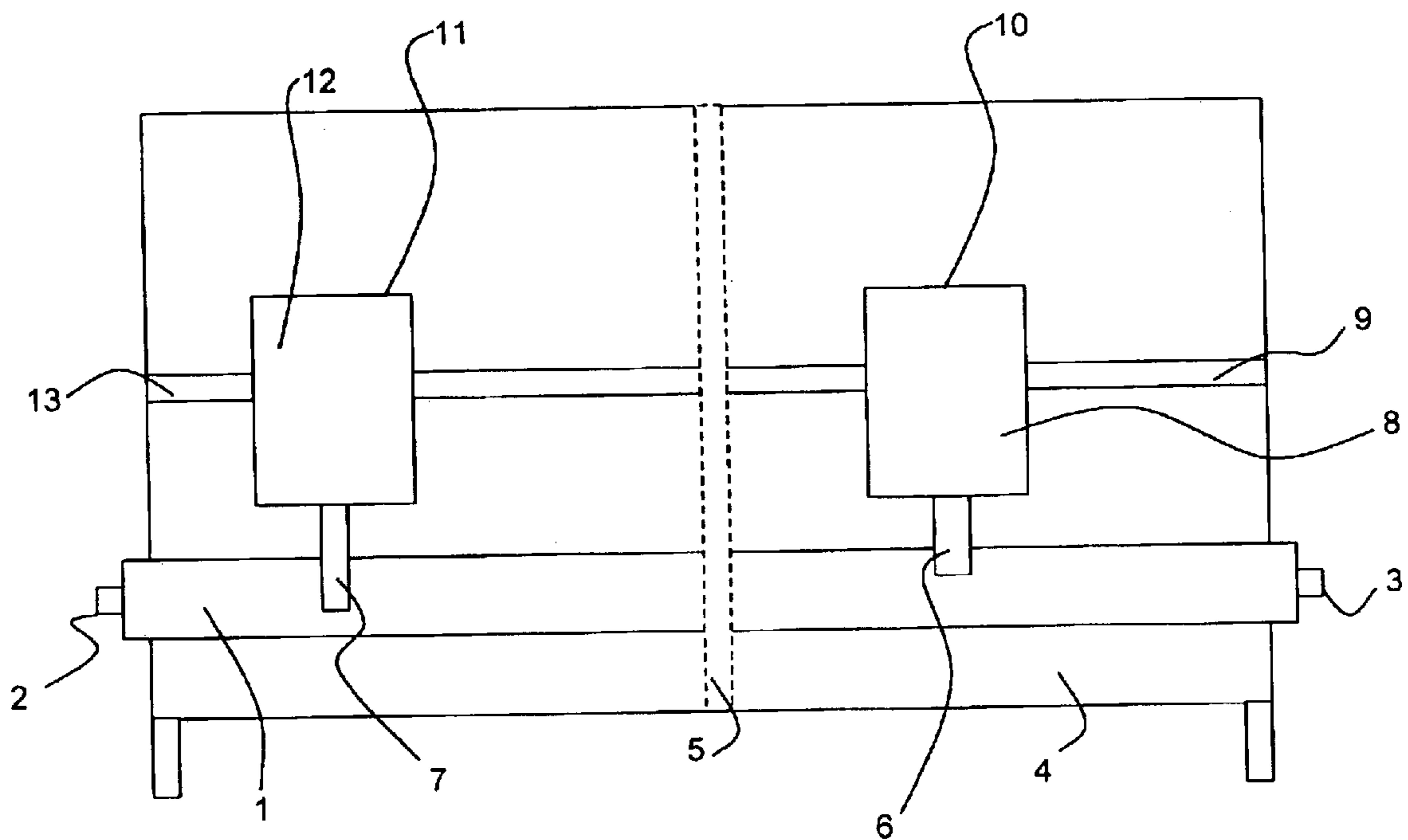
FIG. 2: Prior Art: Pre-matching tuner structure
