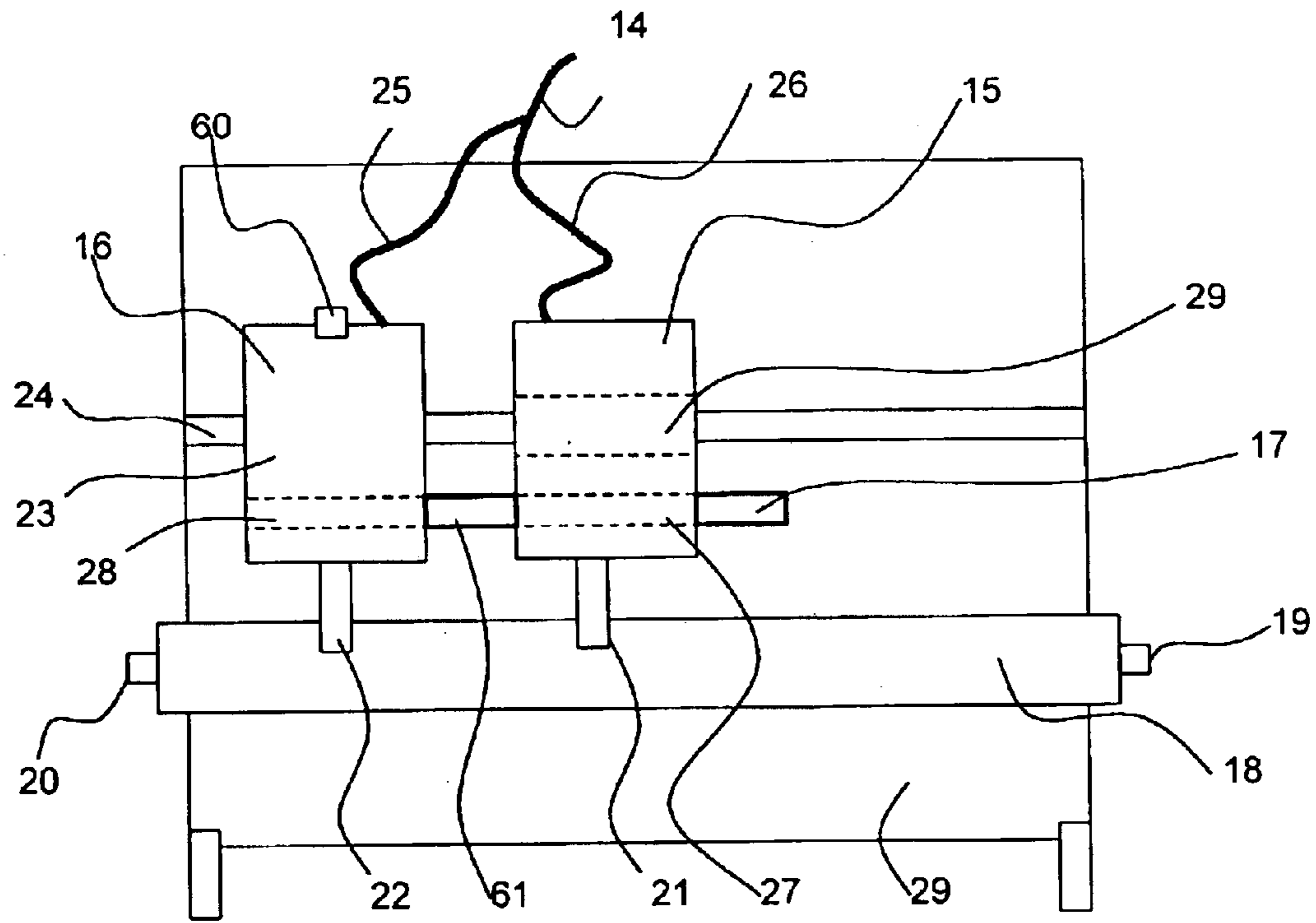
FIG. 3: Synchronized pre-matching tuner structure
