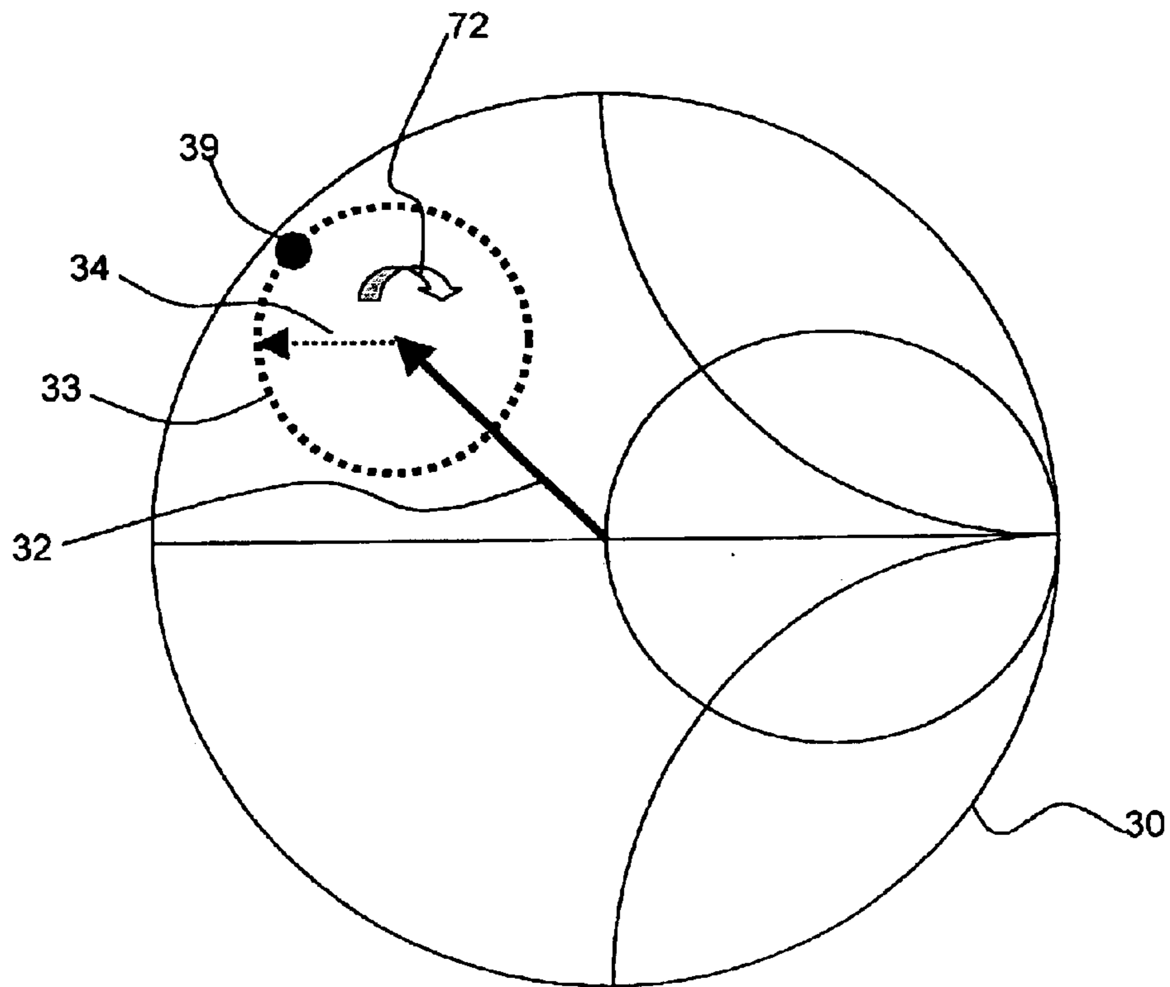
FIG. 4: Prior Art: Tuning mechanism of pre-matching tuner
