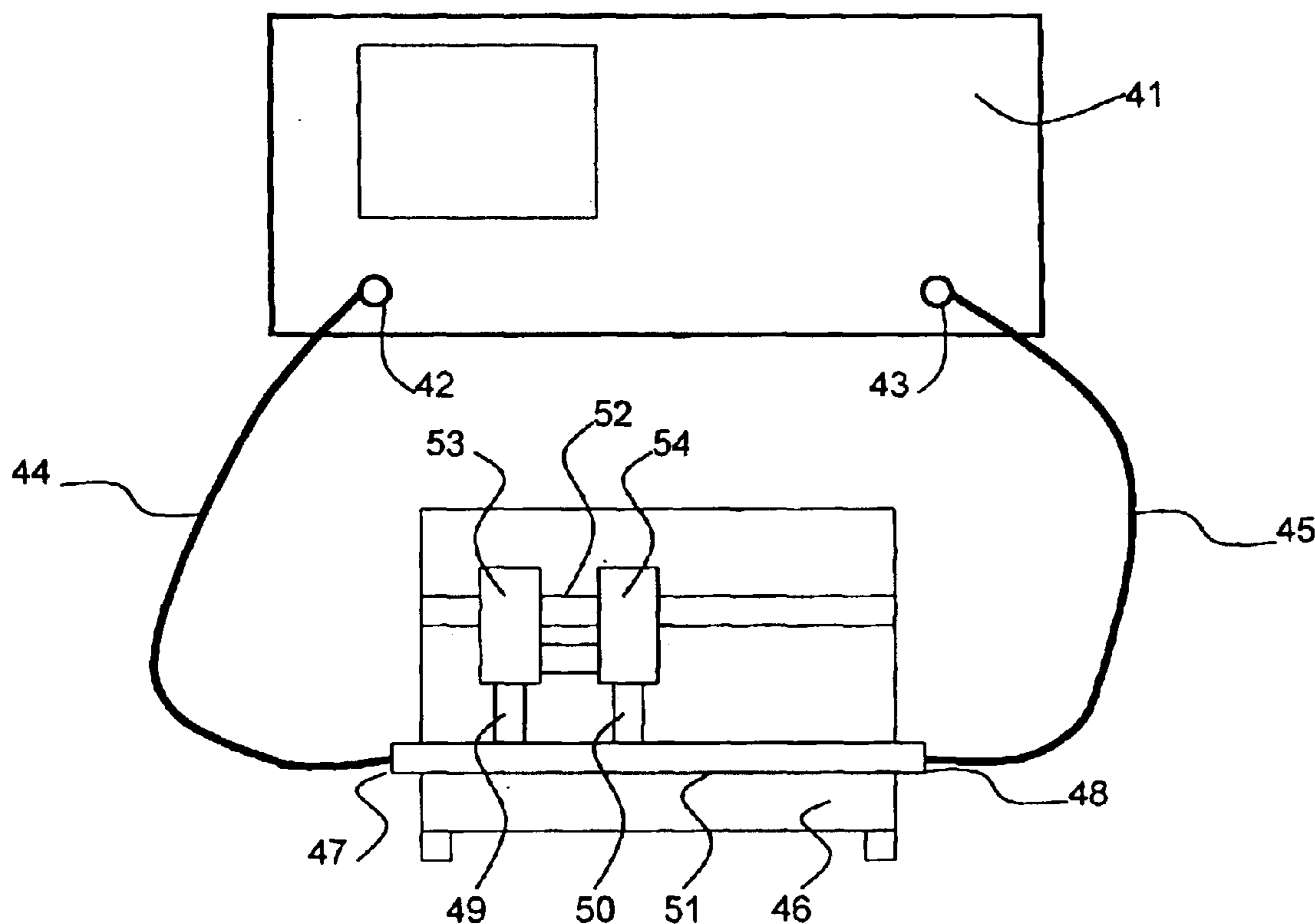
Setup for tuner calibration
