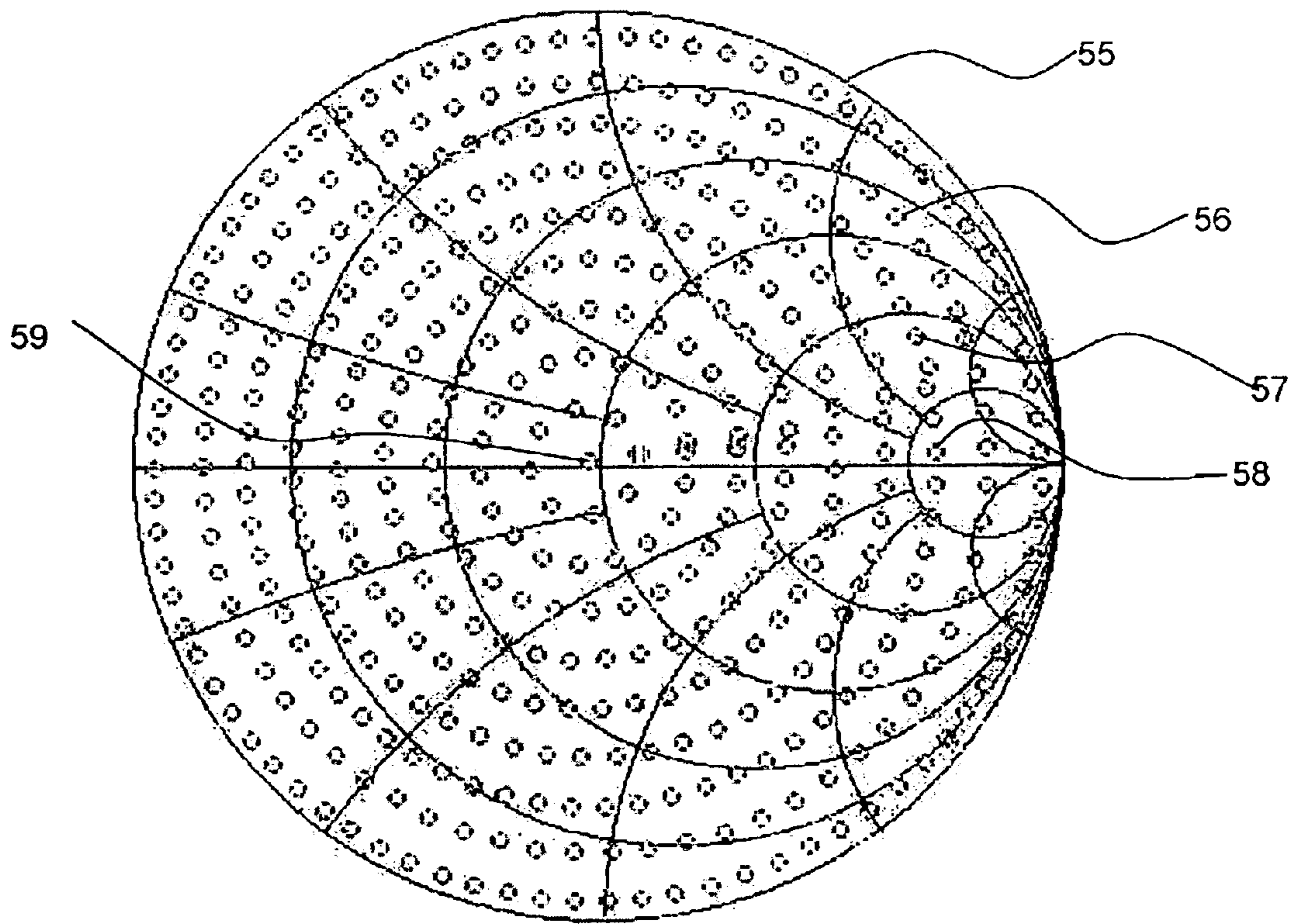
FIG. 8: Calibration point distribution of synchronized pre-matching tuners.
