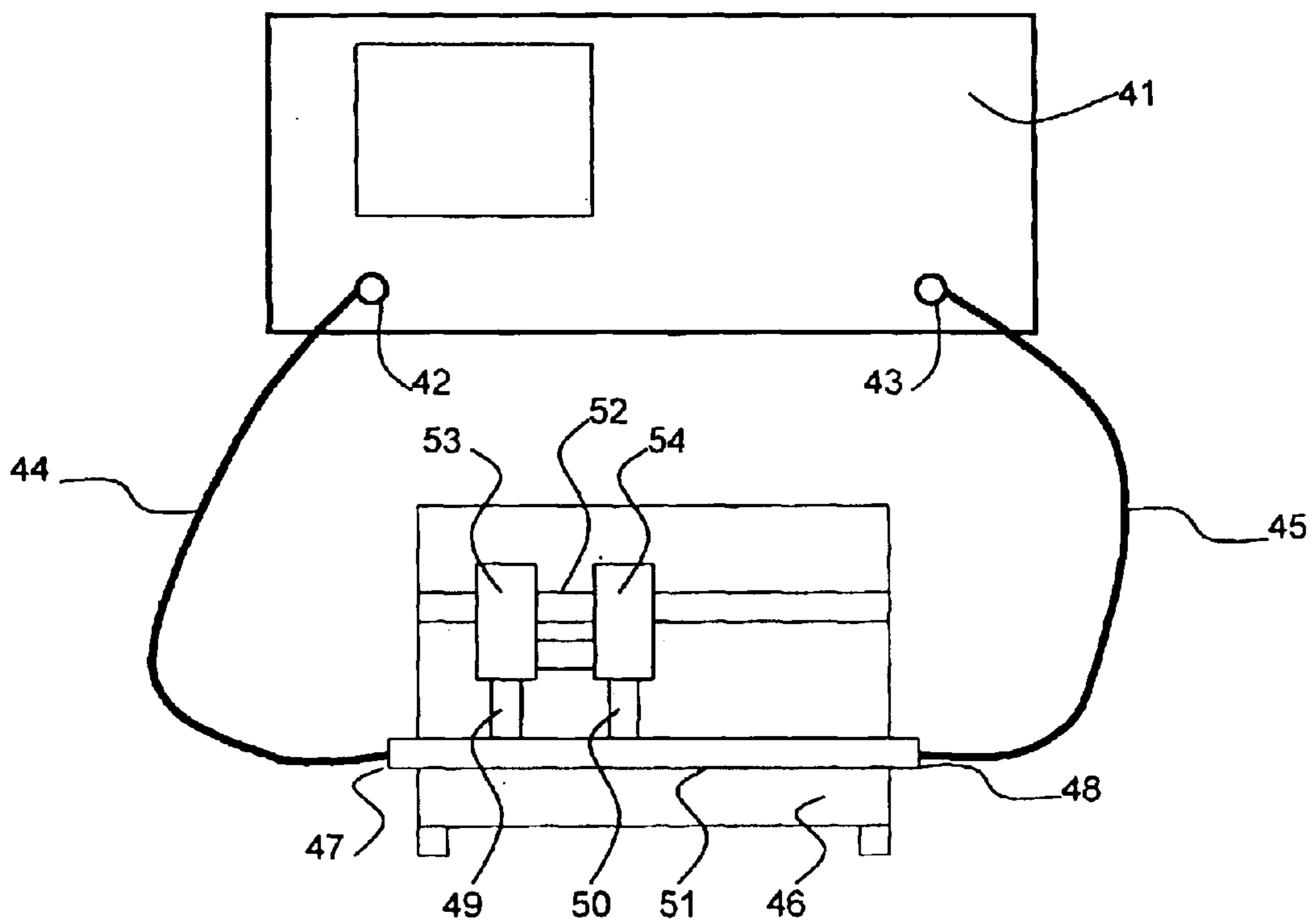
FIG. 6: Setup for tuner calibration
