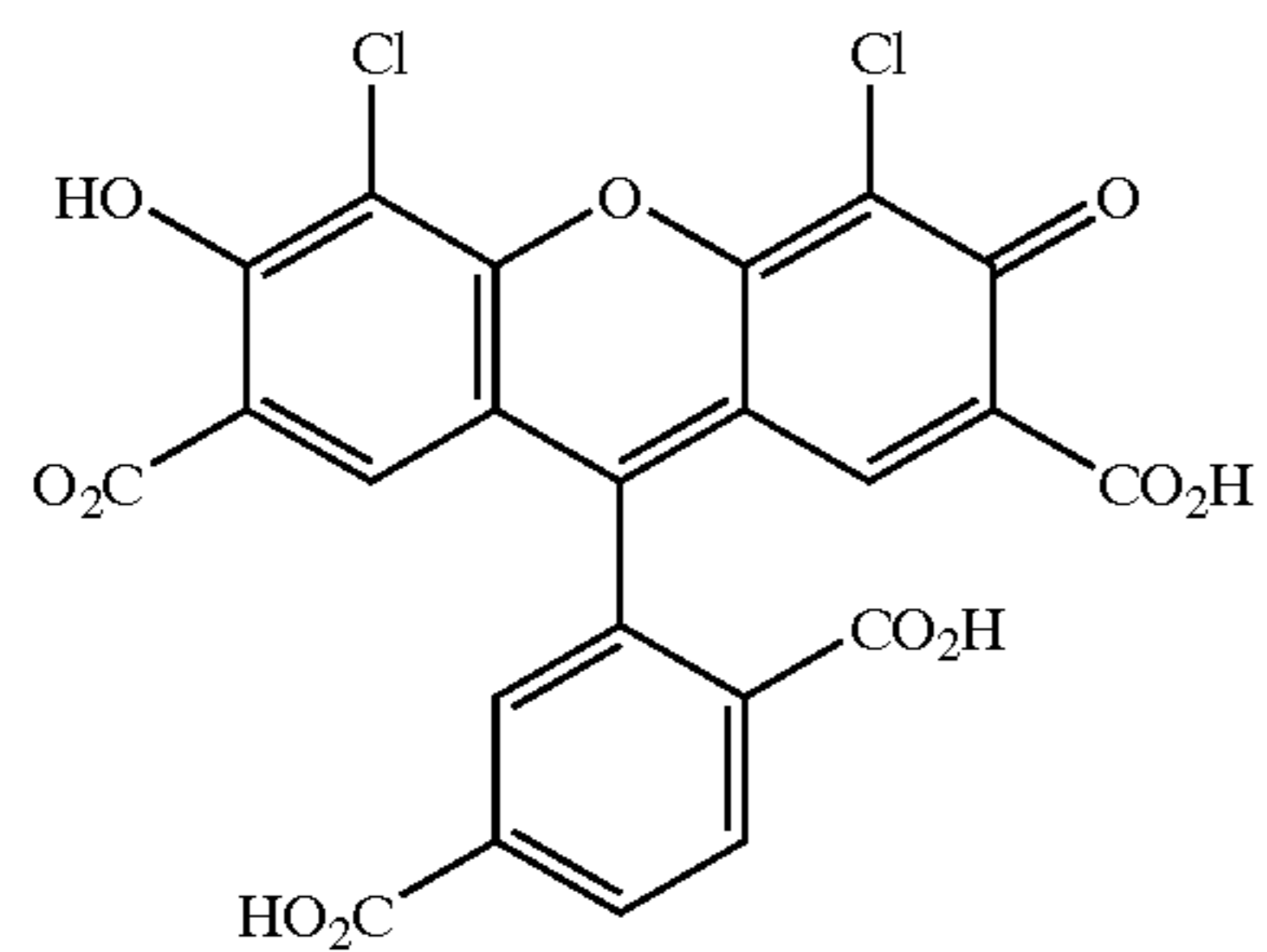
JOE
