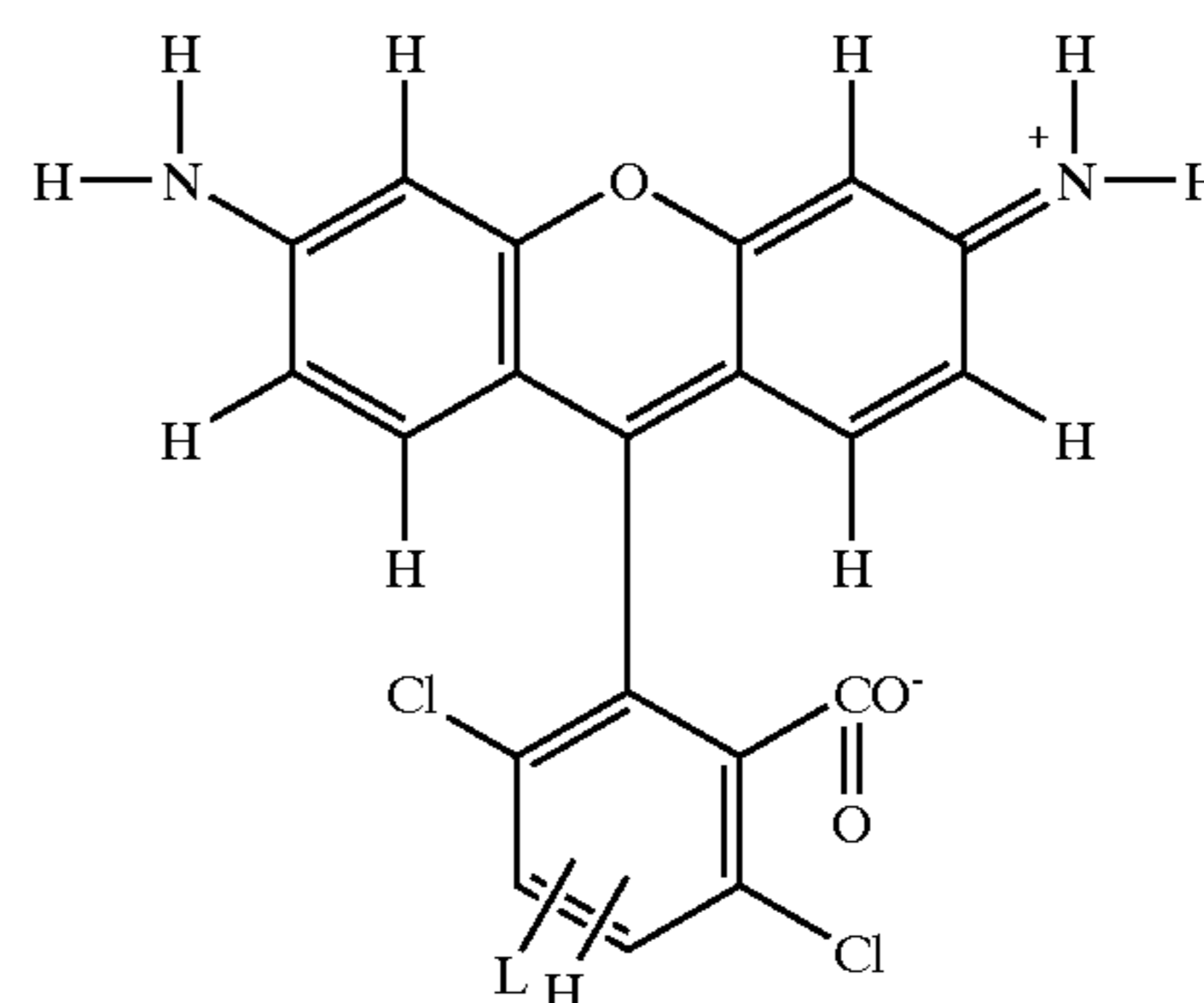
DR110-2
