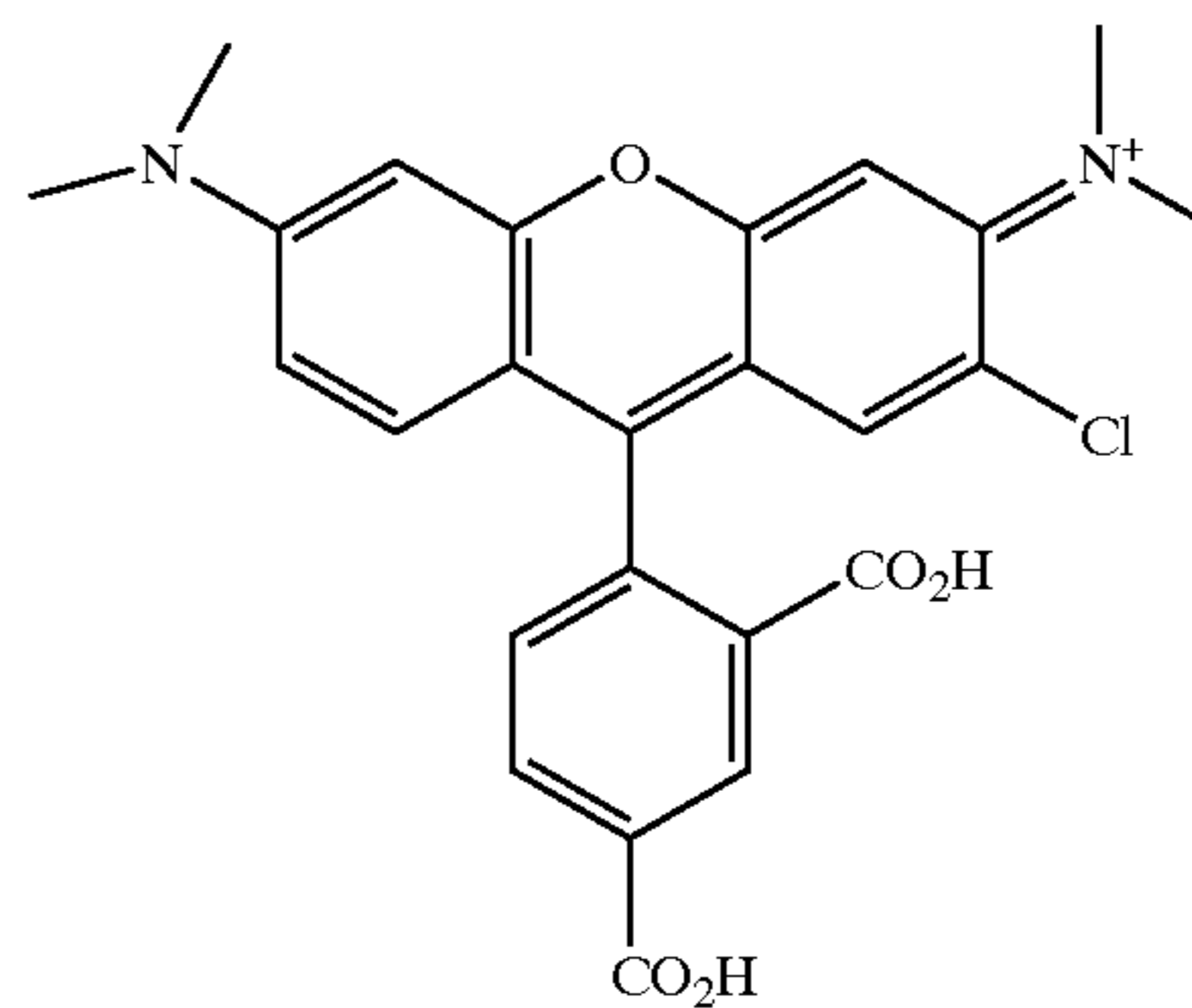
5-carboxyrhodamine
