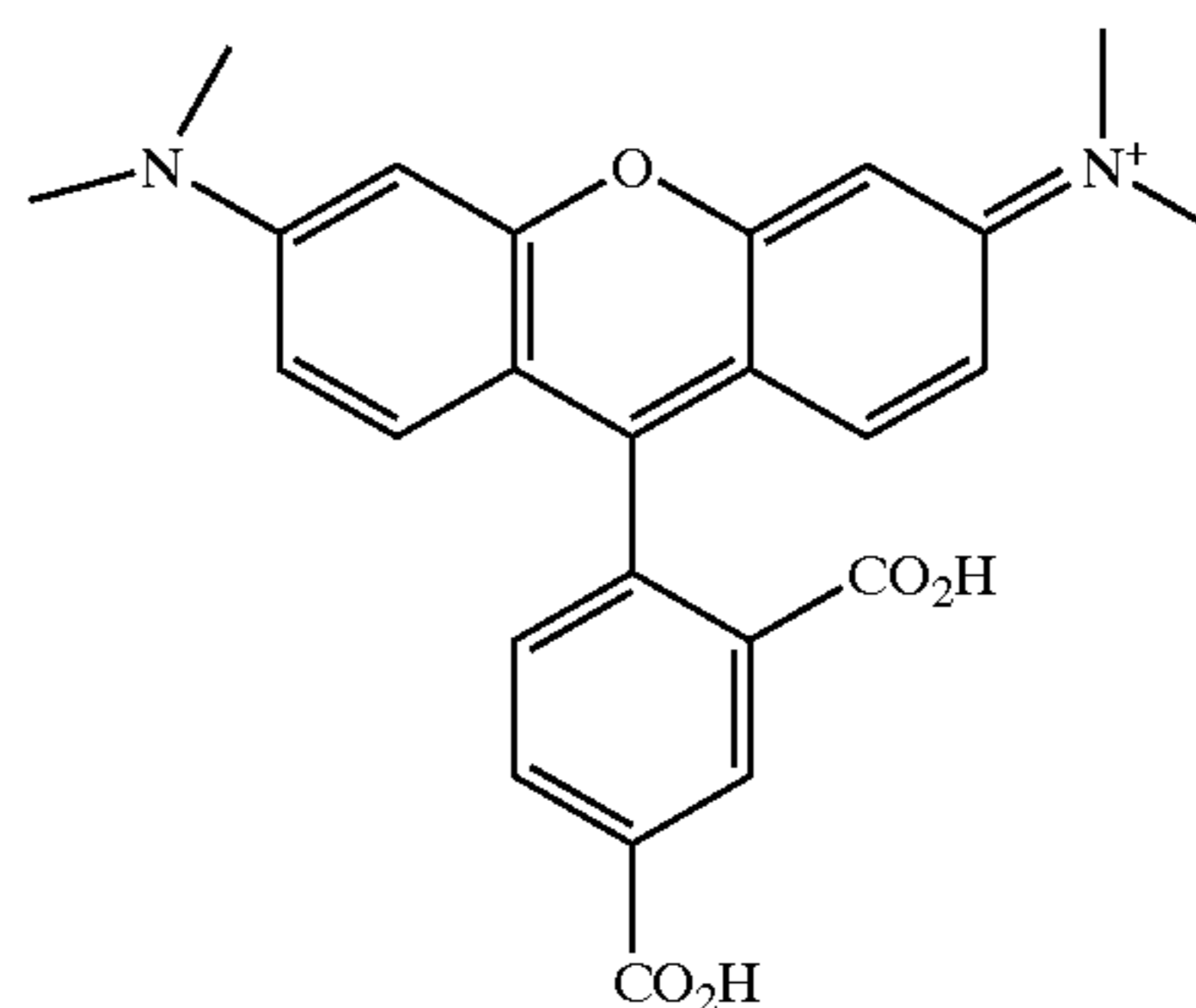
TAMRA
