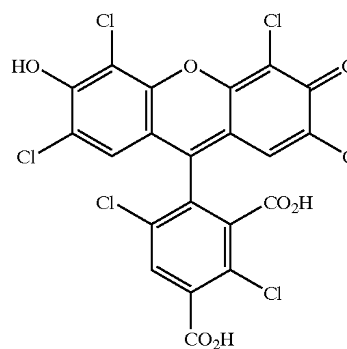
5-carboxy-HEX
