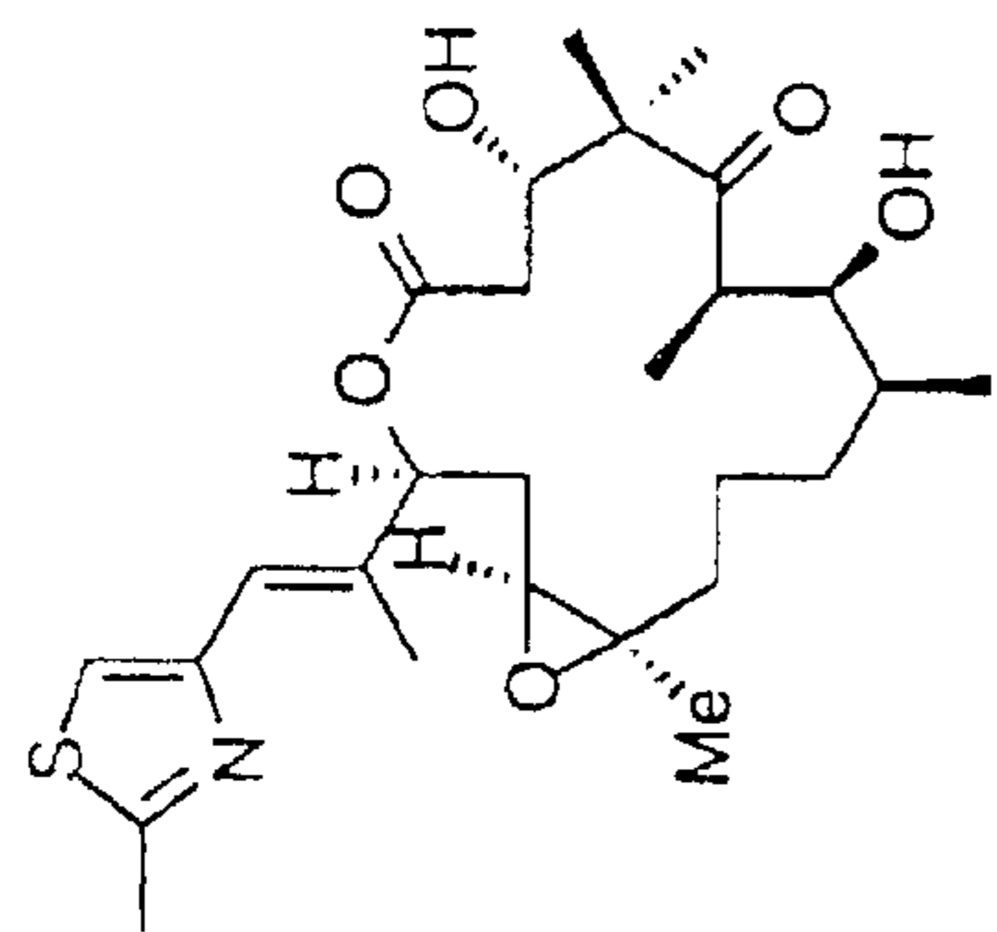
natural epothilone B
