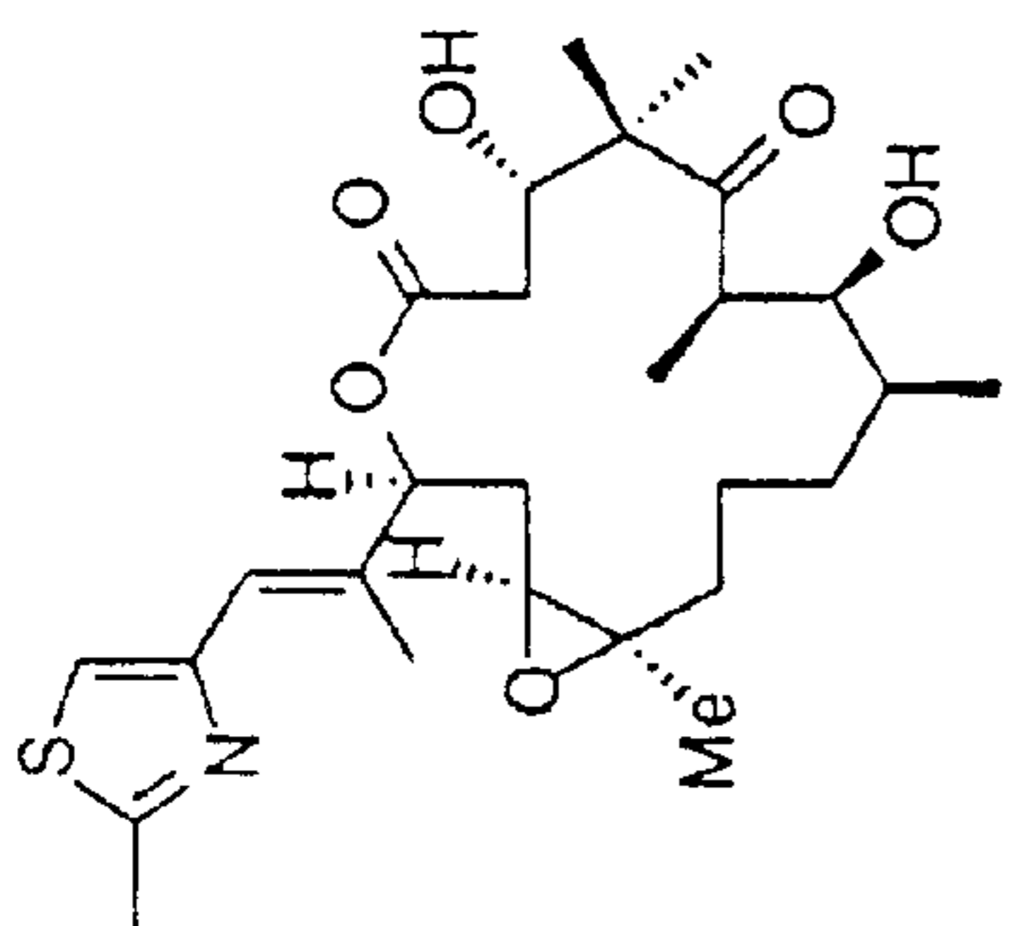
synthetic epothilone B
