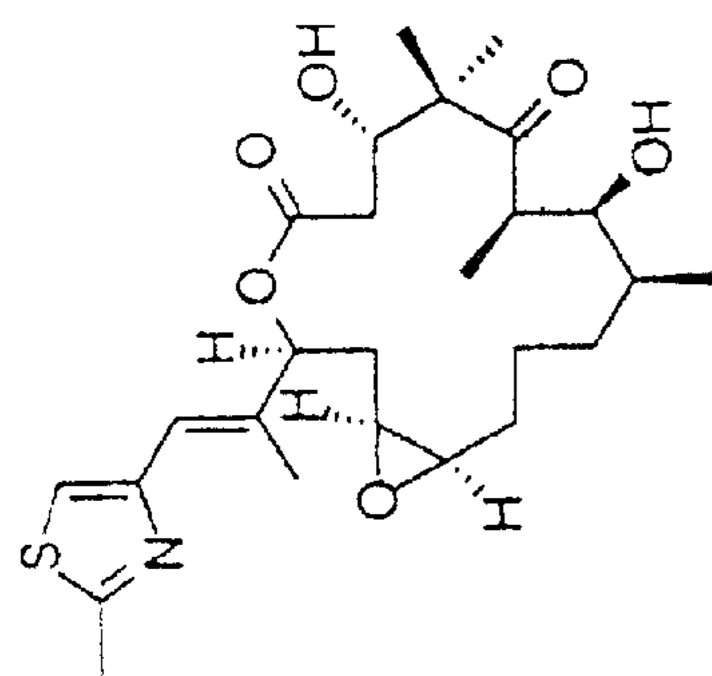
epothilone A
