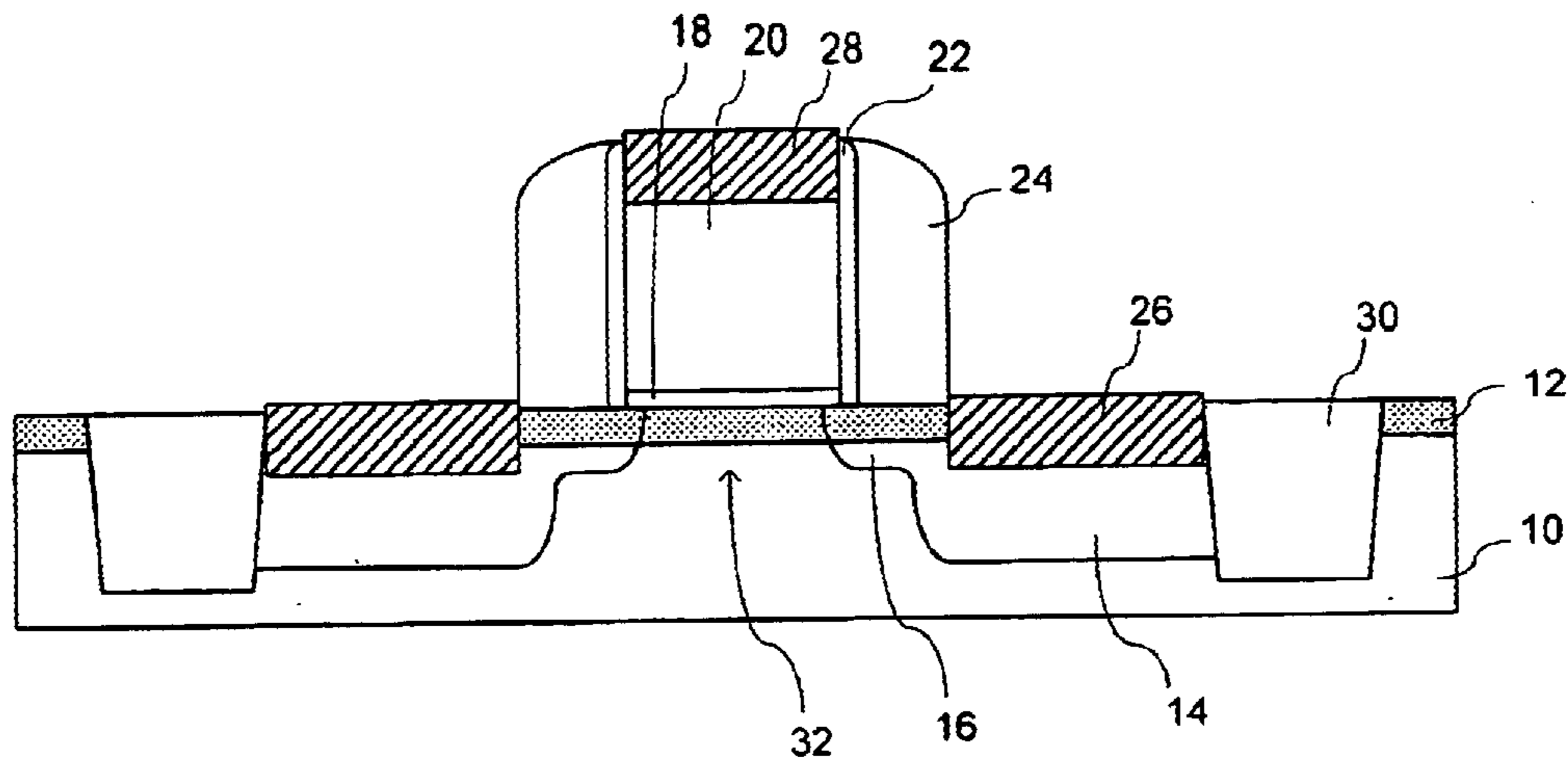
Figure 1 Prior Art
