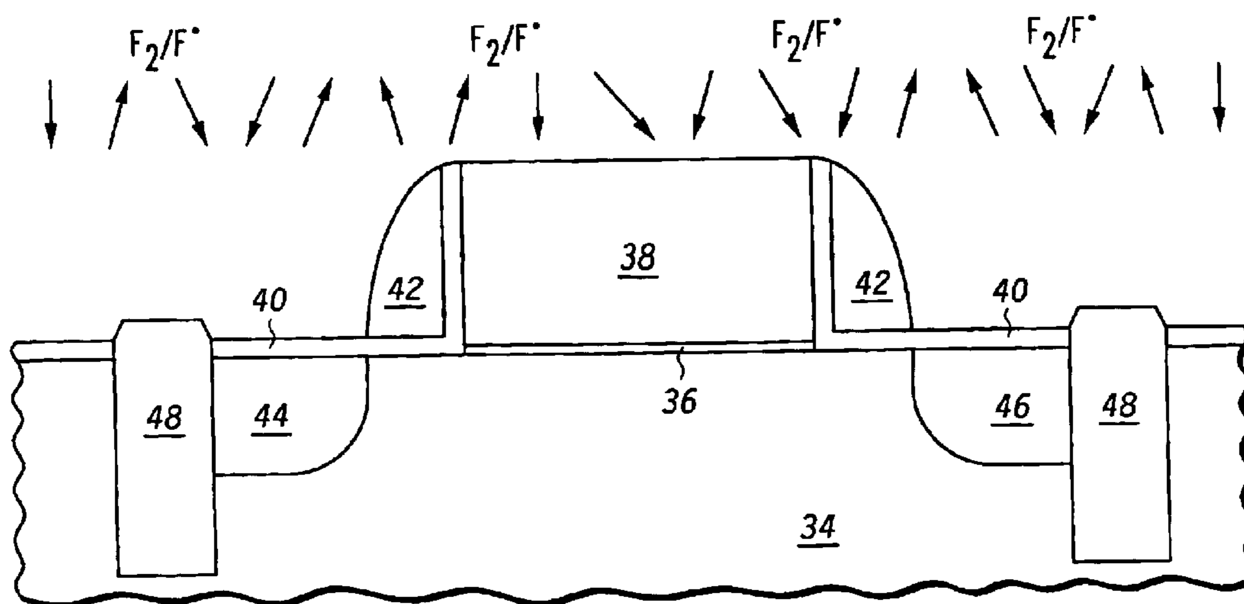
FIG. 2 -PRIOR ART-
