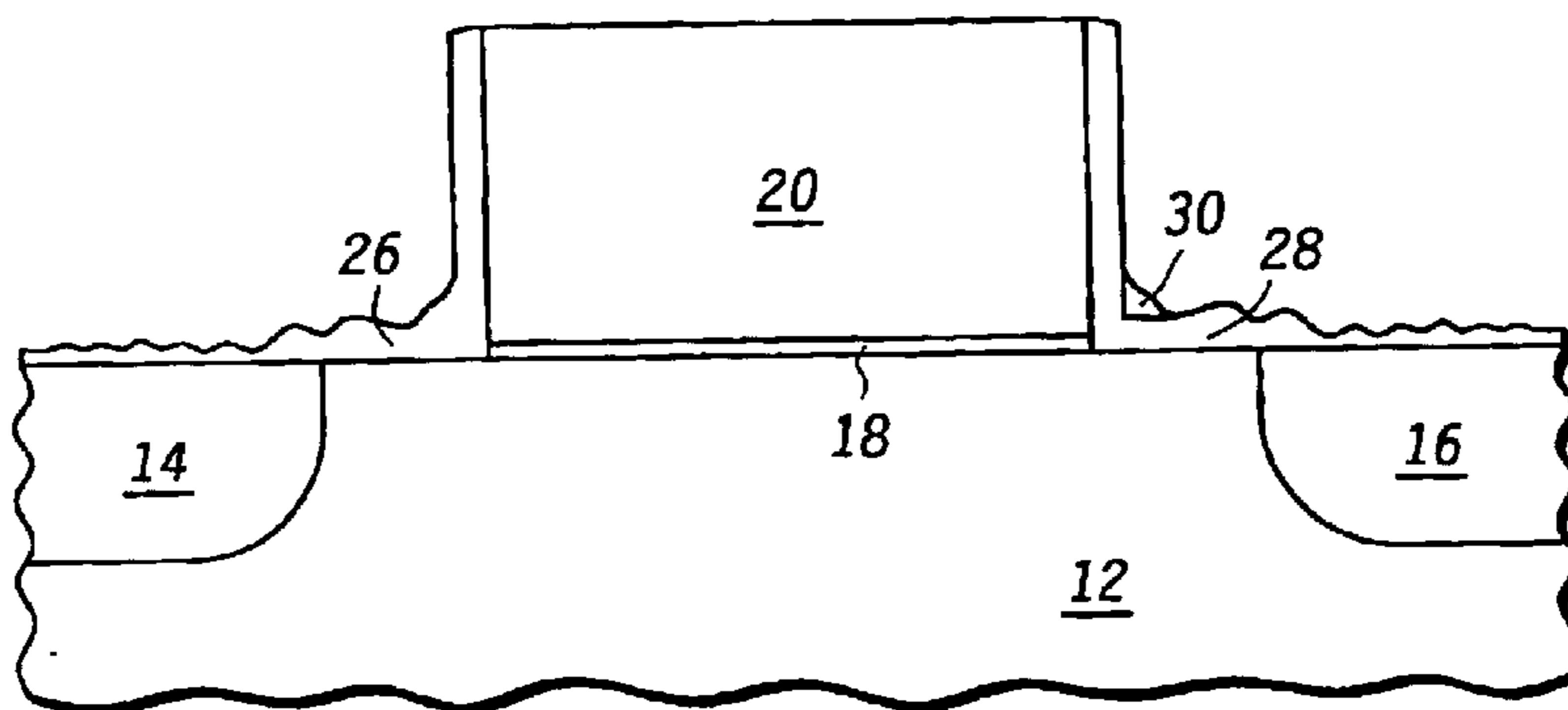
FIG. 2 -PRIOR ART-
