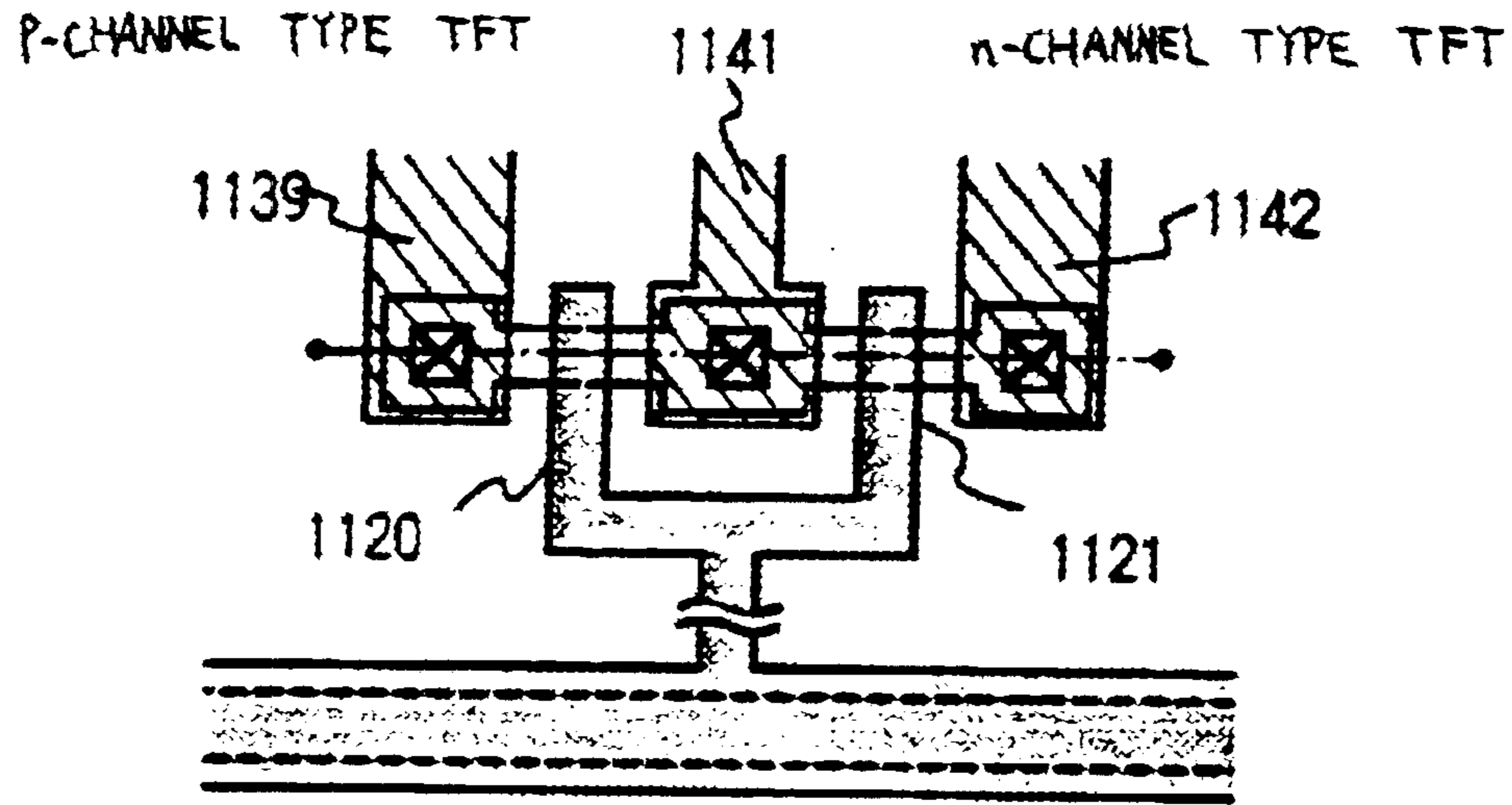
Fig. 10(A) TOP PLAN VIEW OF CMOS CIRCUIT
