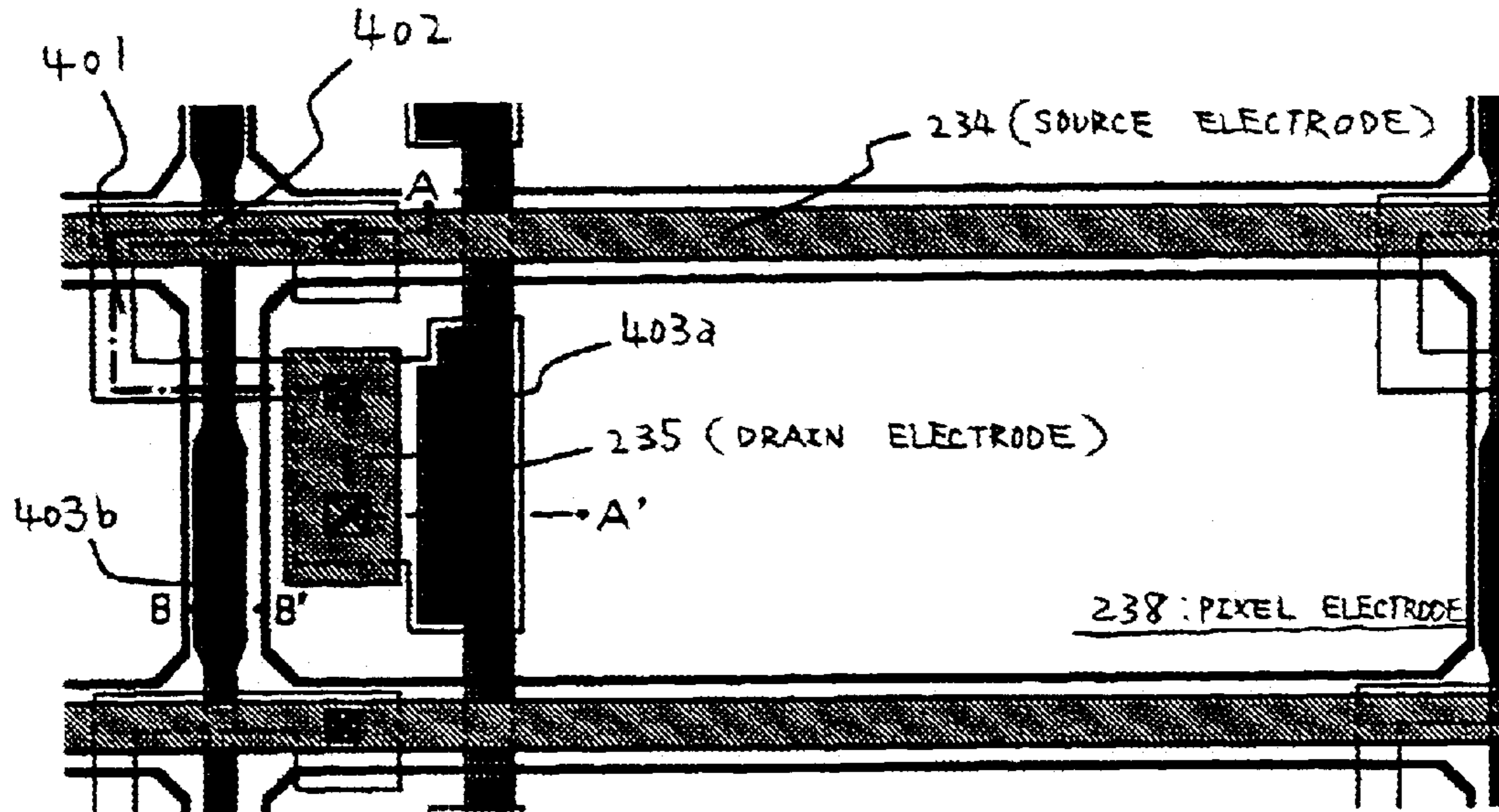
Fig. 5(B) TOP PLAN VIEW SHOWING PIXEL UNIT
