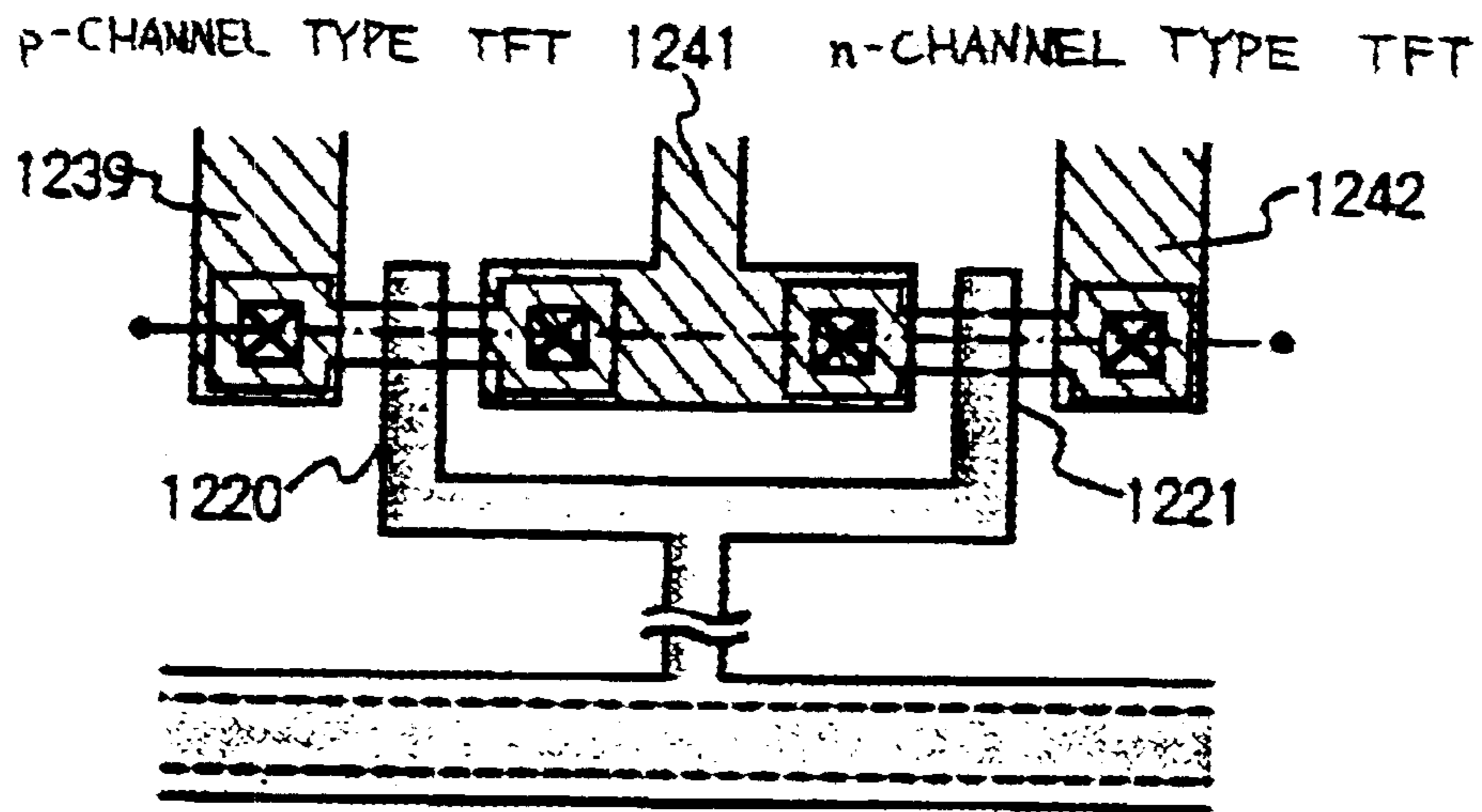
Fig. 10(B) TOP PLAN VIEW OF CMOS CIRCUIT
