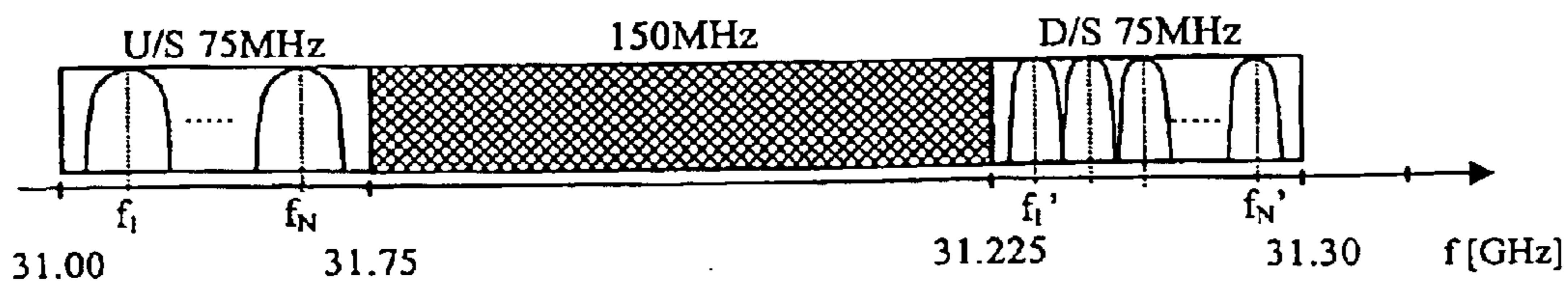
Figure 21. LMDS U.S. B-Band
