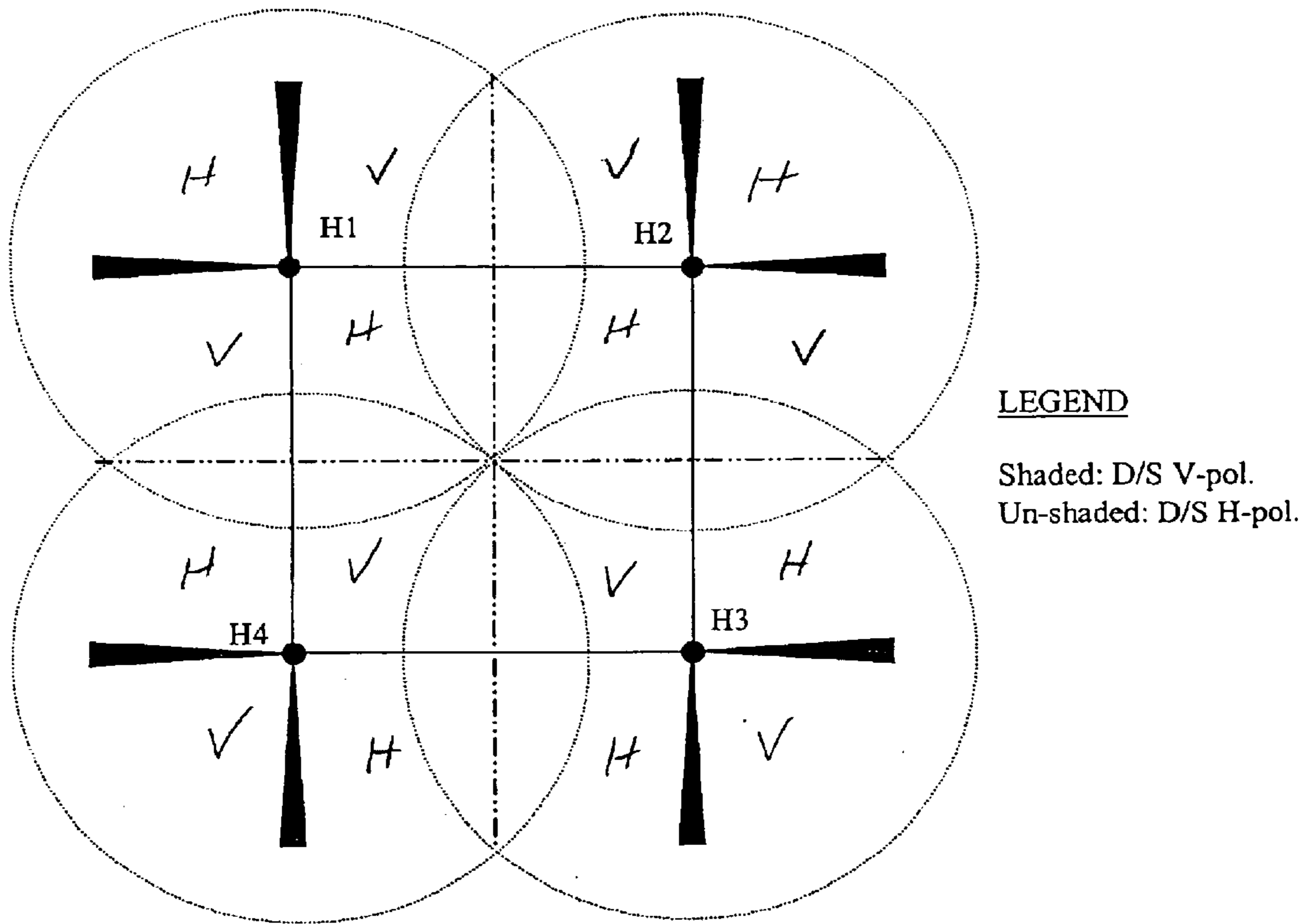
Figure 10. Straight 4 Hub D/S Interference (Polarization B)
