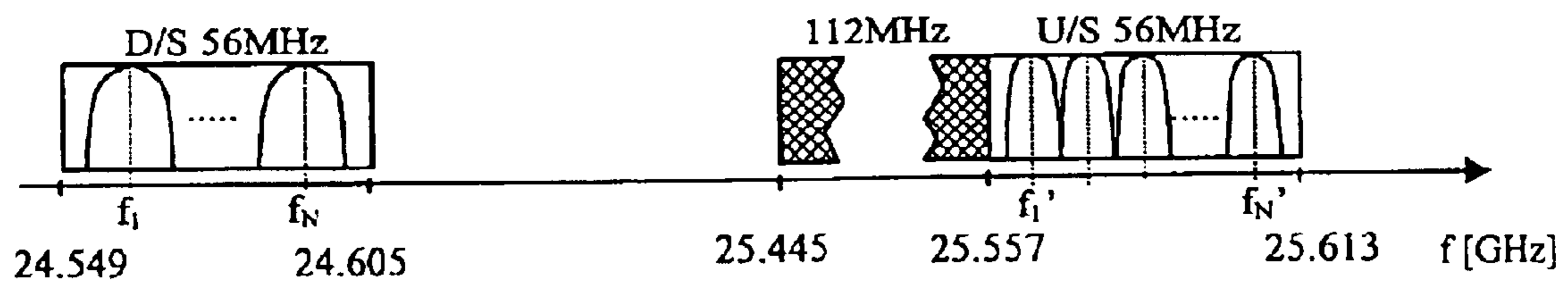
Figure 23. ETSI 26 GHz Spectrum (Detailed Example)
