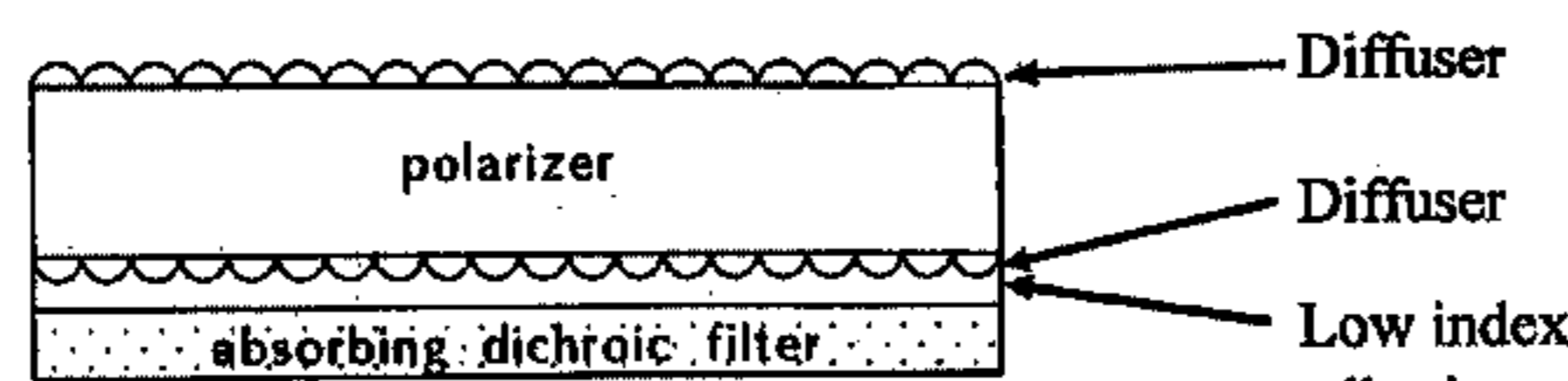
b. Front surface diffuser and immersed diffuser
