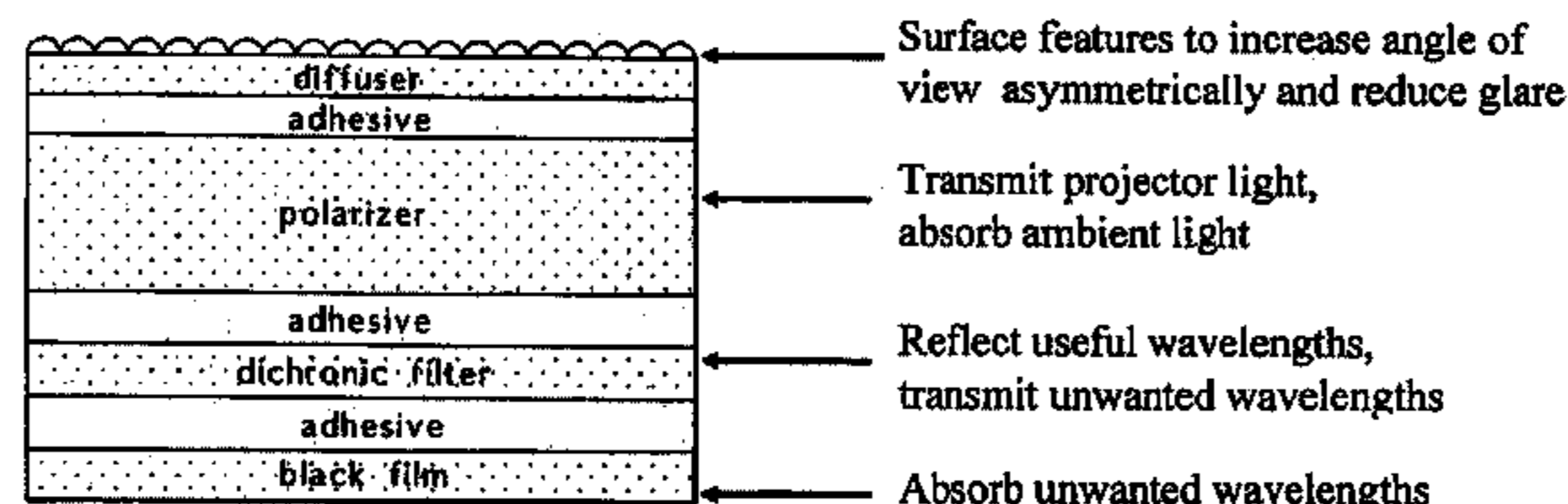
DRAWING 7 MINIMAL RISK CONSTRUCTION 3/15/01, B.L.
