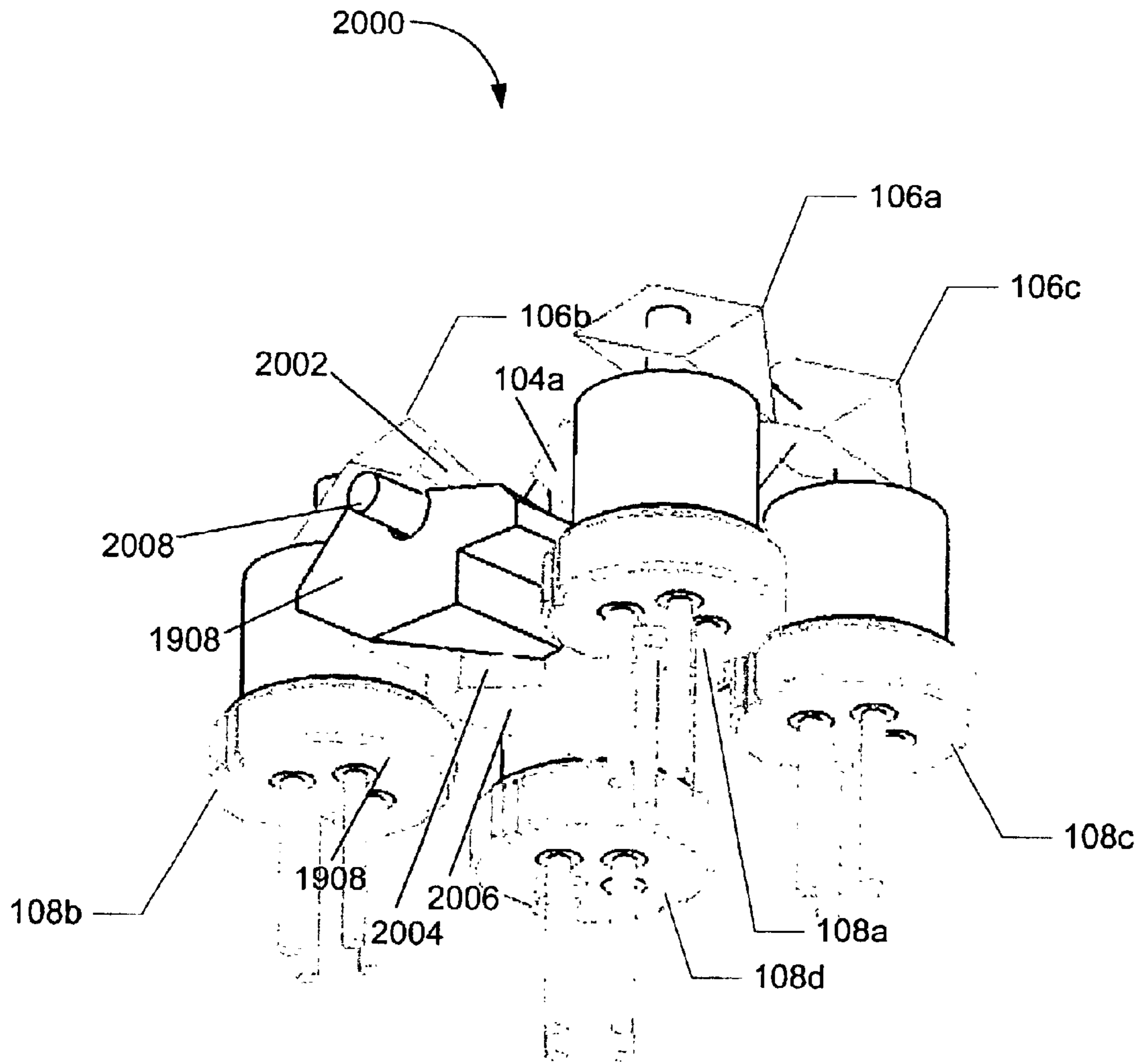
BOTTOM ISOMETRIC VIEW
