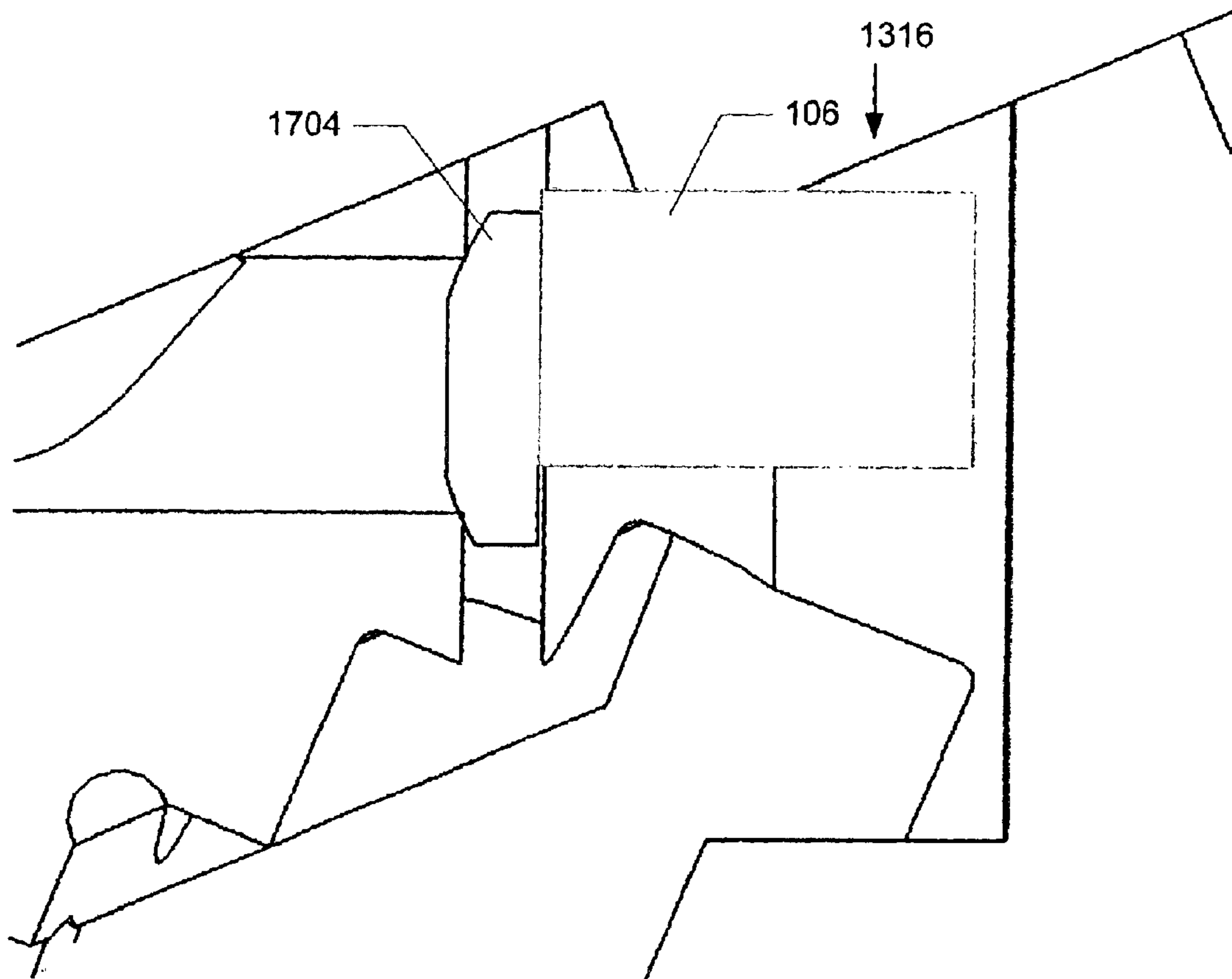
SIDE CROSS-SECTIONAL VIEW
