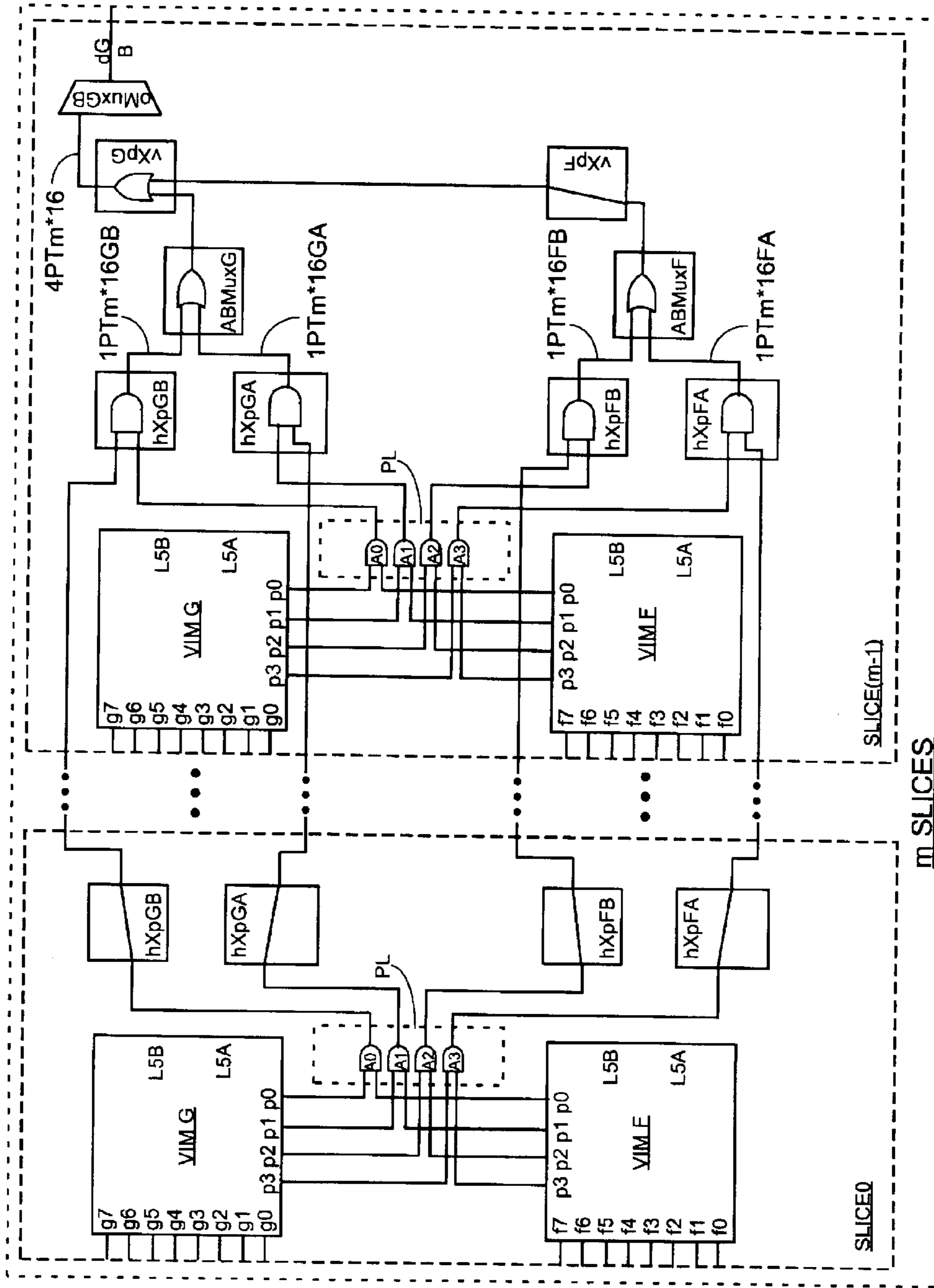
(1 PAL of 4 Pterms with m*16 inputs) FIG. 9
