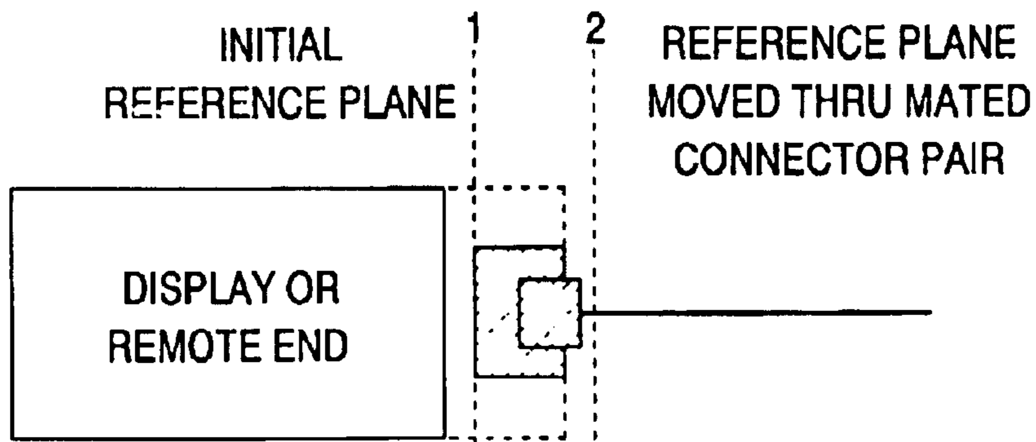
Fig. 14 [S_{21}] CONNECTOR PAIR
