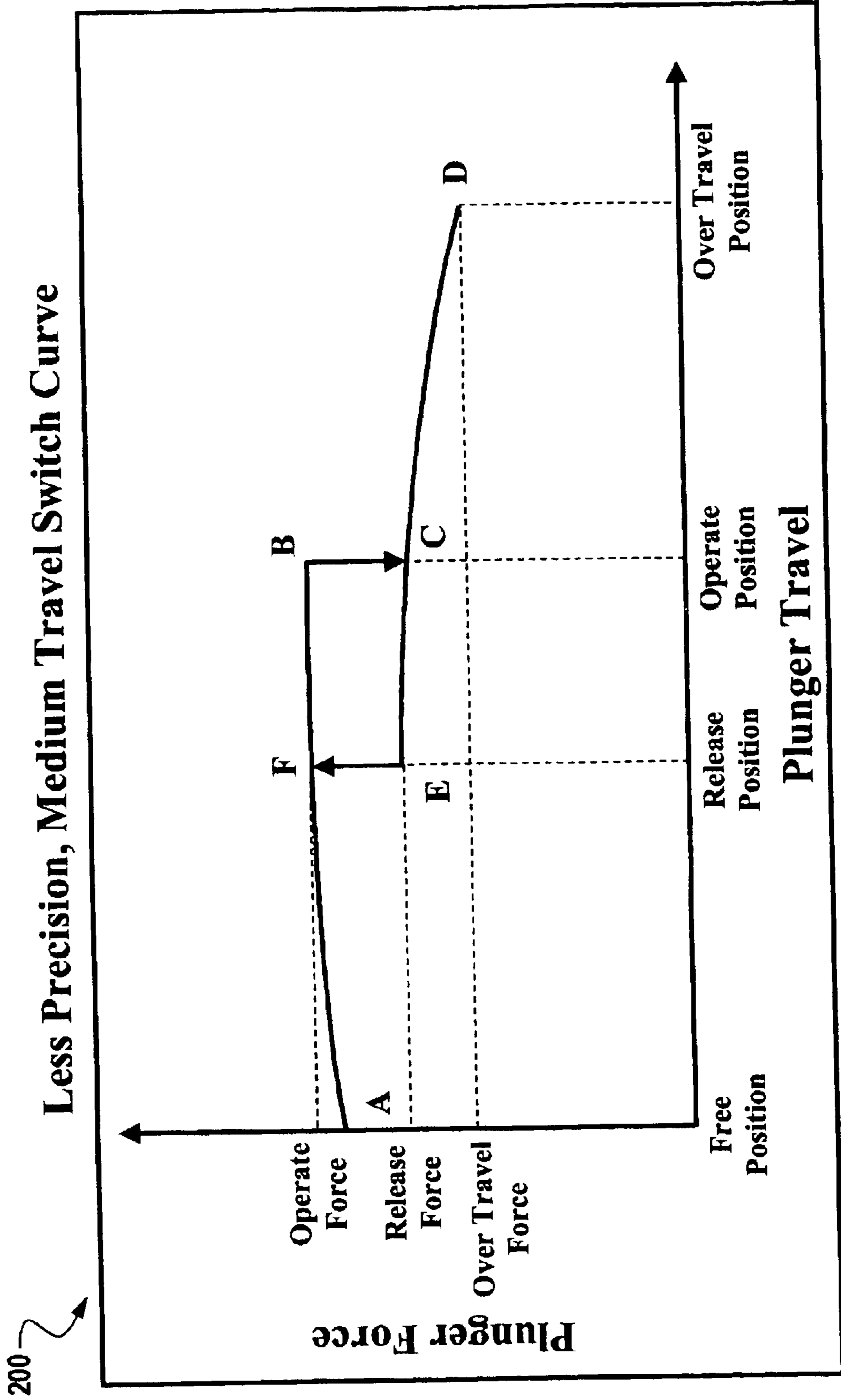
Fig. 2 (Prior Art)
