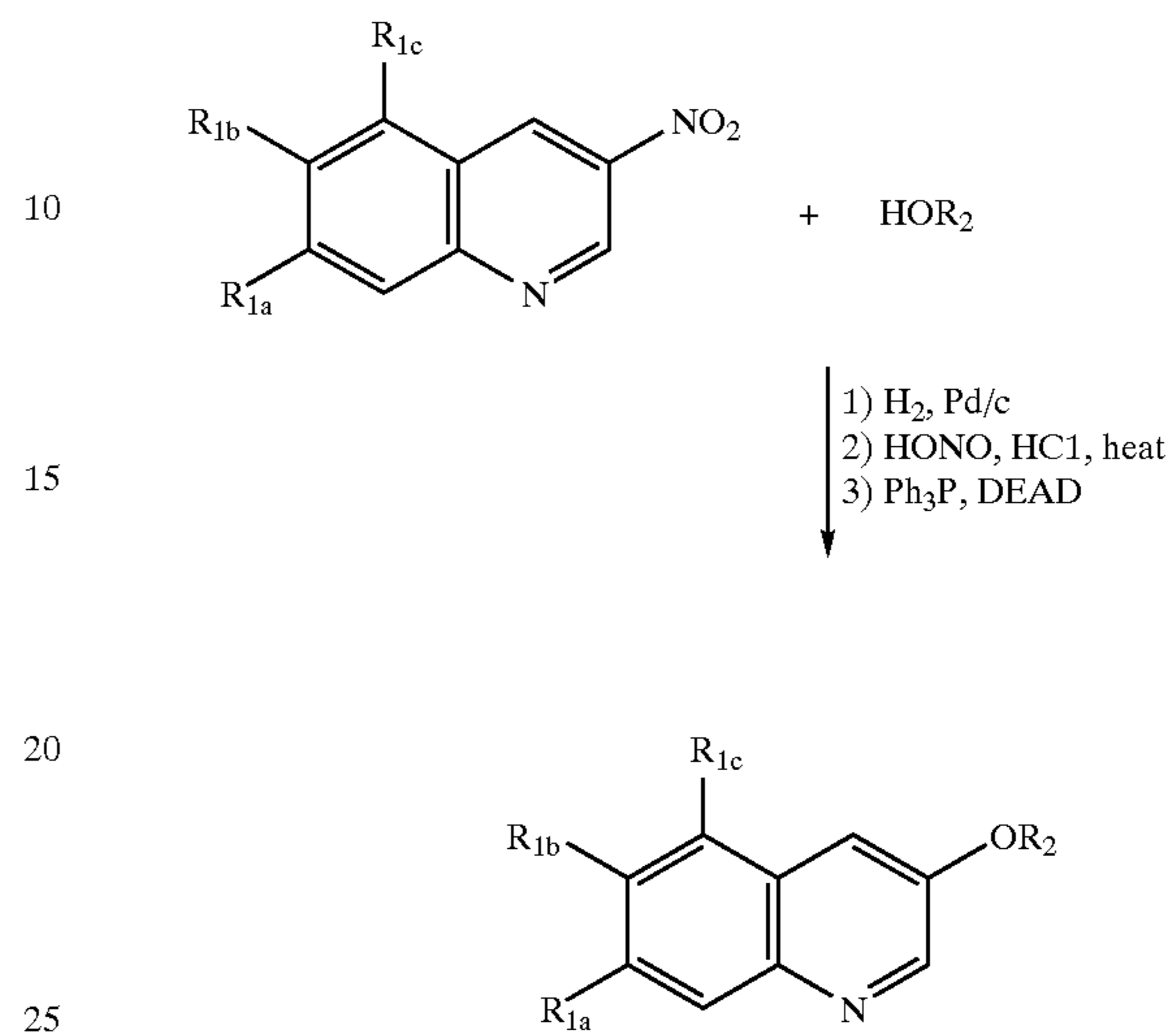
Scheme V
