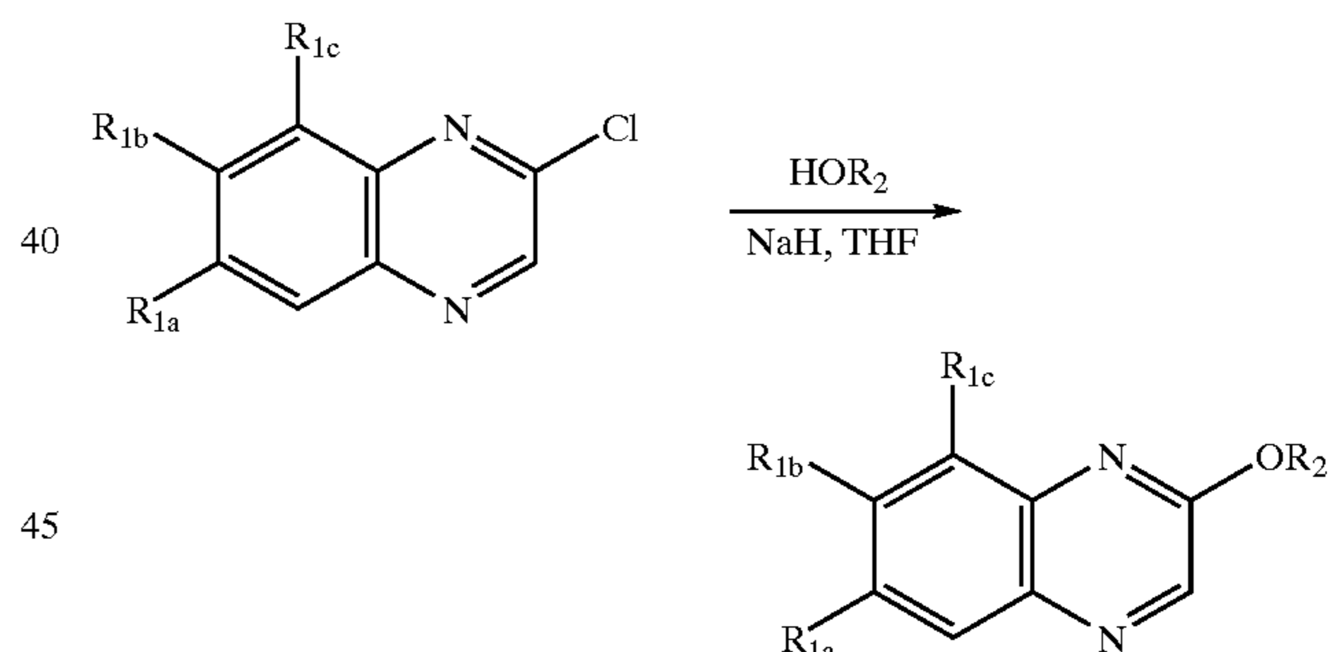
Scheme III
