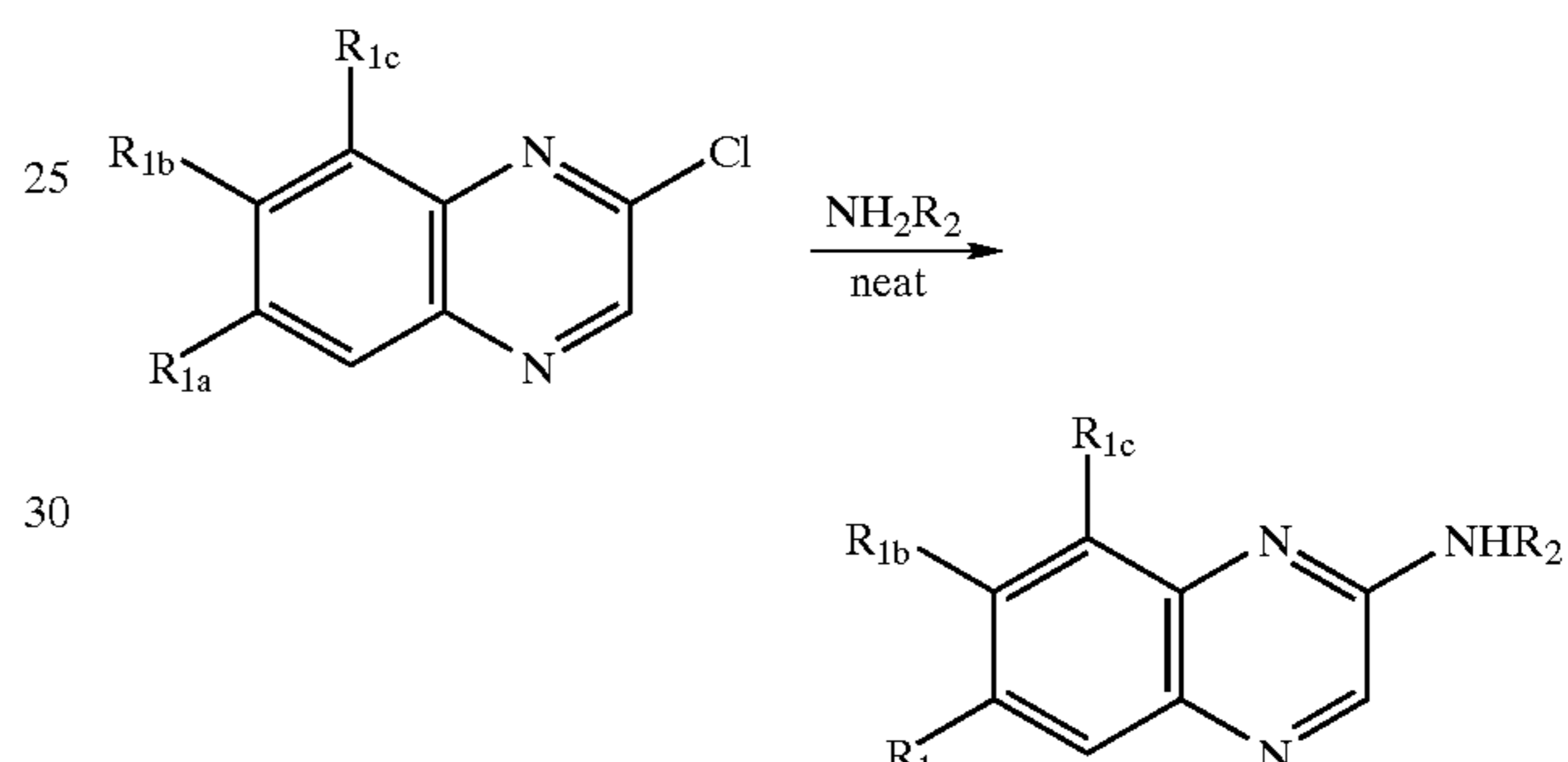
Scheme II
