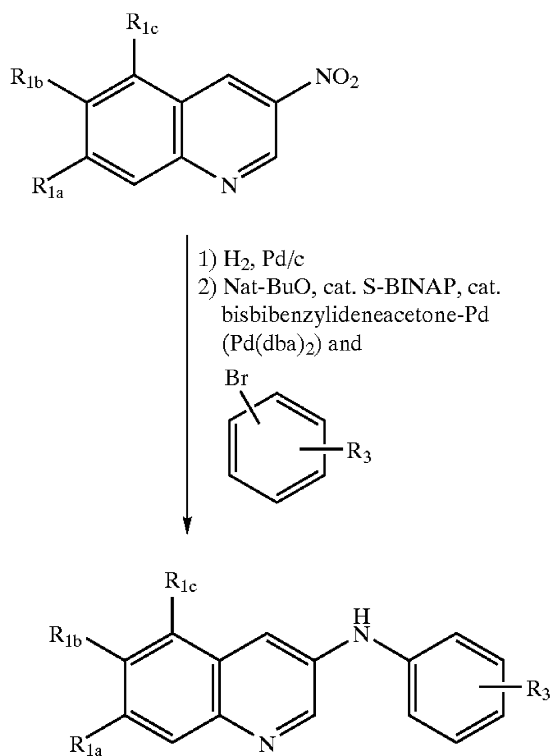
Scheme IV
