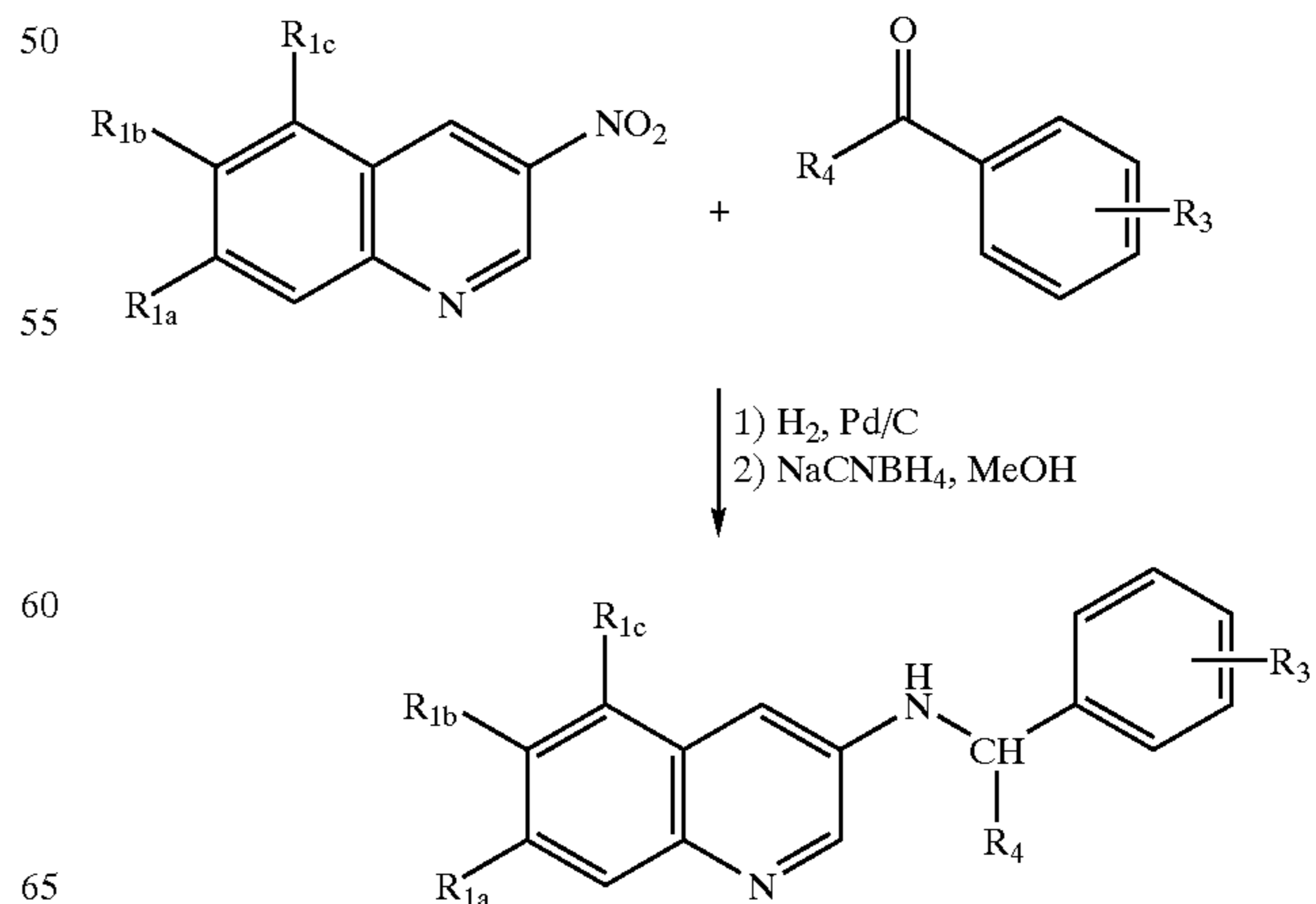
Scheme III
