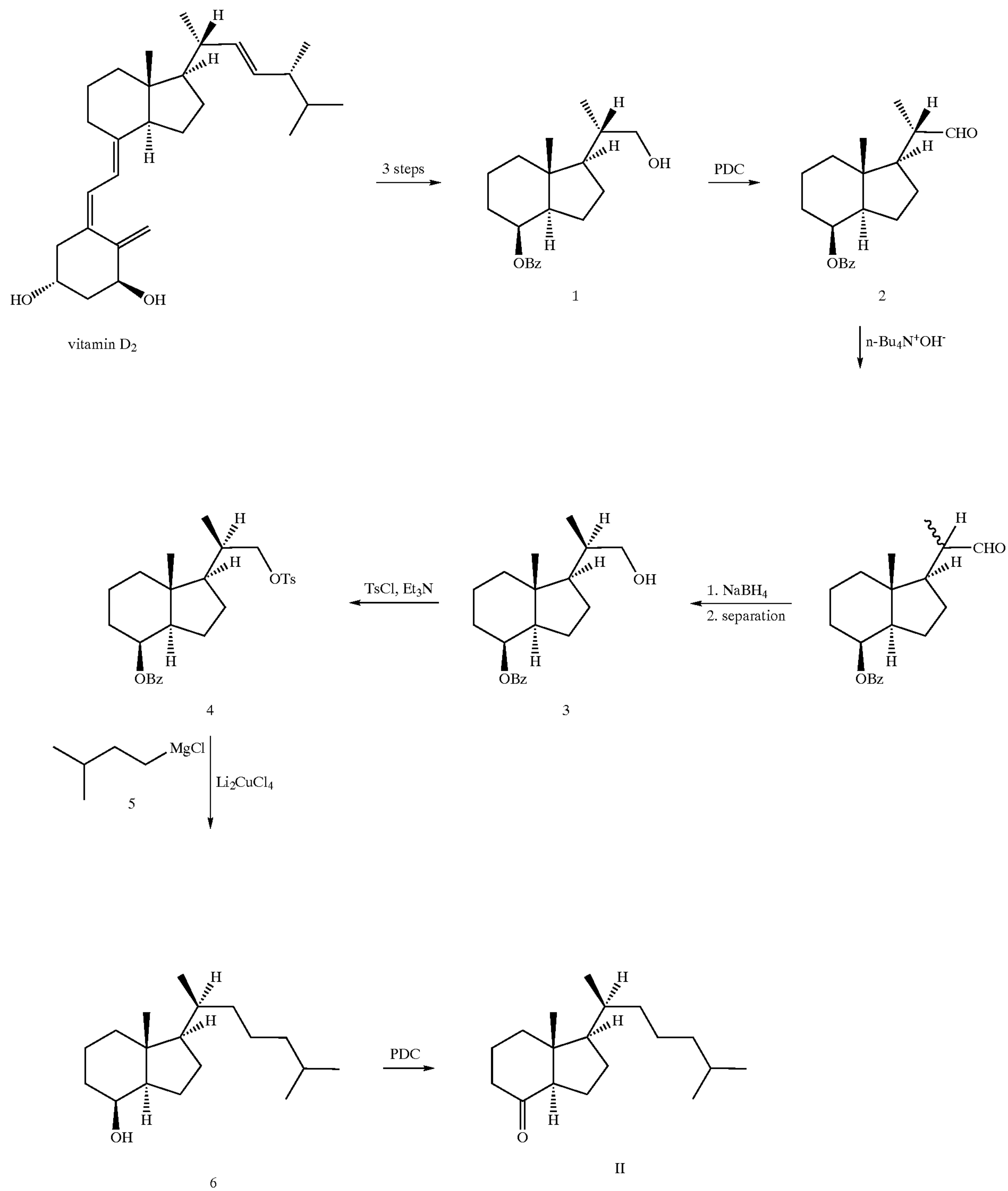
Scheme 1
