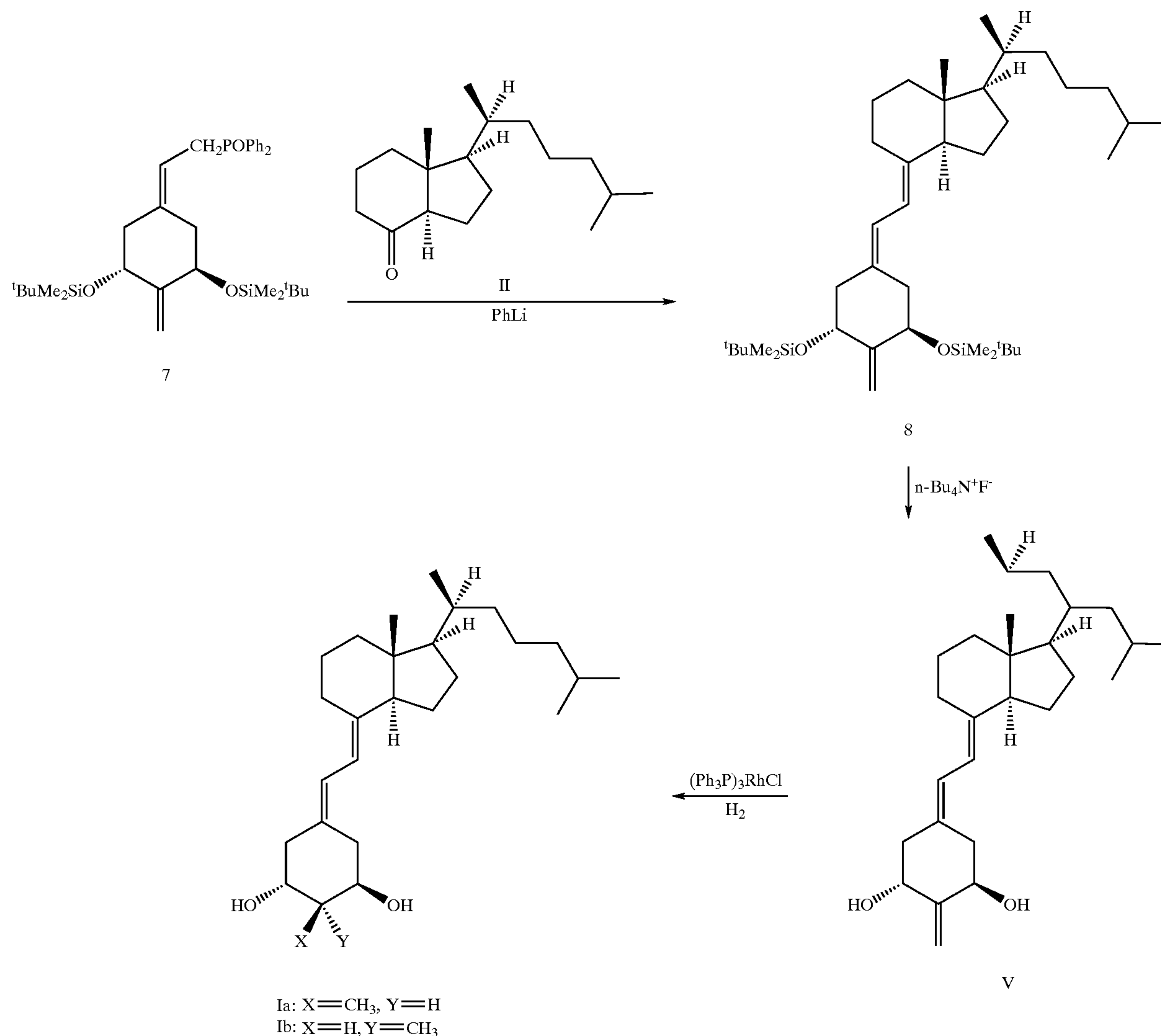
Scheme 2
