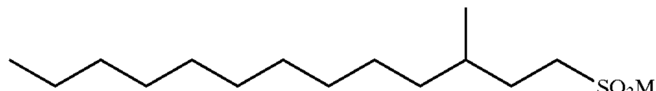
8-Methyltridecyl sulfate:
