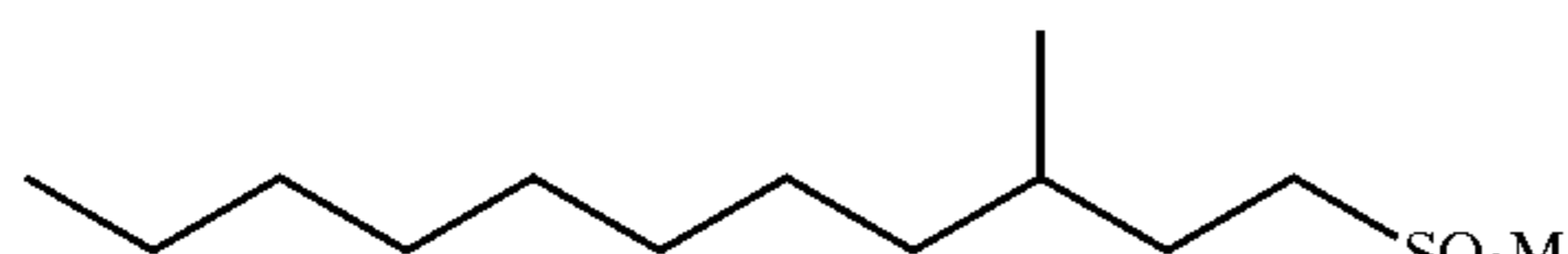
3-Methyltridecyl sulfate:
