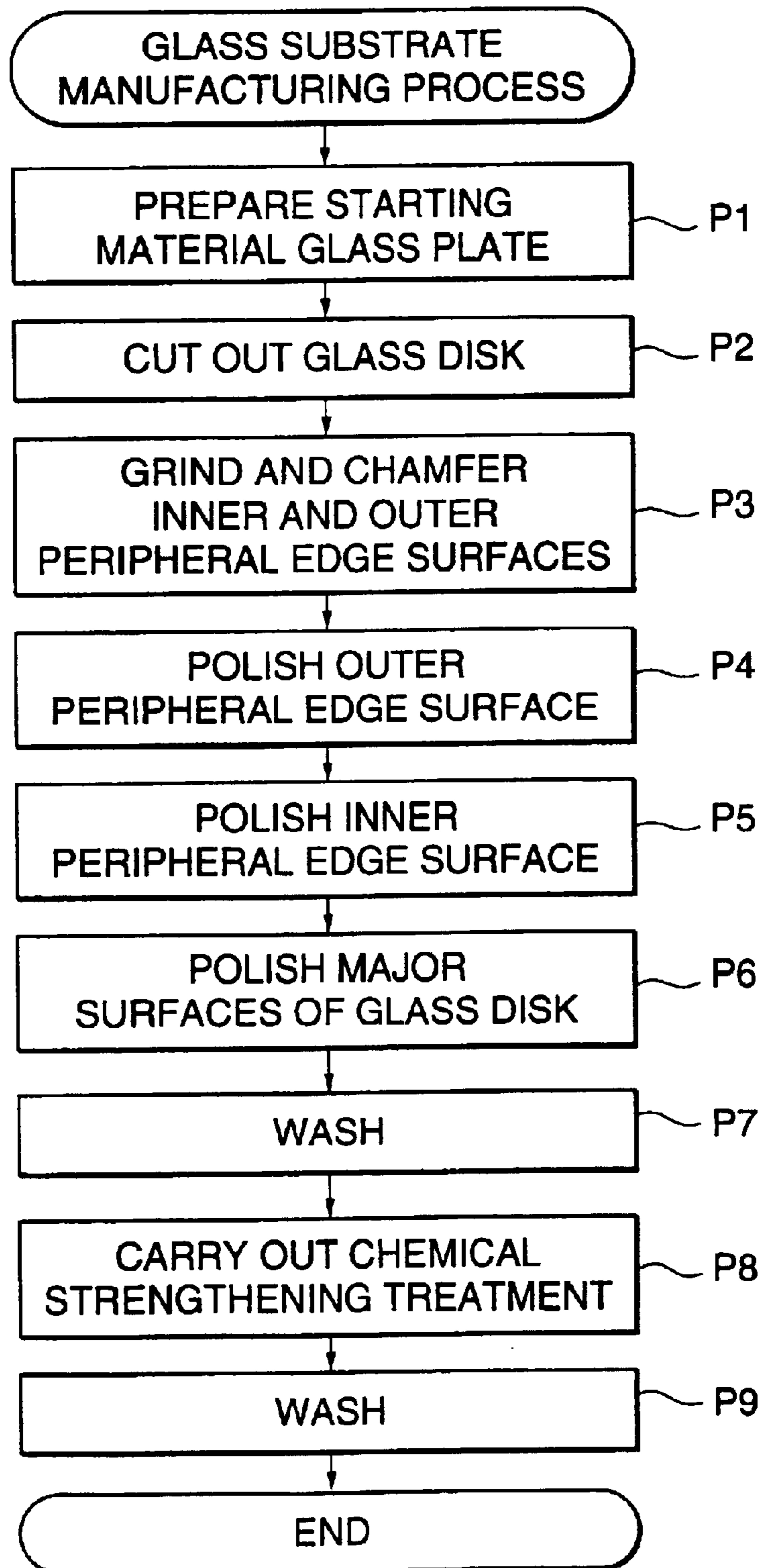
FIG. 9 PRIOR ART
