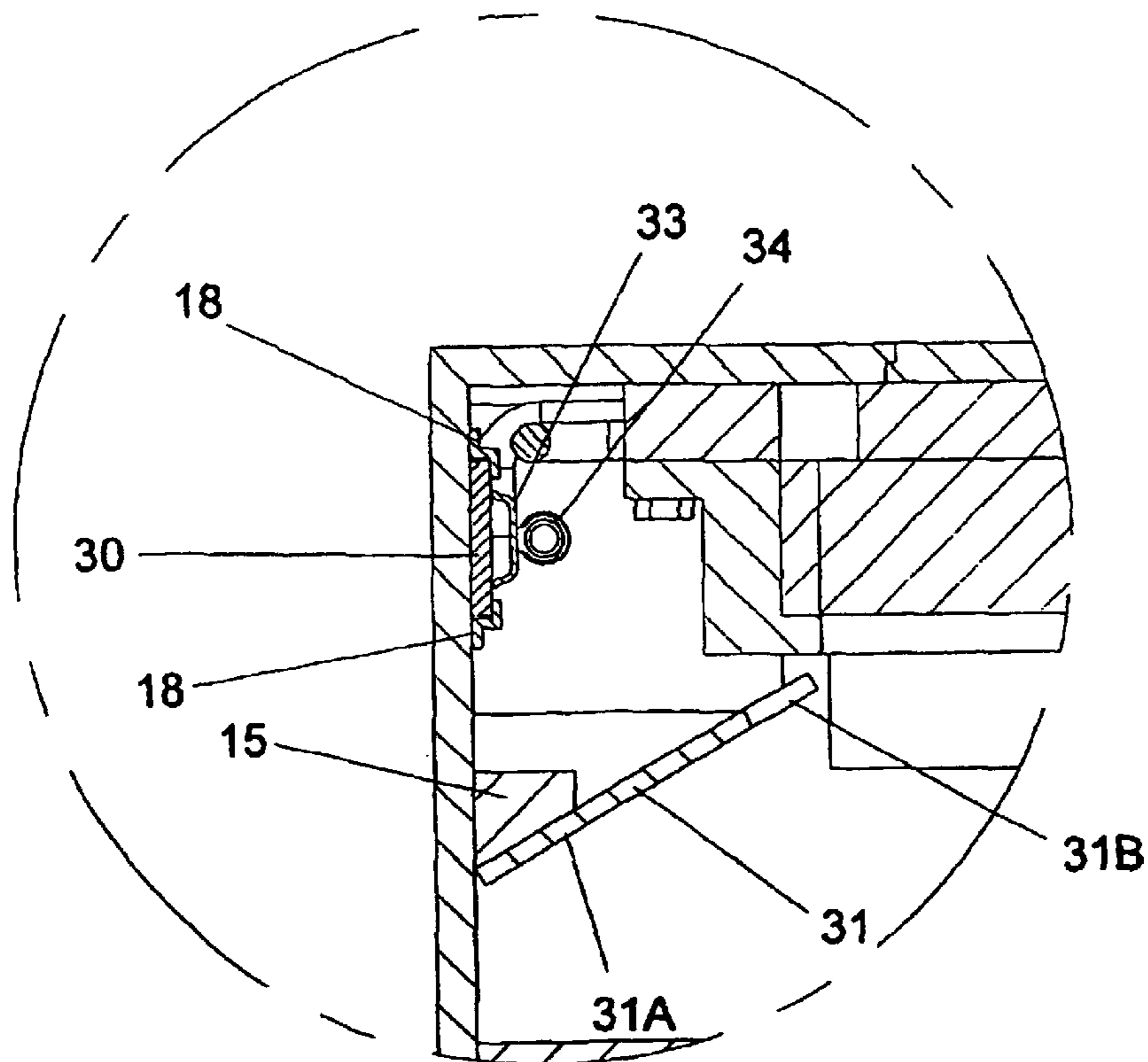
DETAIL "A"
