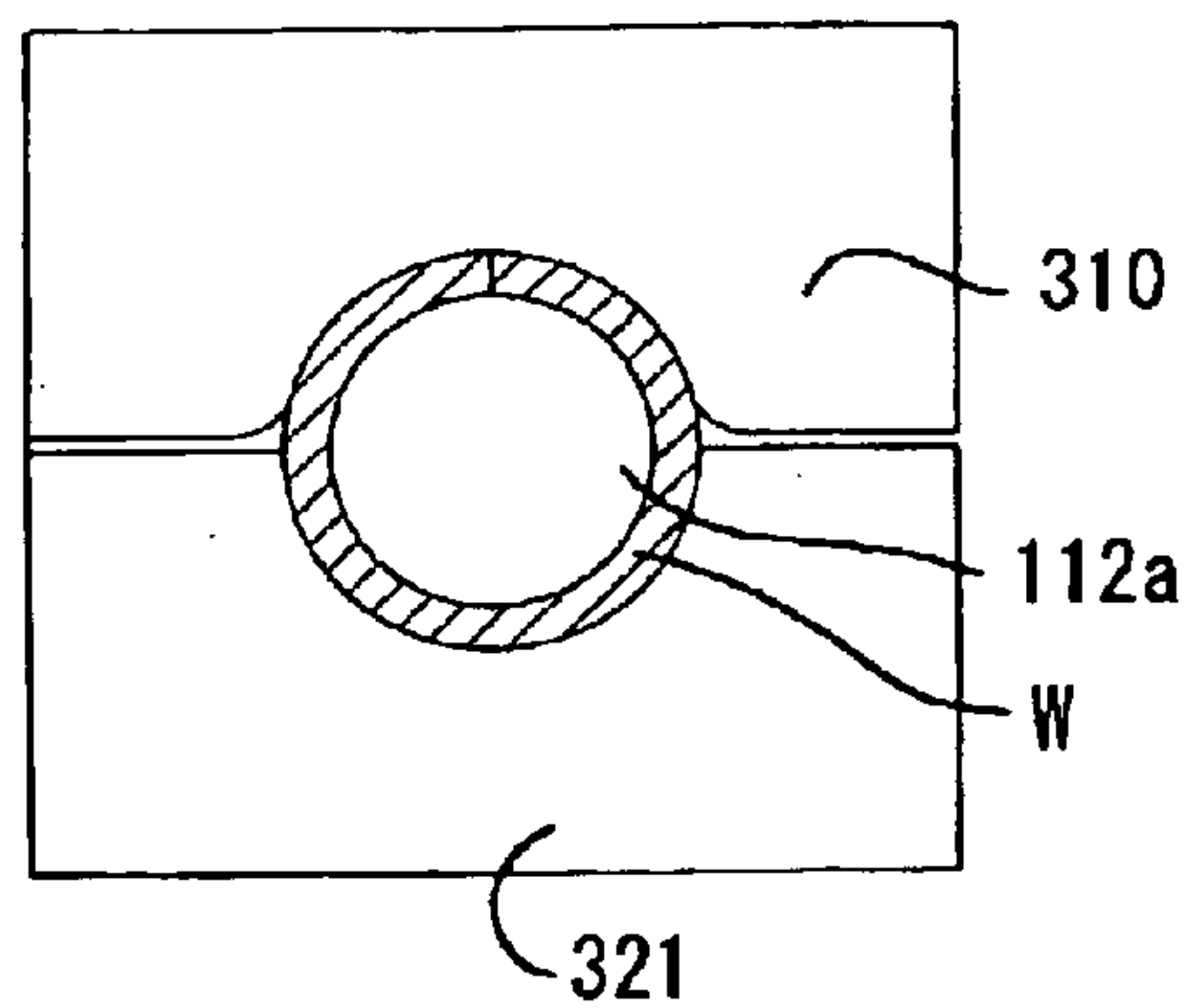
Fig.22c
