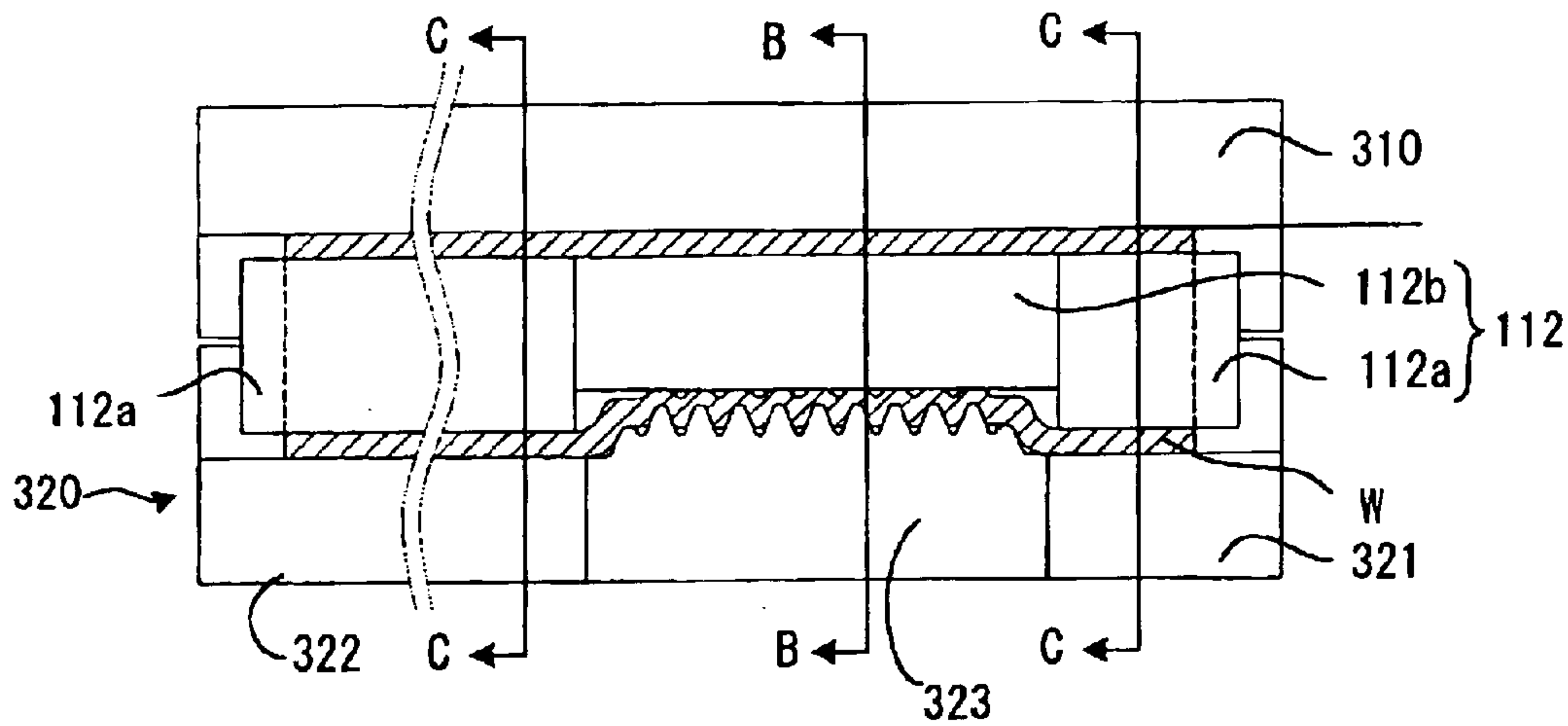
Fig.22c
