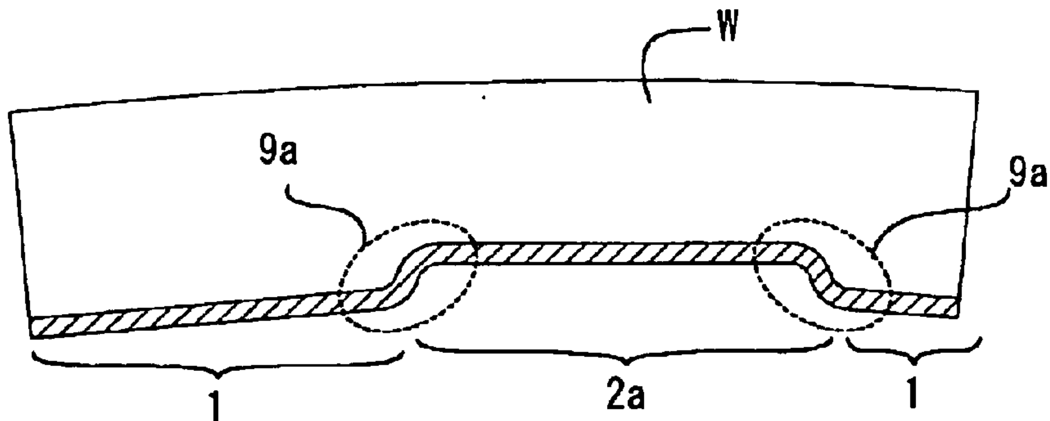
Fig. 2 PRIOR ART
