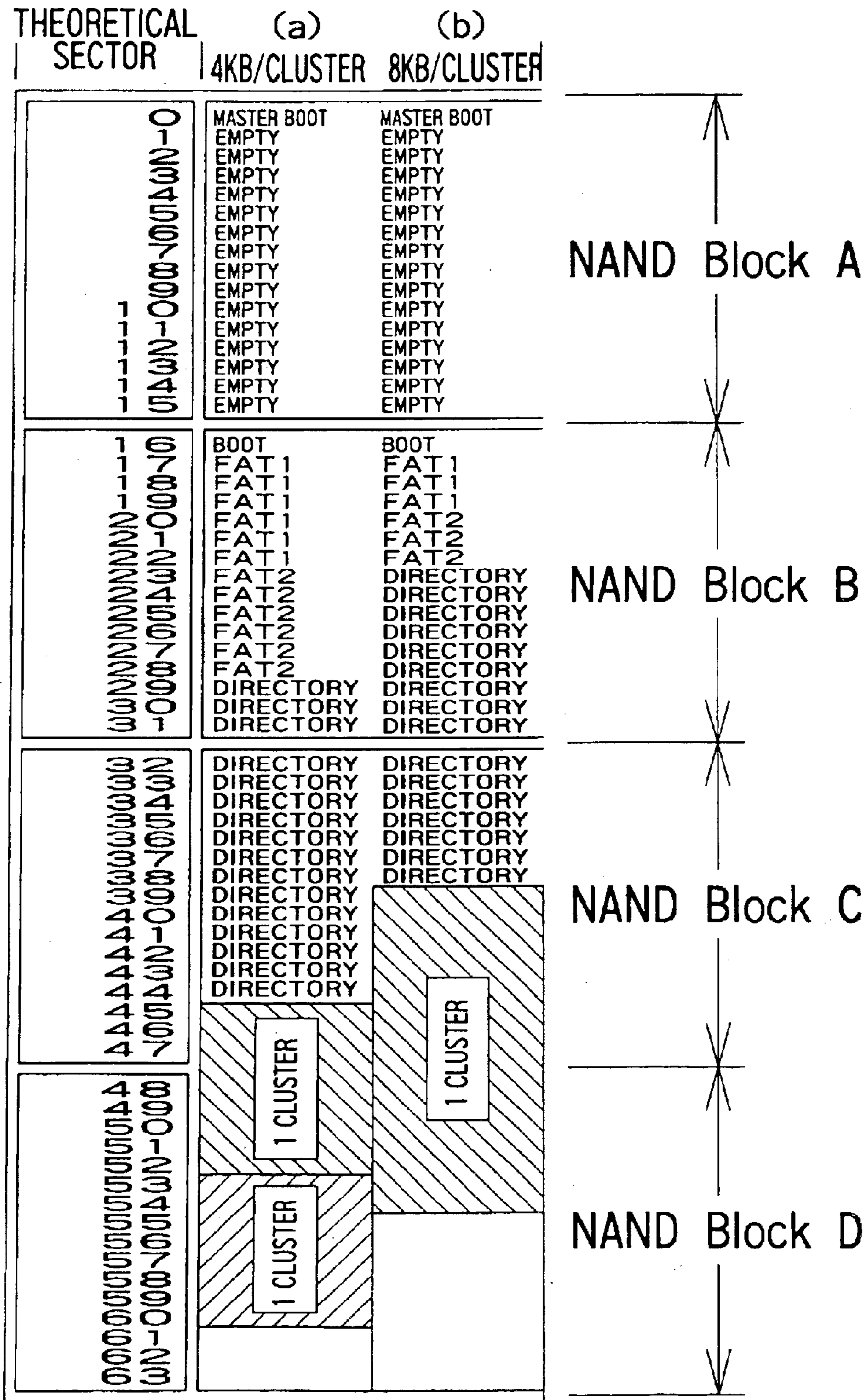
FIG. 12 PRIOR ART
