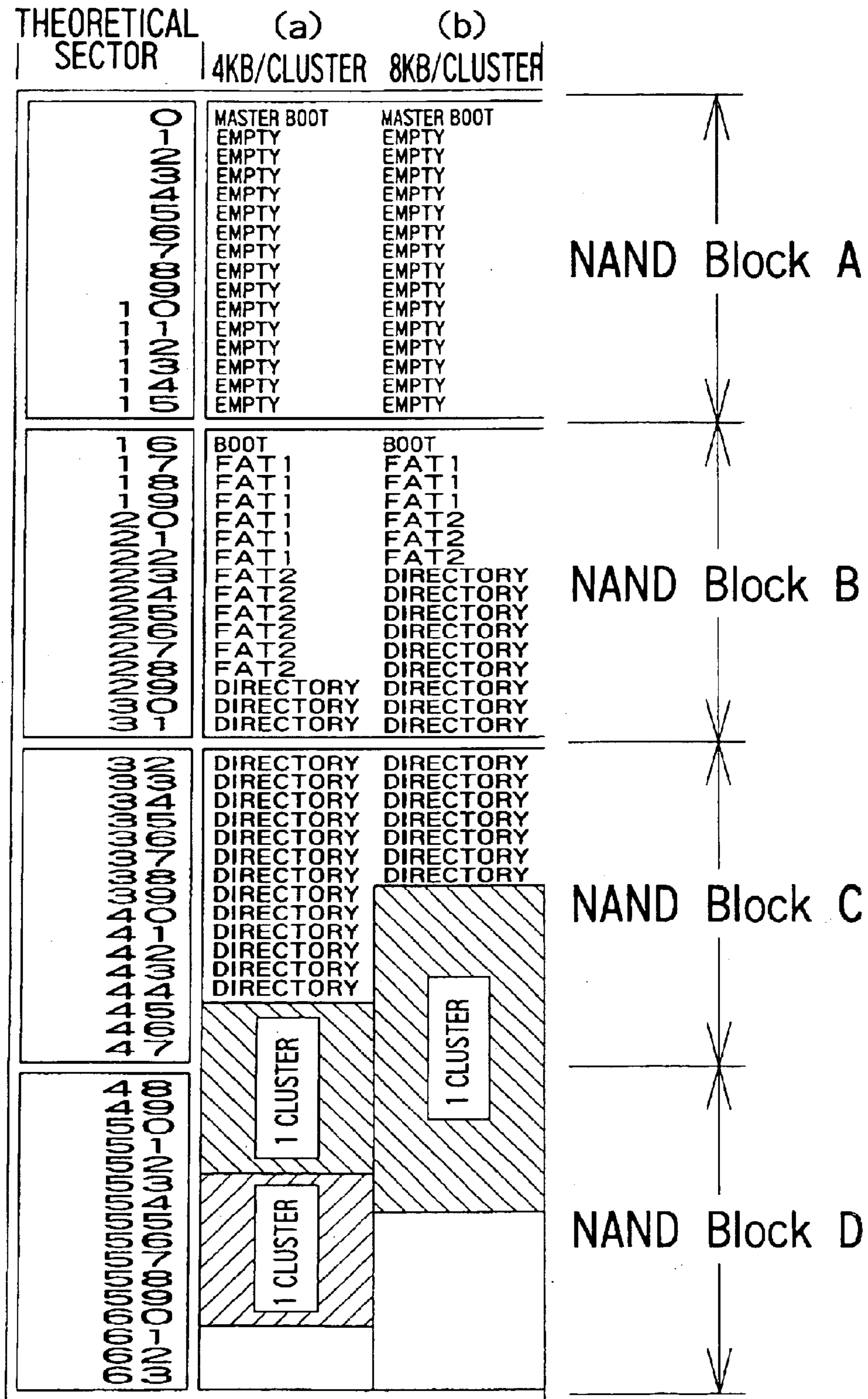
FIG. 12 PRIOR ART
