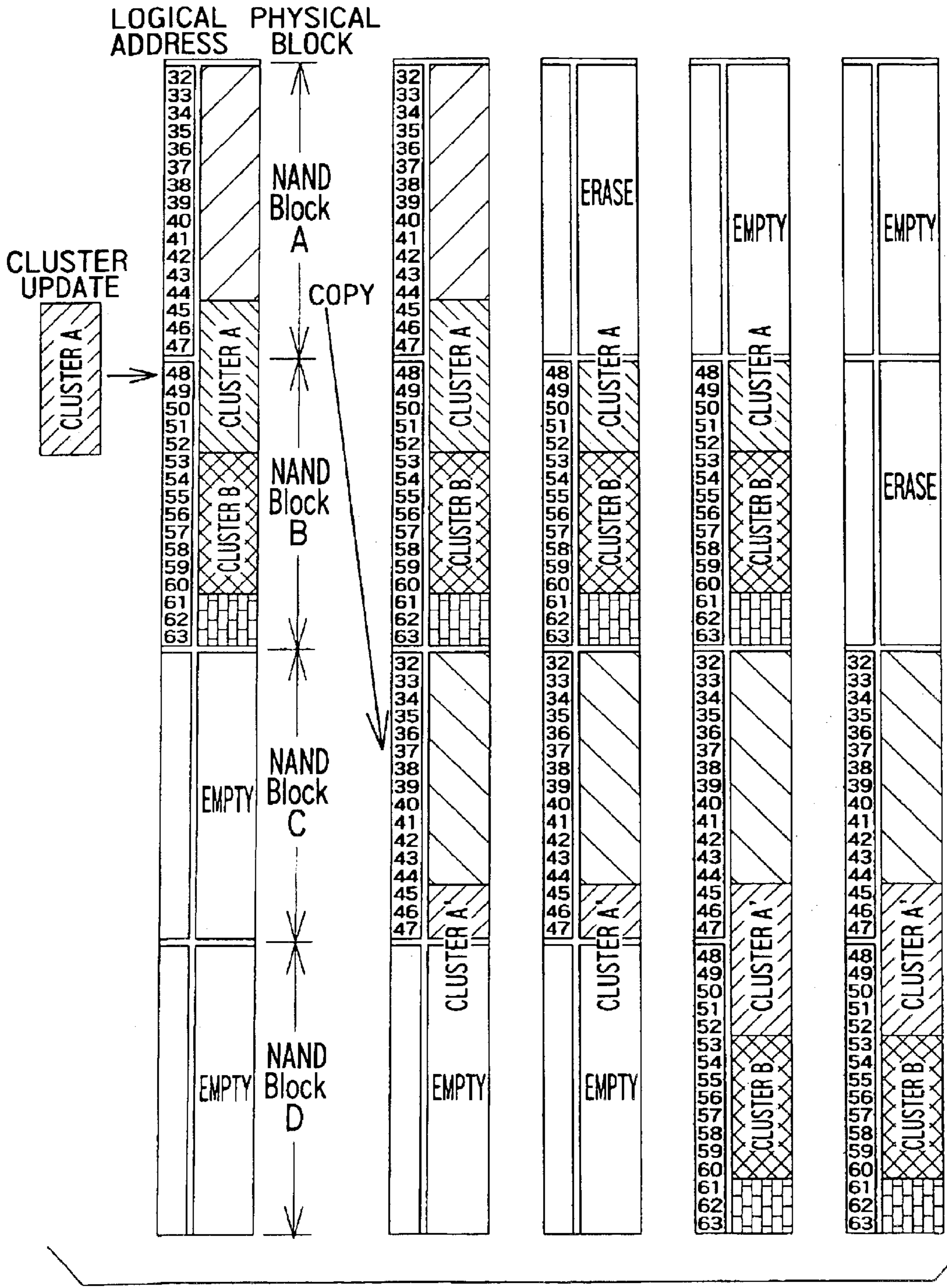
FIG. 13 PRIOR ART
