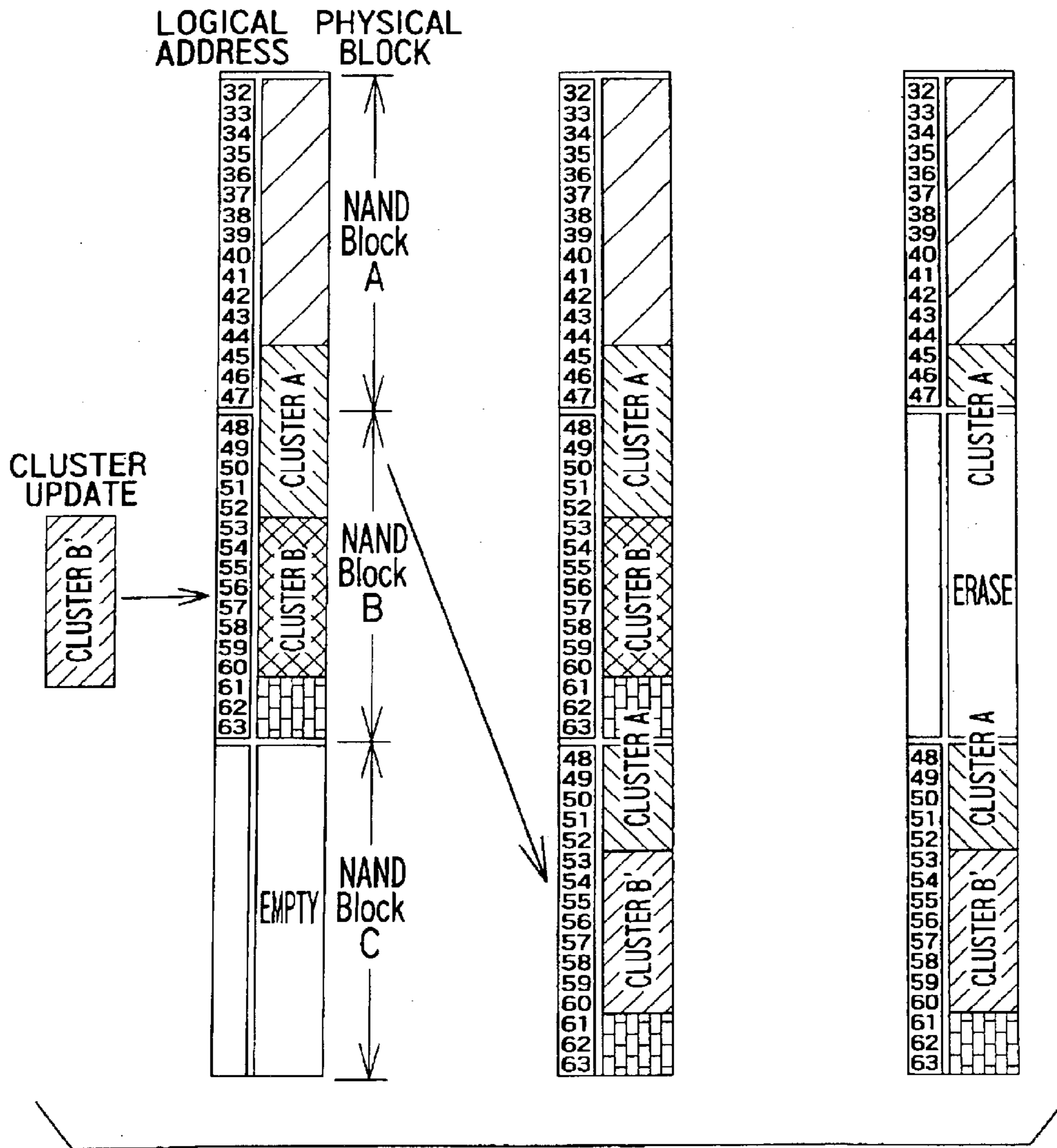
FIG. 14 PRIOR ART
