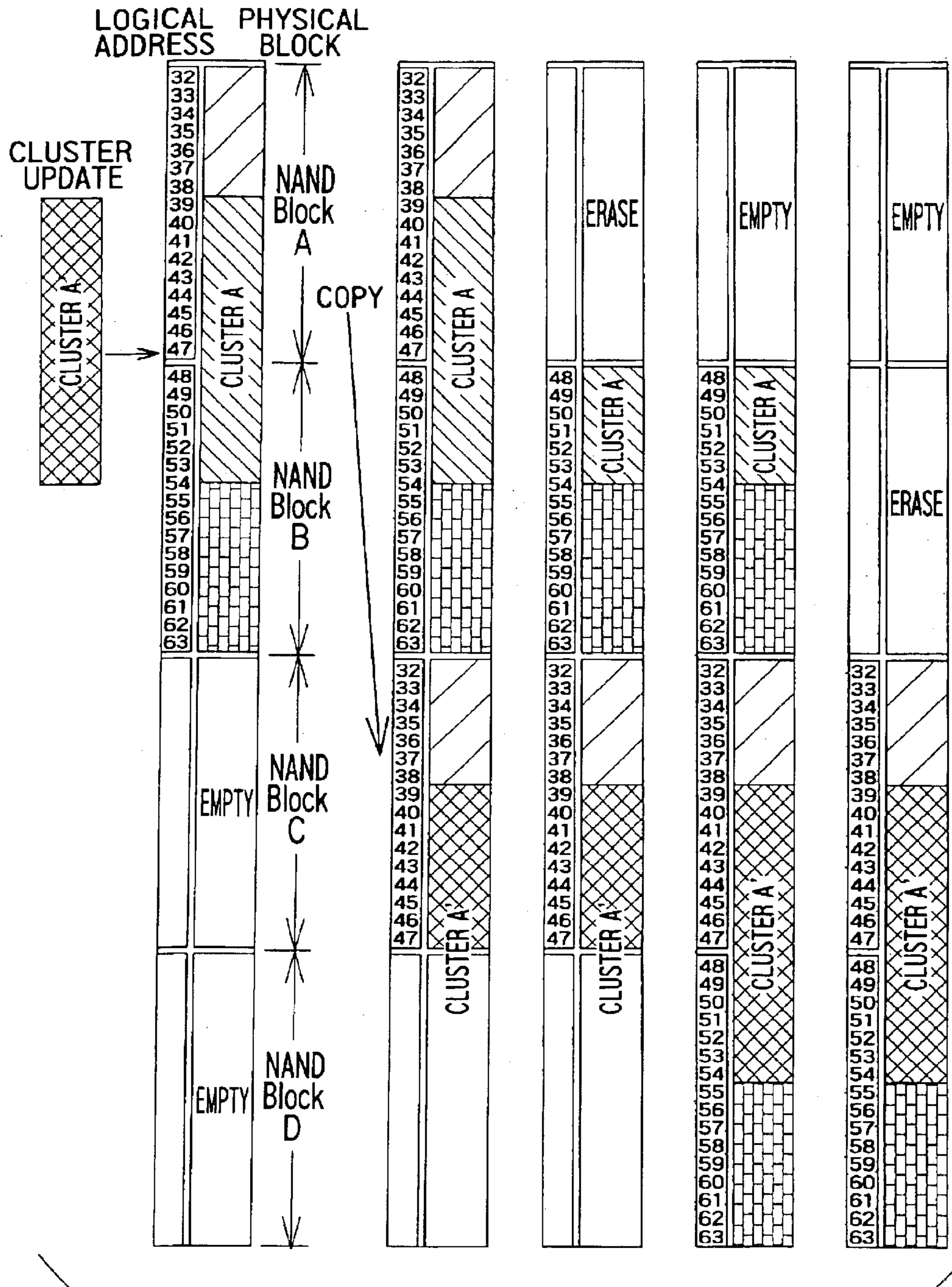
FIG. 15 PRIOR ART
