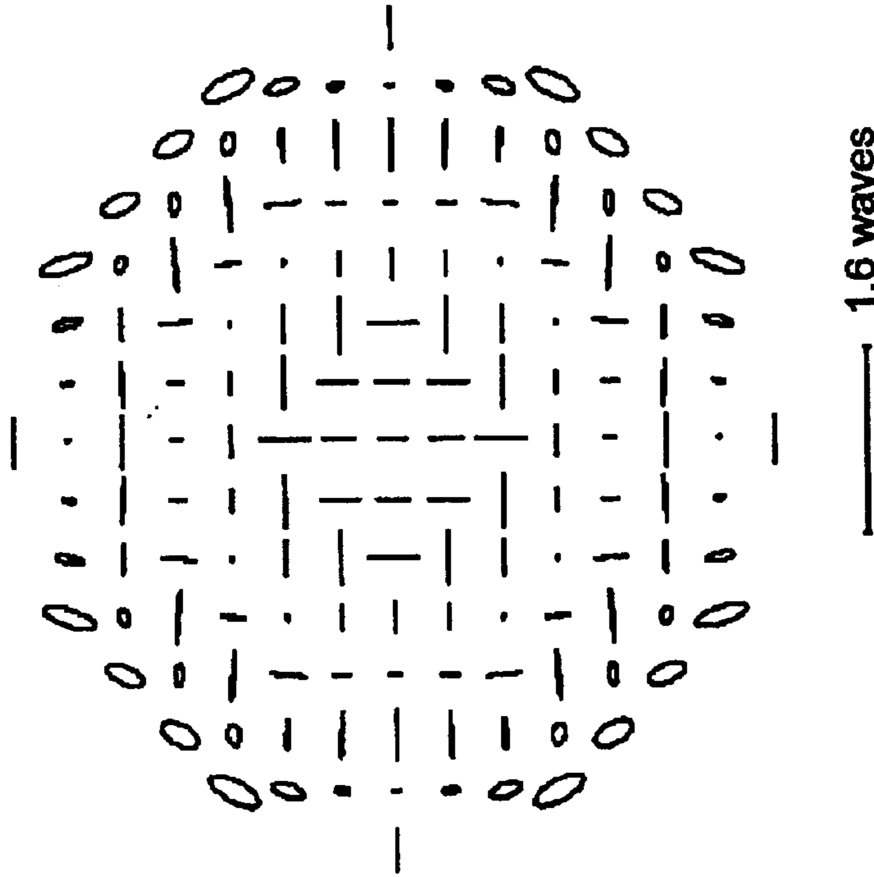
Retardance, On-Axis Field
