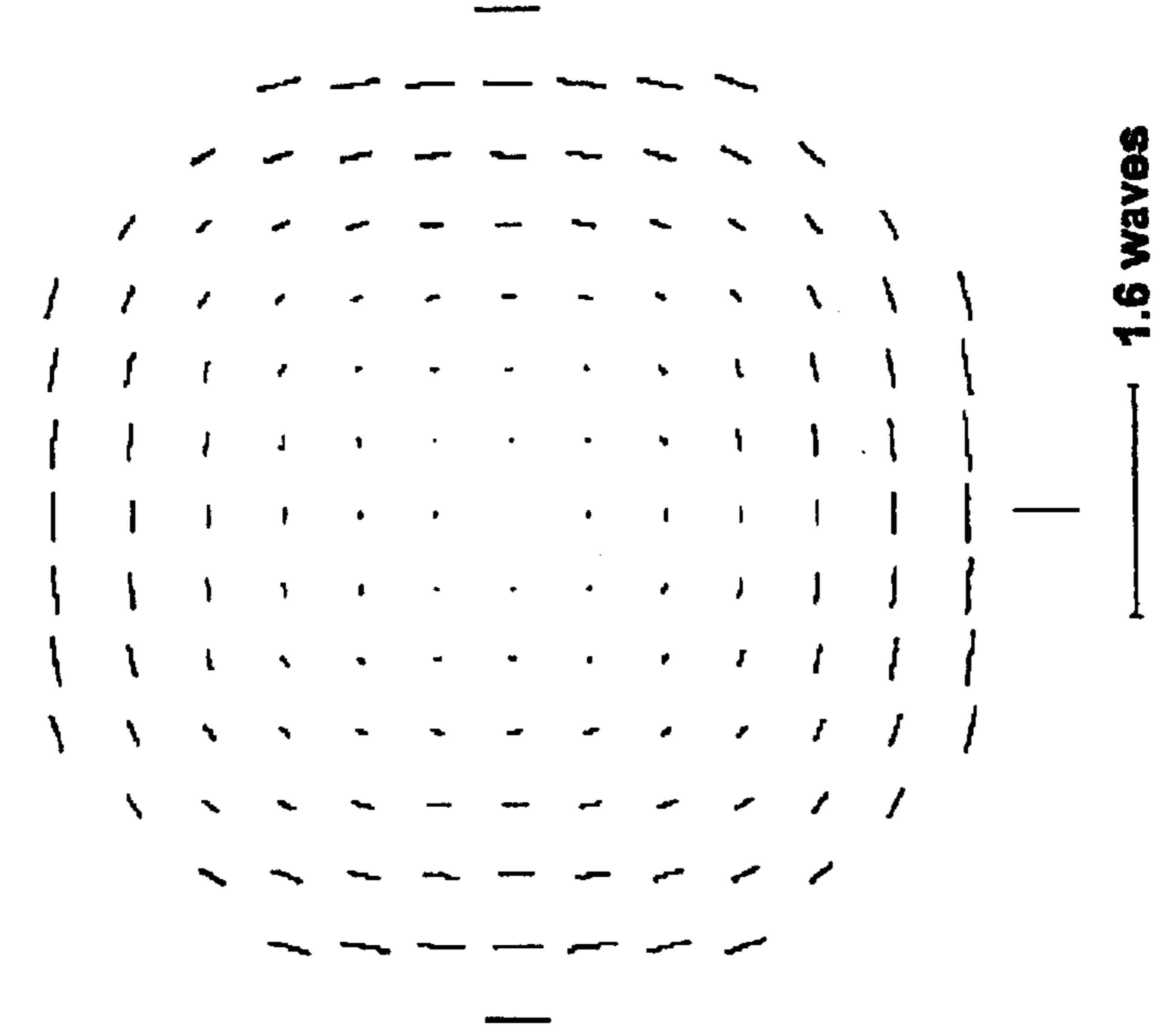
Net Retardance of Elements Following Rotators, Extreme Field
