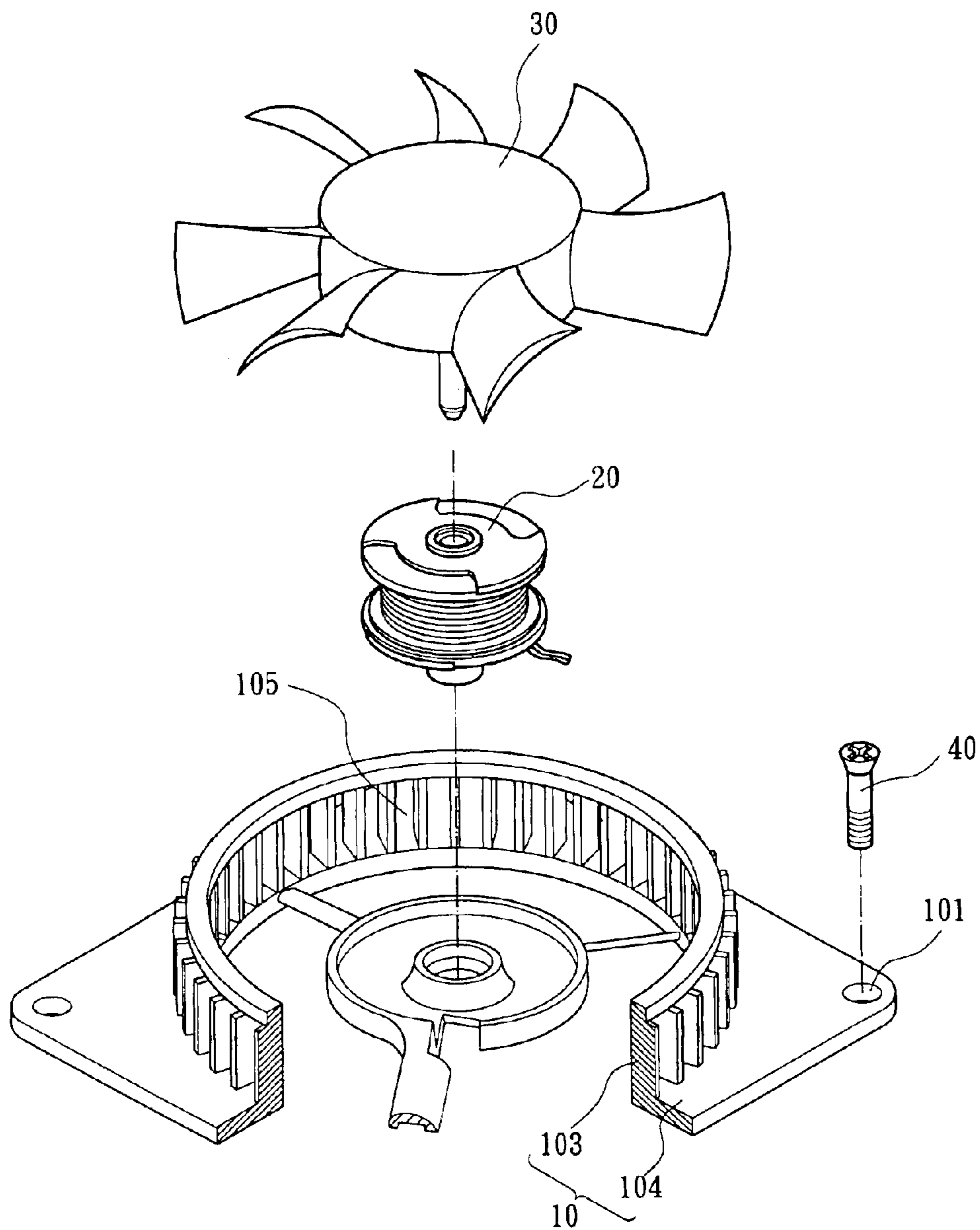
FIG. 2 PRIOR ART
