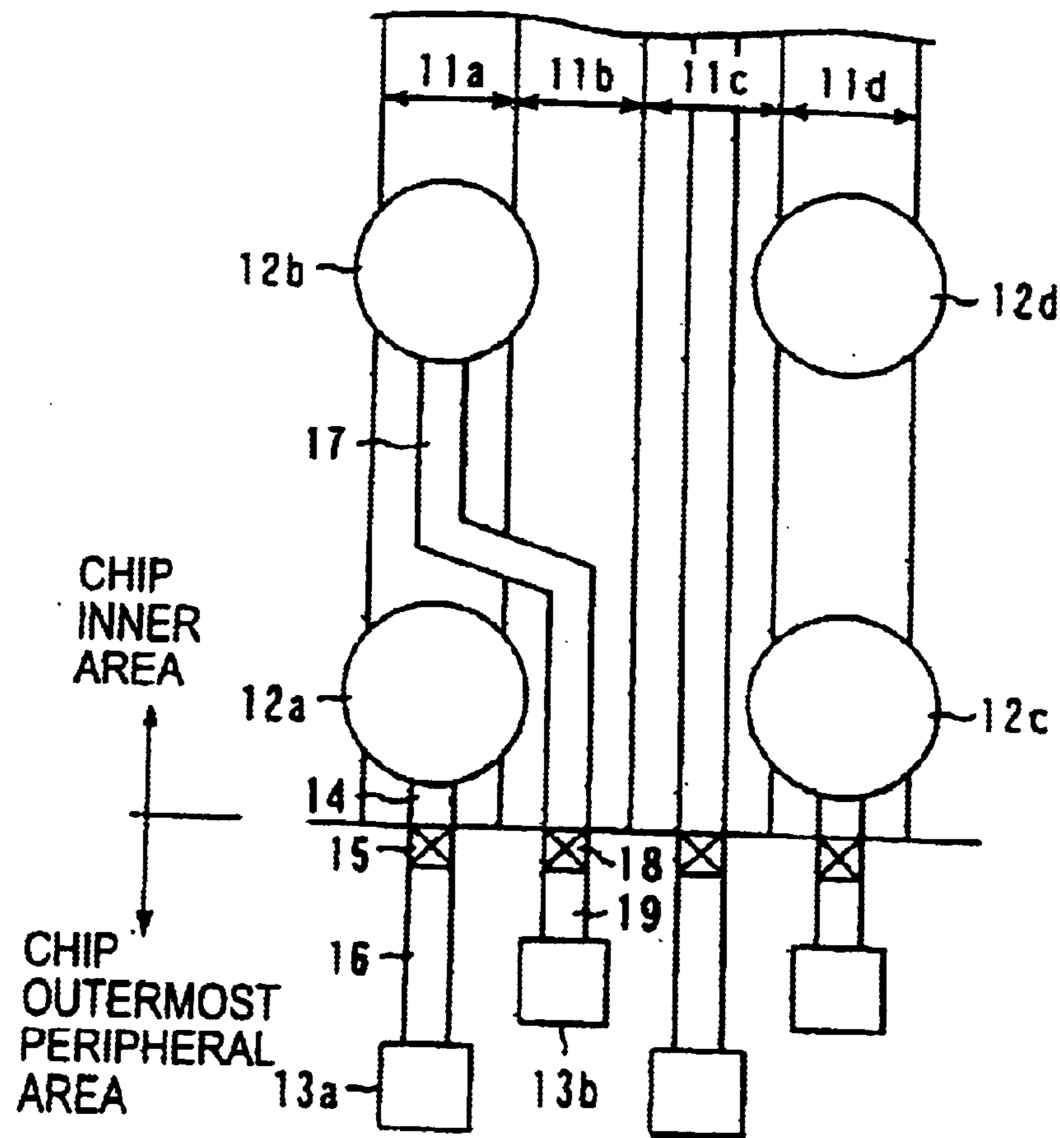
FIG. 4 PRIOR ART
