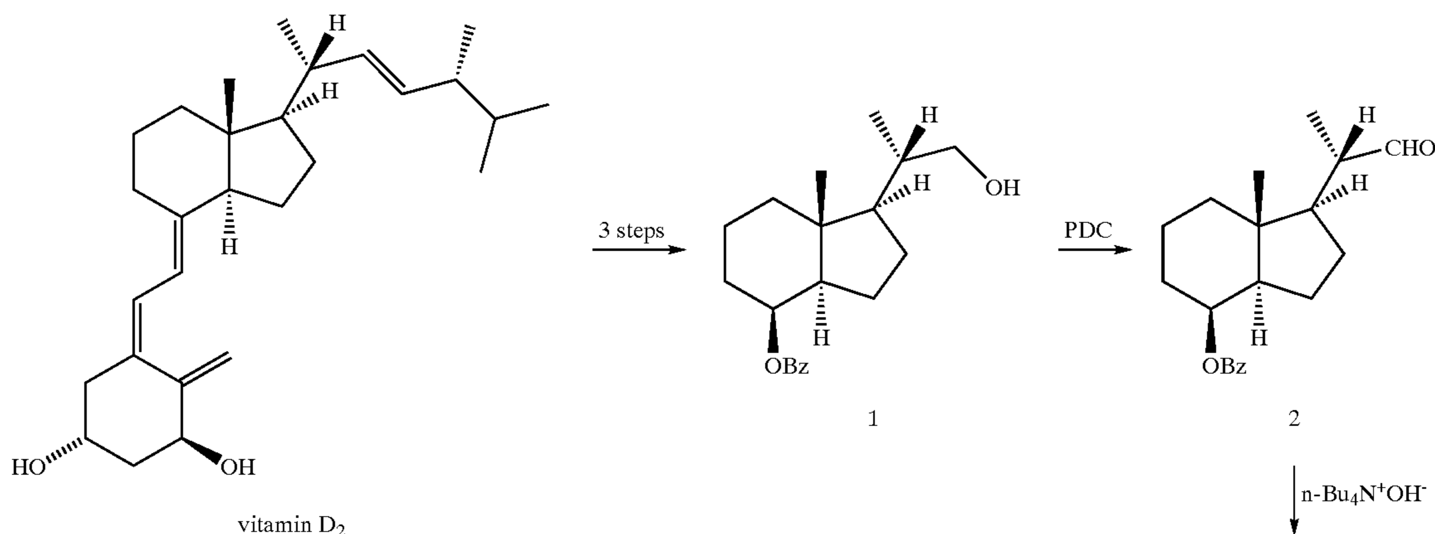
Scheme 1
