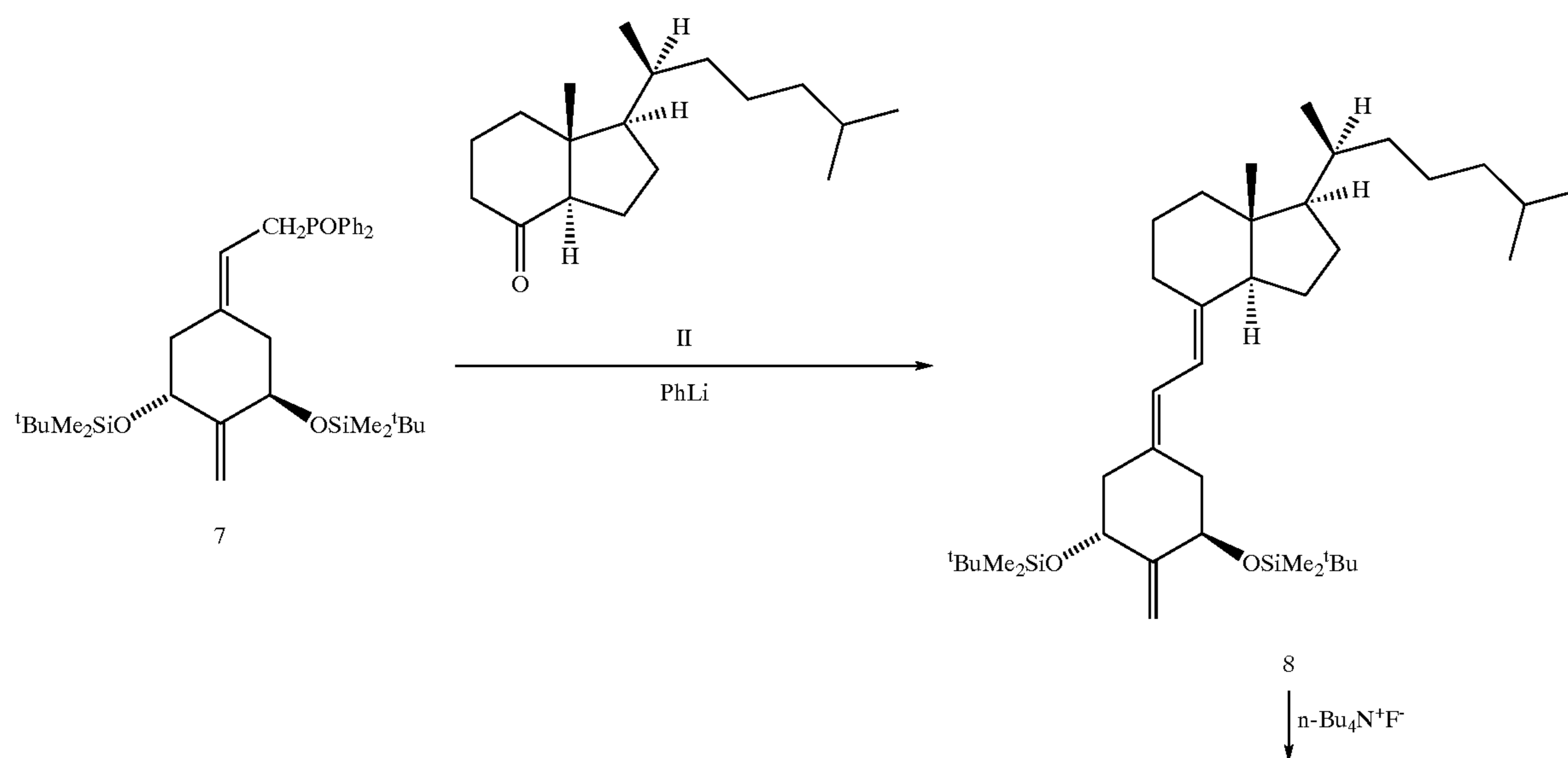
Scheme 2
