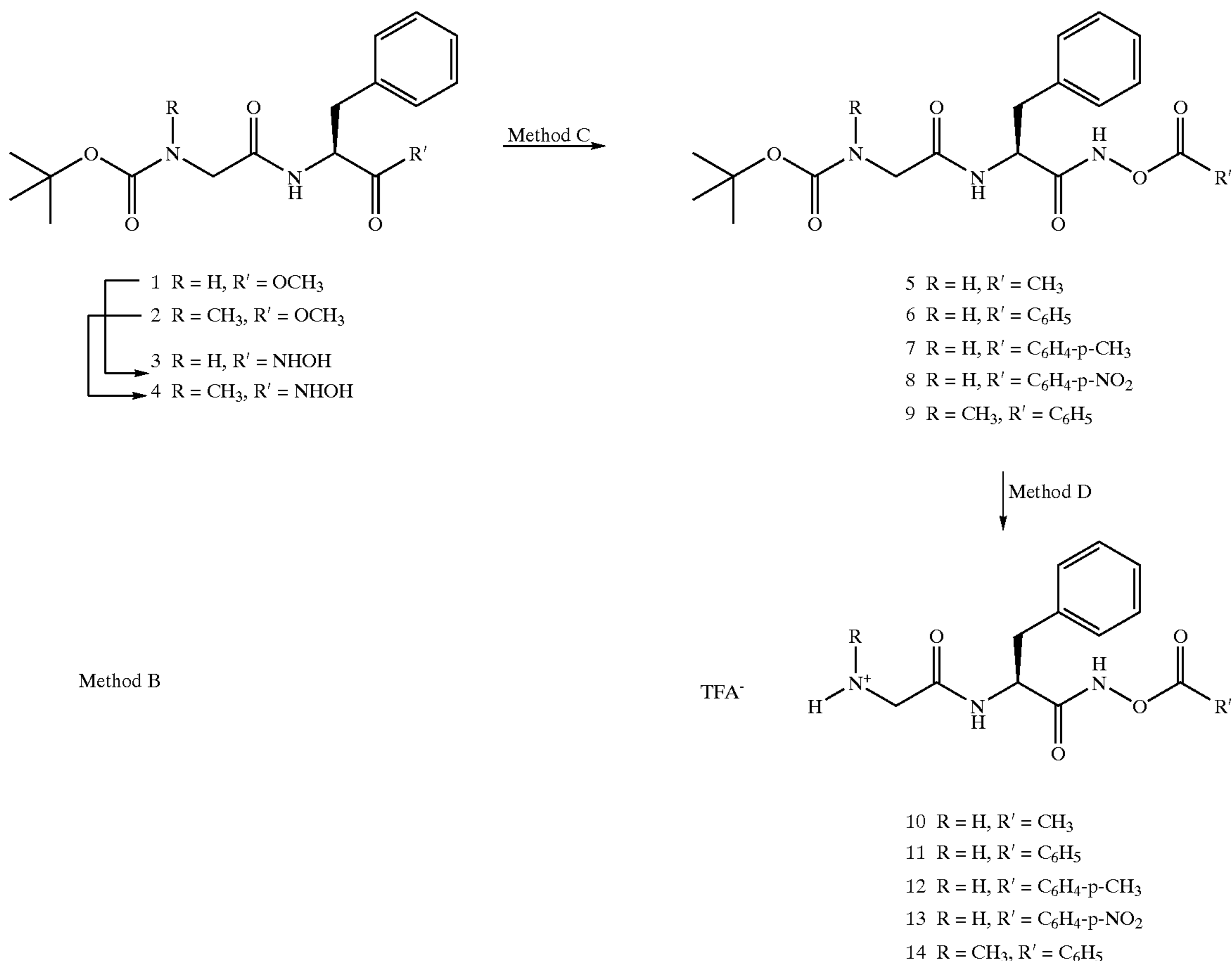
Scheme 1. Synthesis of the compounds 1–14
