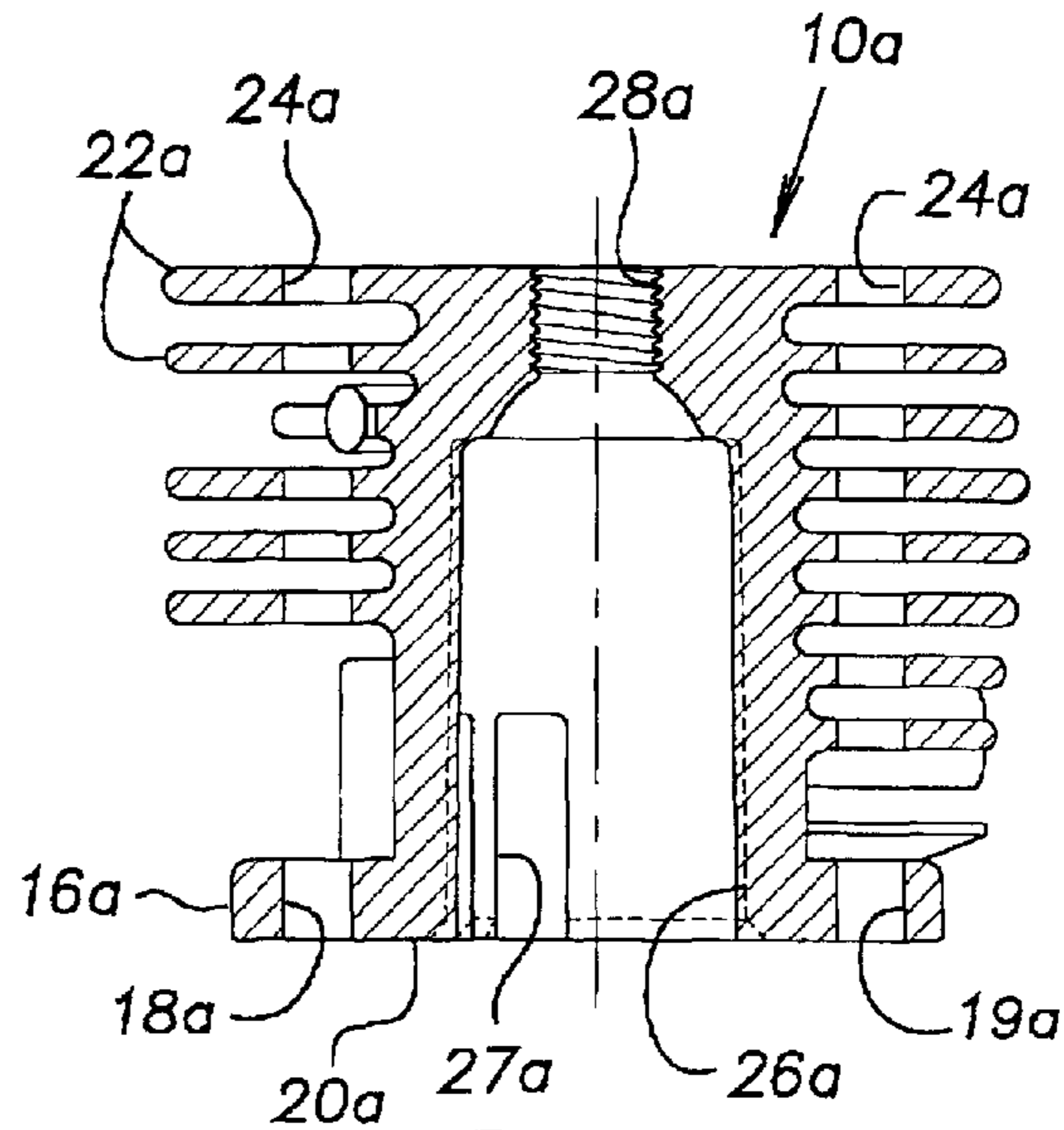
FIG. 7 PRIOR ART
