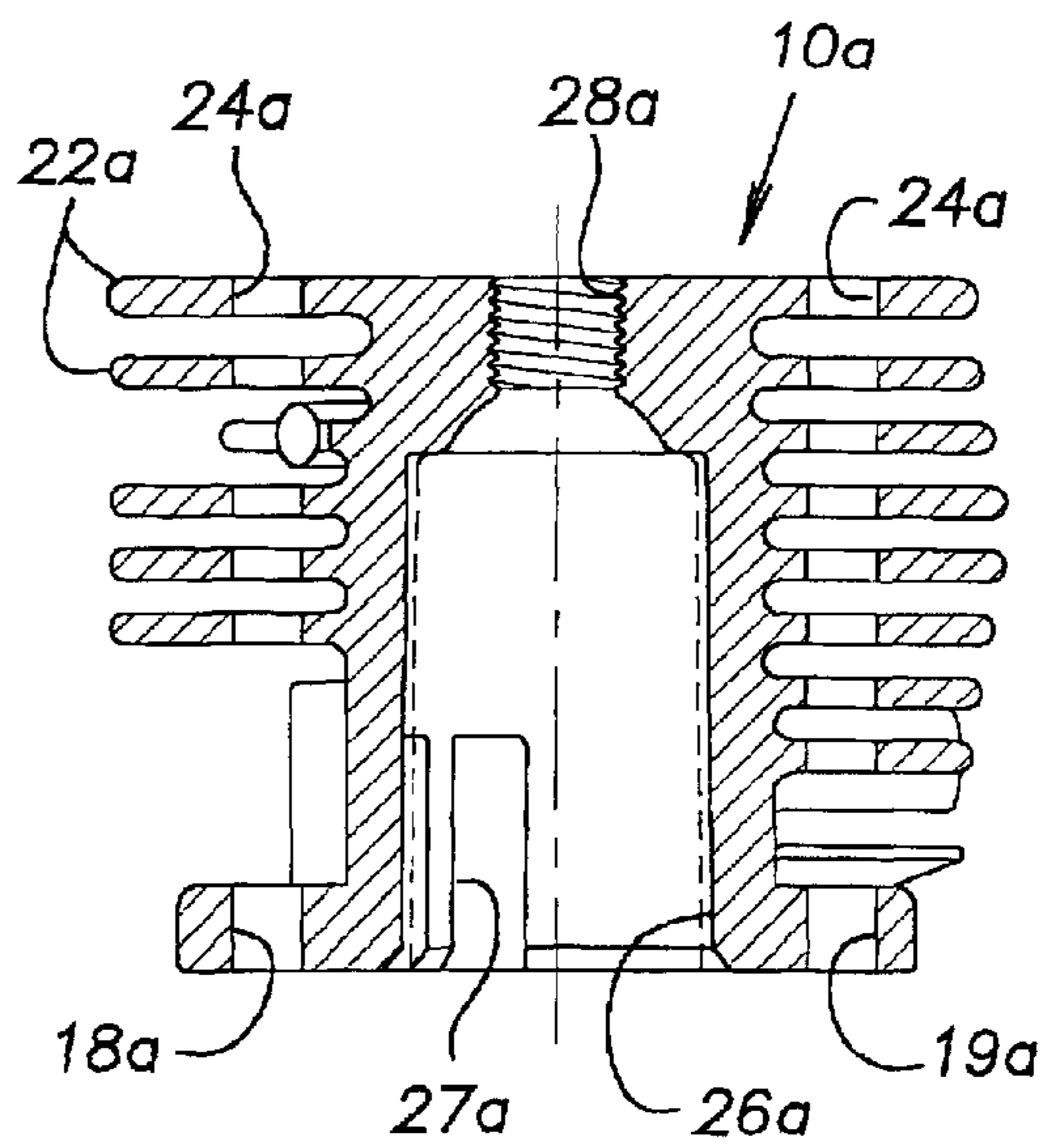
FIG. 9 PRIOR ART
