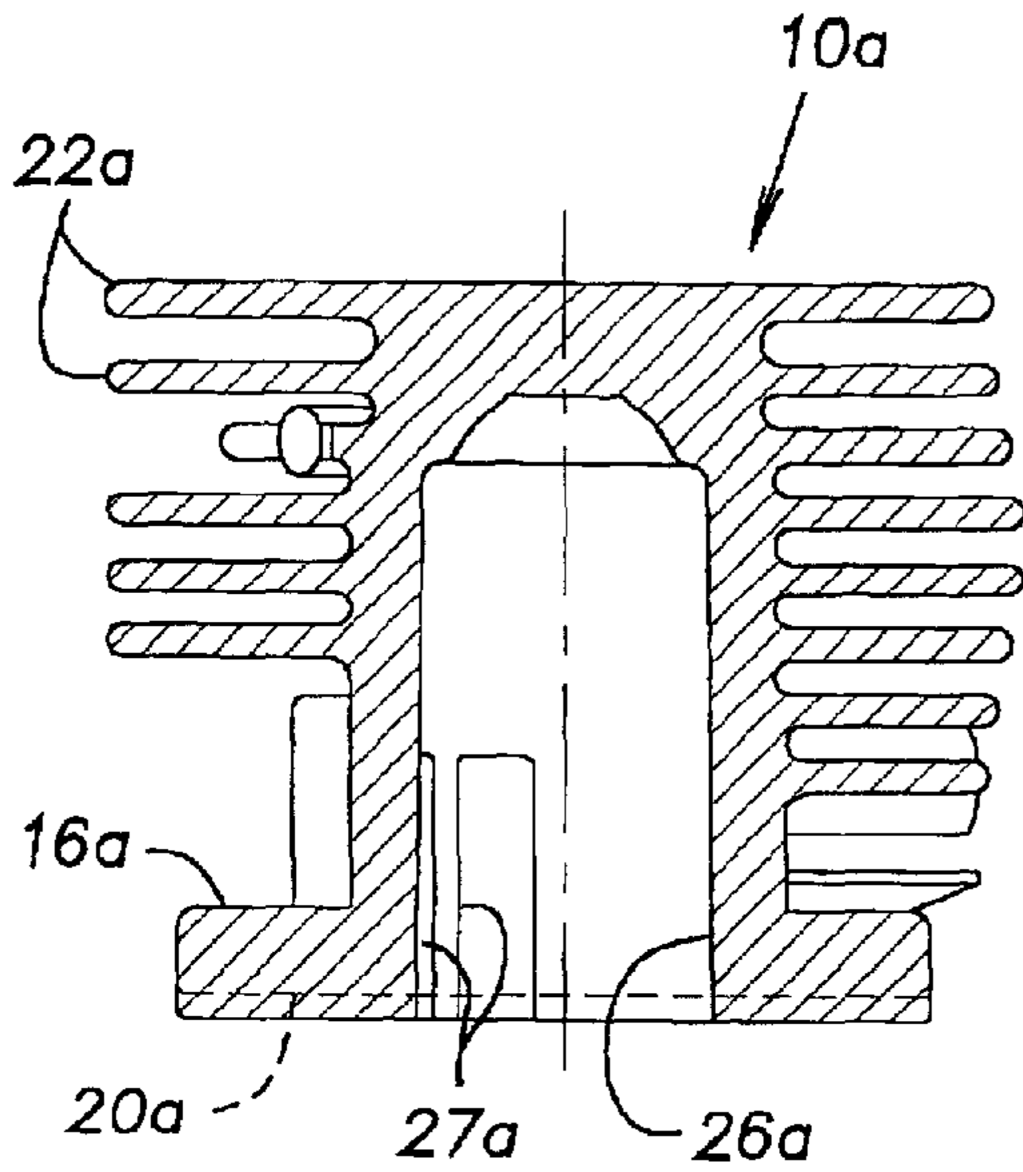
FIG. 6 PRIOR ART
