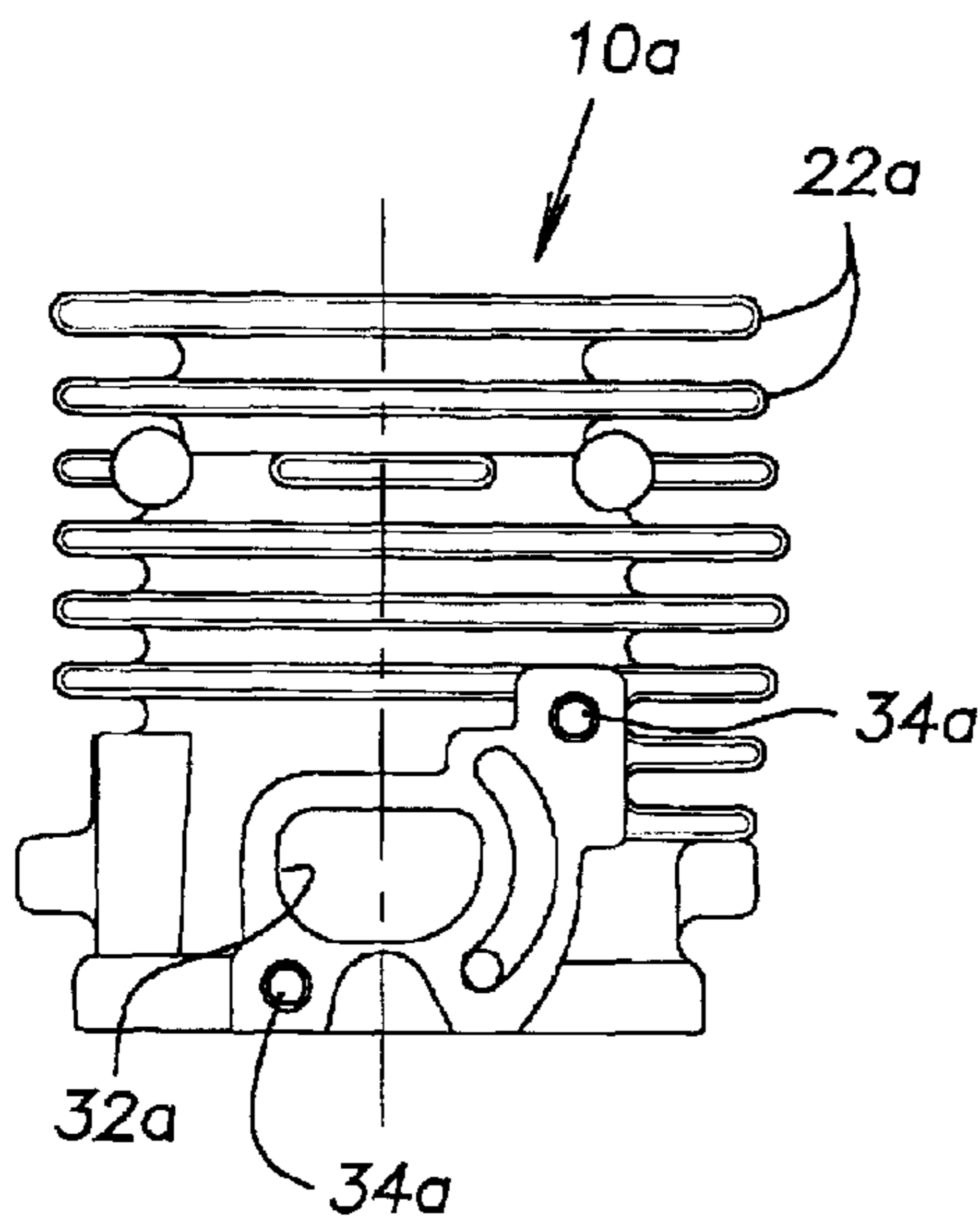
FIG. 8 PRIOR ART
