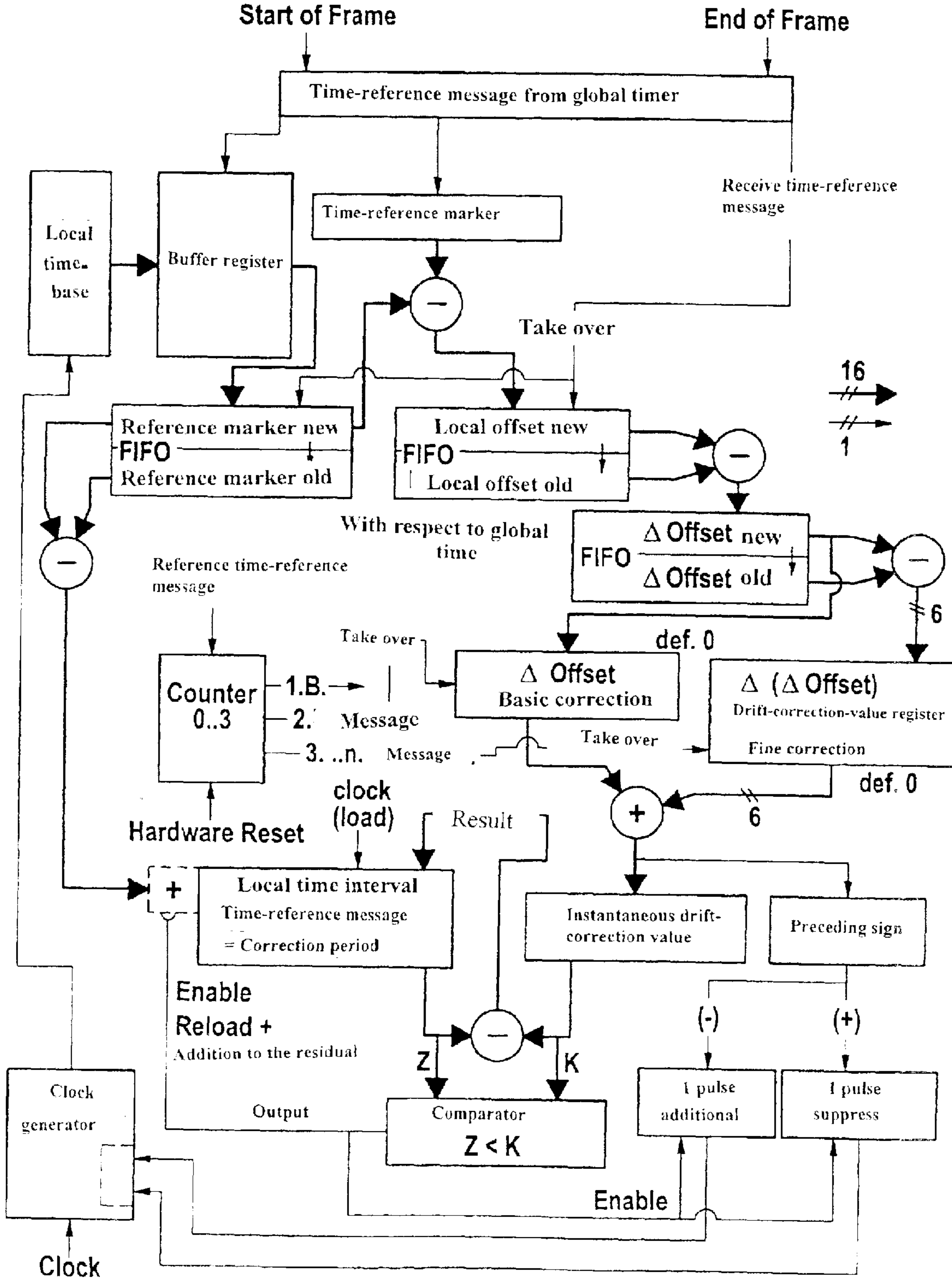
Drift correction (Block diagram)
