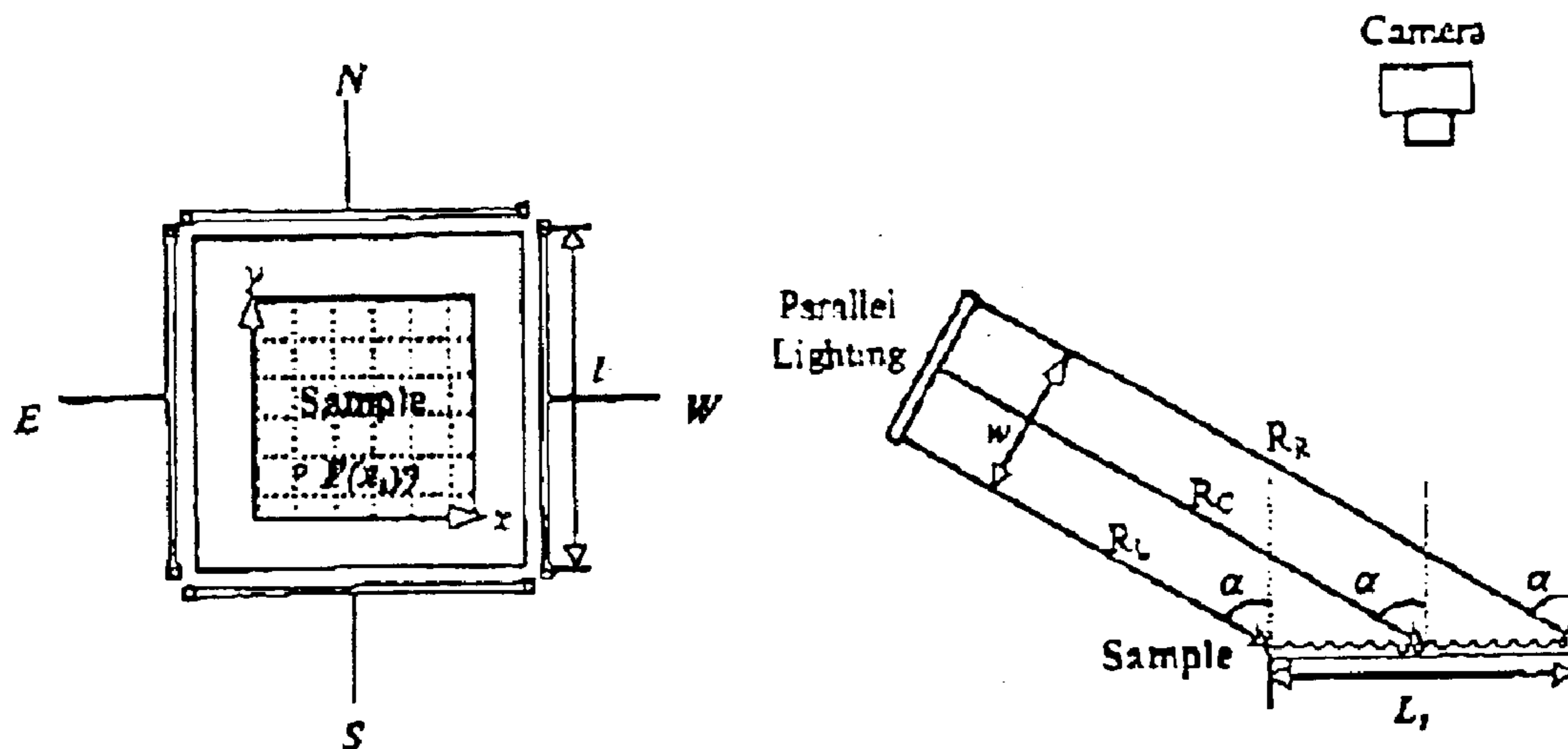
Figure 2 Lighting System
