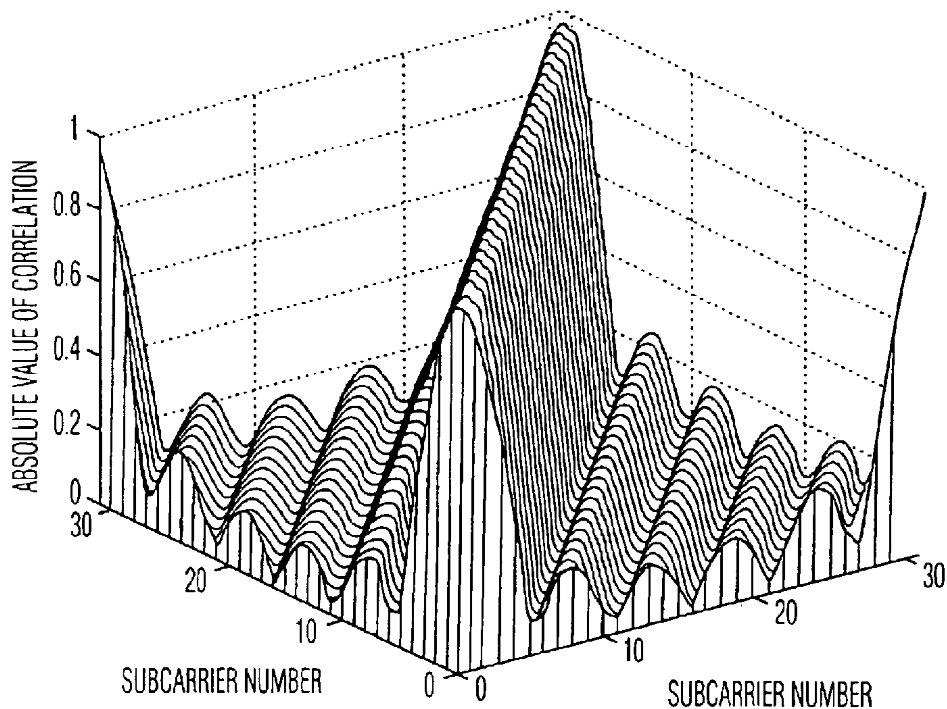
FIG. 7 (PRIOR ART)
