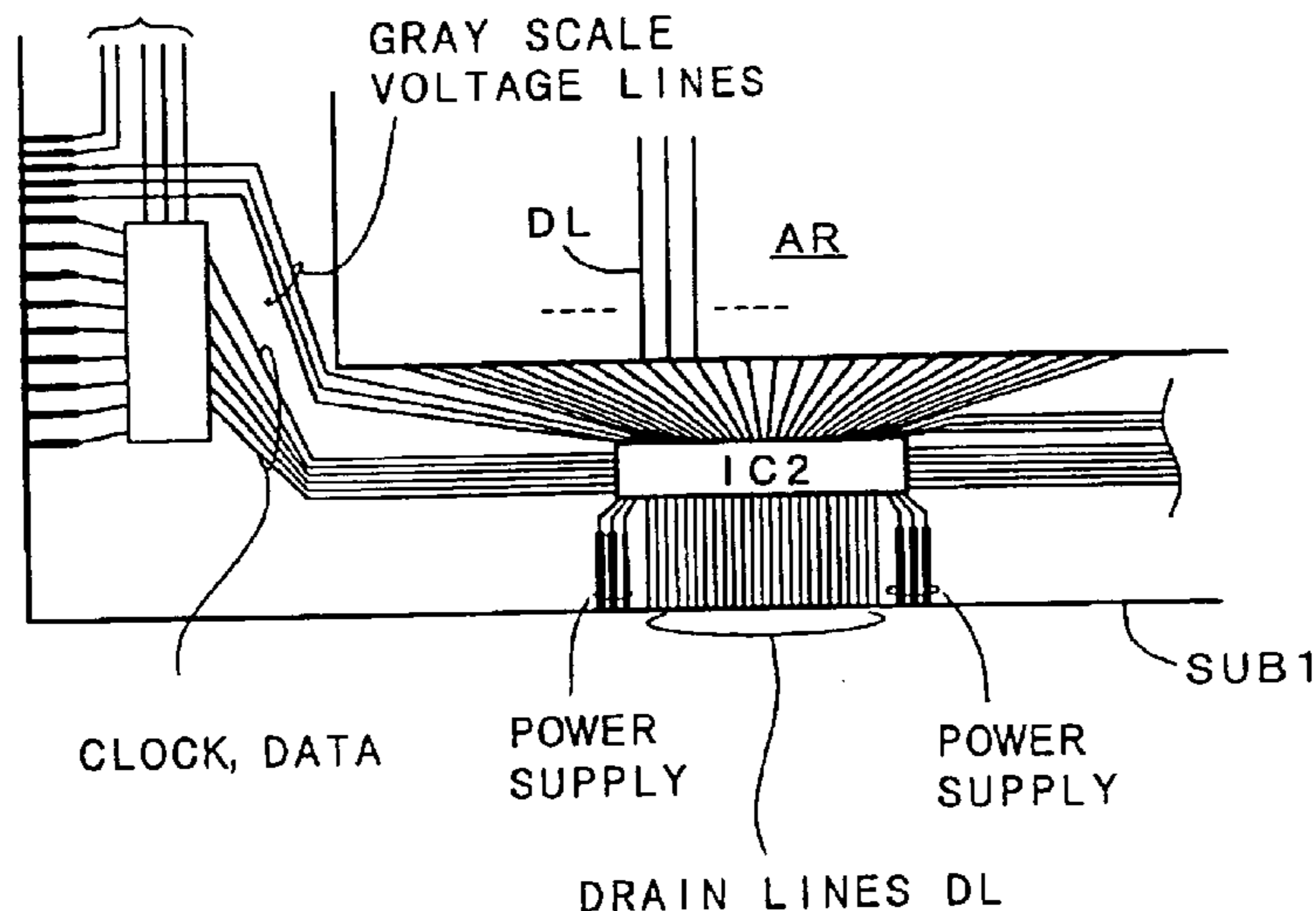
POWER SUPPLY LINES AND SIGNAL LINES FOR GATE ELECTRODES
